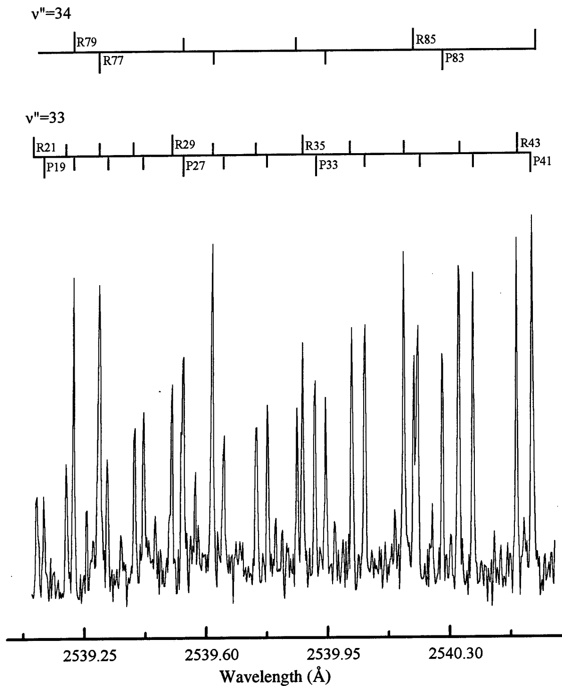
Figure 7.4: High Resolution LIF of I_2 ( D, v'=33, 34 \leftarrow X, v''=23 ) with Ar (400 ns delay, 150 mTorr)
