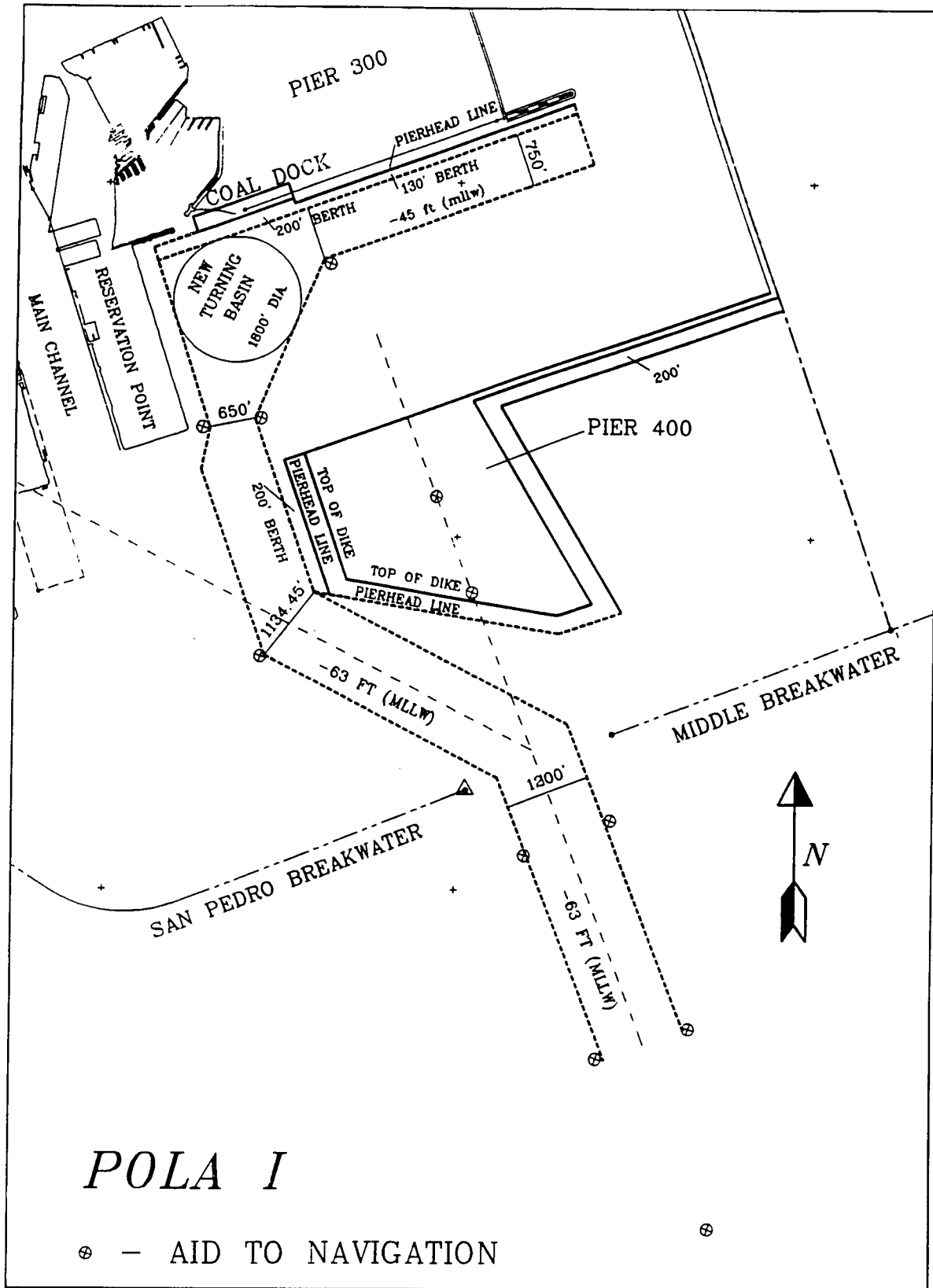
Figure 2. POLA I - Proposed channel
