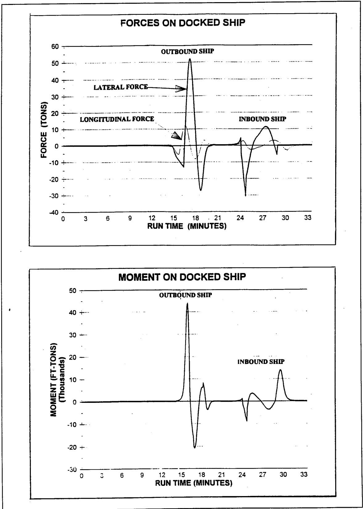
Figure 9. Passing ship effects
