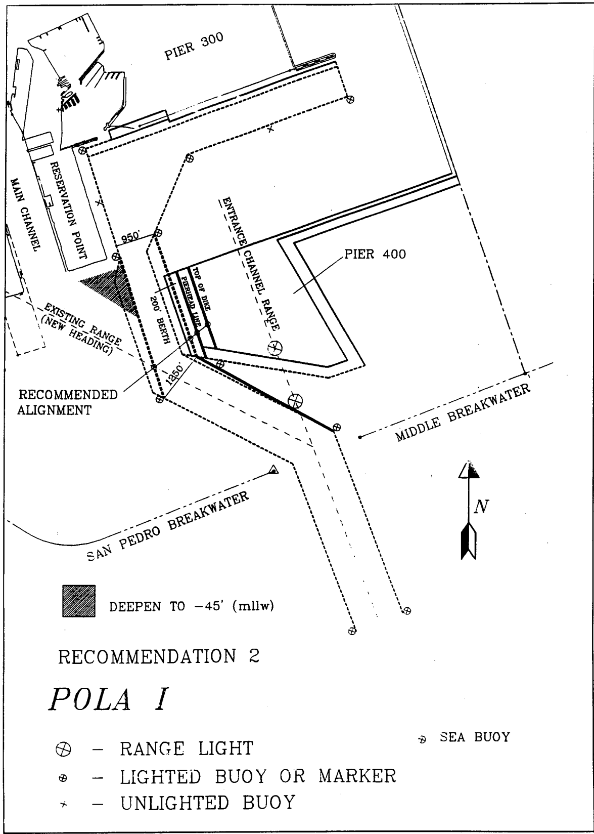
Figure 11. POLA I Recommendation 2
