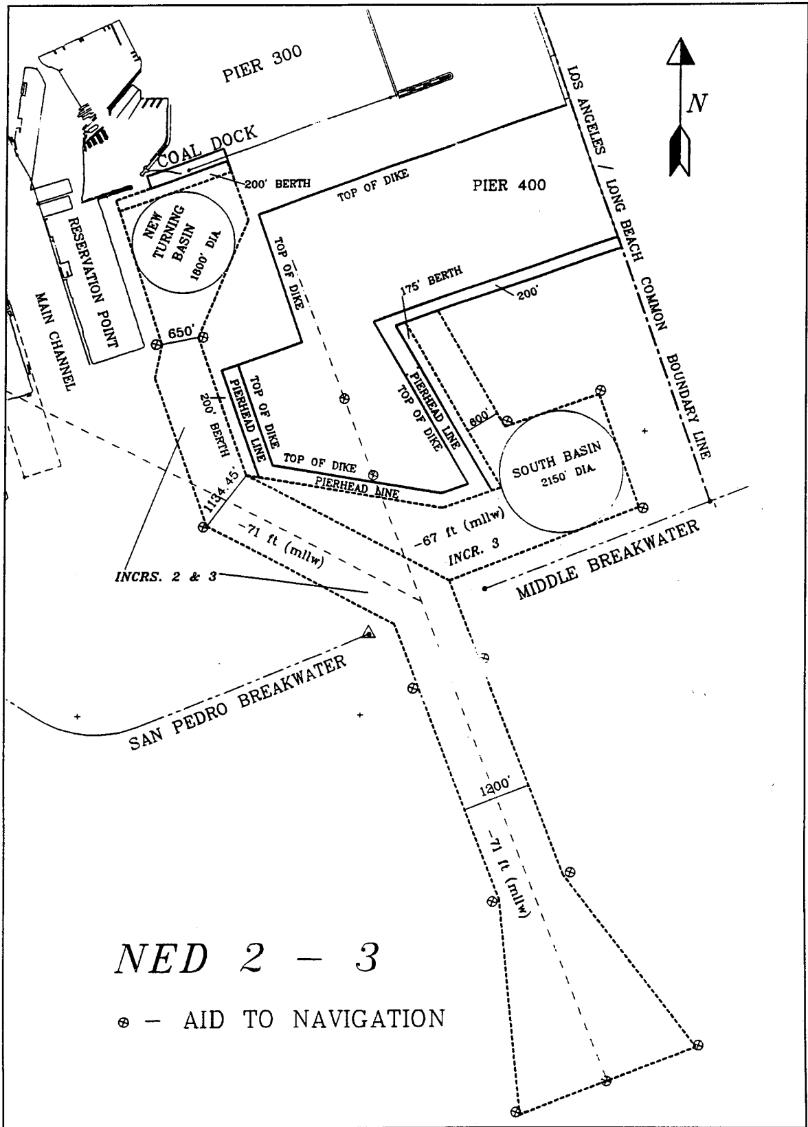
Figure 5. NED 2-3 - Proposed channel
