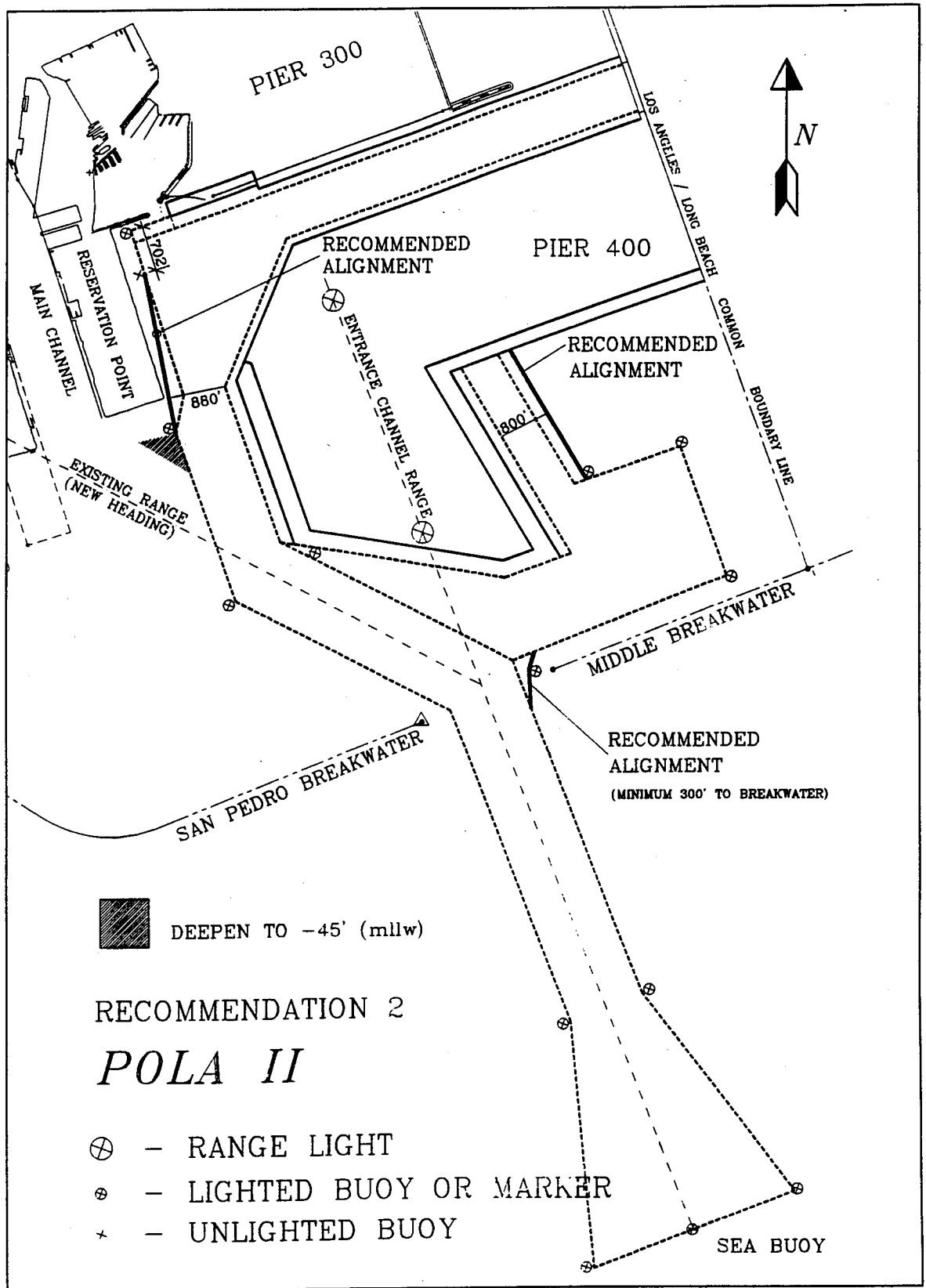
Figure 14. POLA II Recommendation 2
