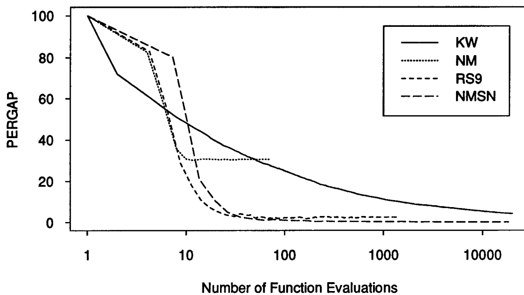
Function 10, Gap/Sigma = 10
