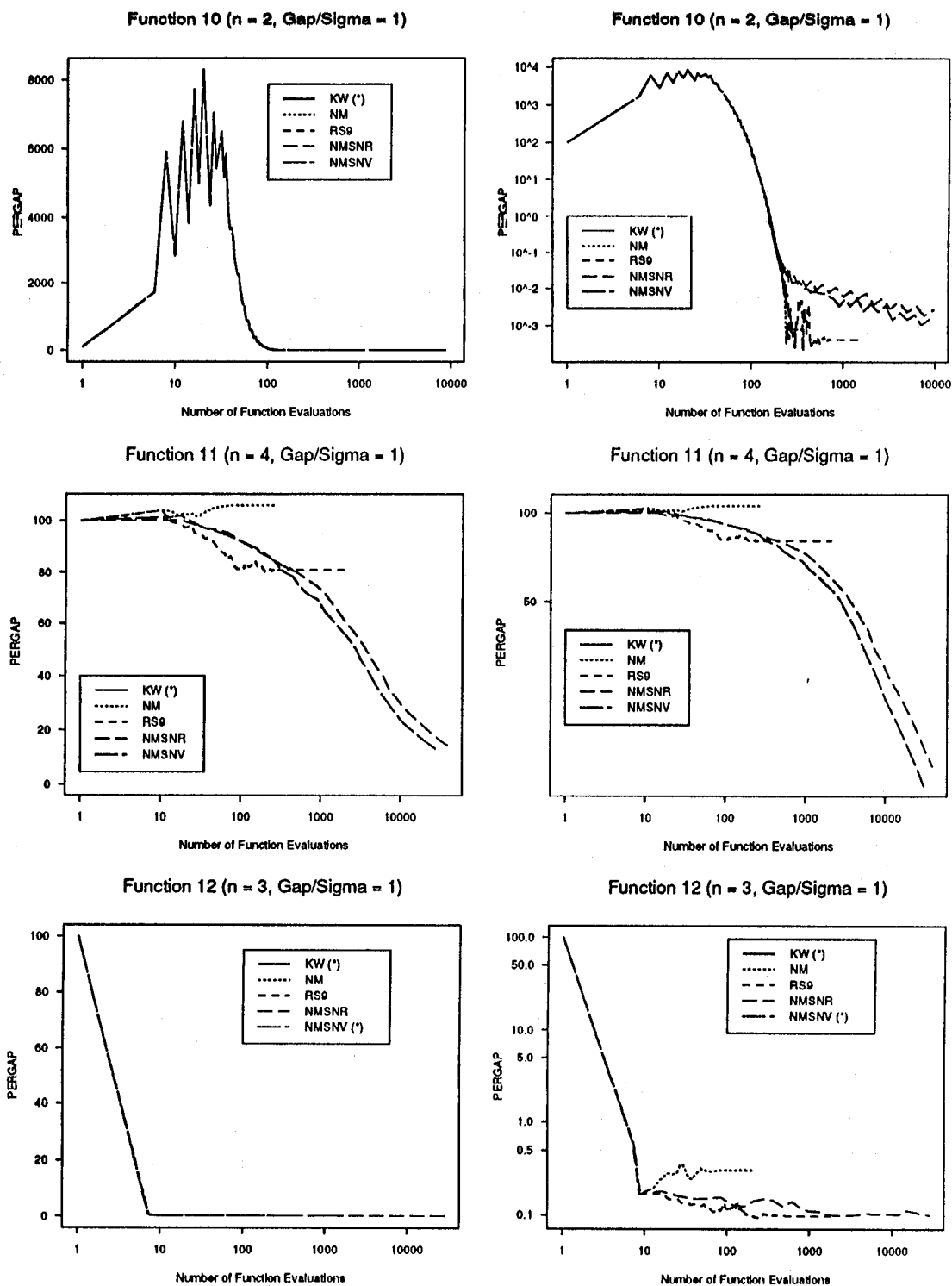
Figure C.4: Test Results for Multivariate Functions 10-12, GAP/\sigma \approx 1
