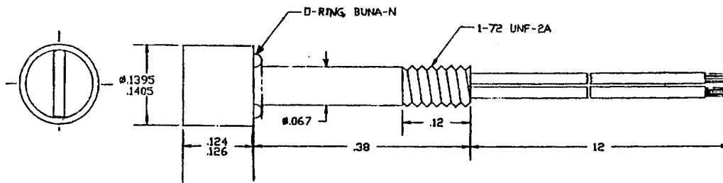
Fig. 3.2 Model PTF 100-20404 Heat Flux Gauge (Medtherm Corp., 1994)
