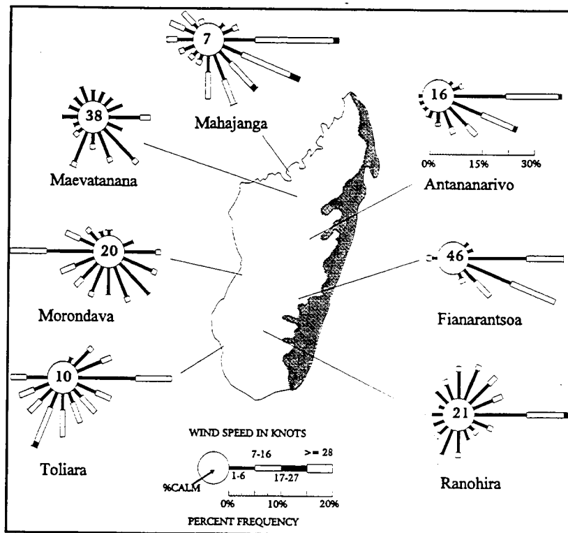
Figure 7-14. July Surface Wind Roses.
