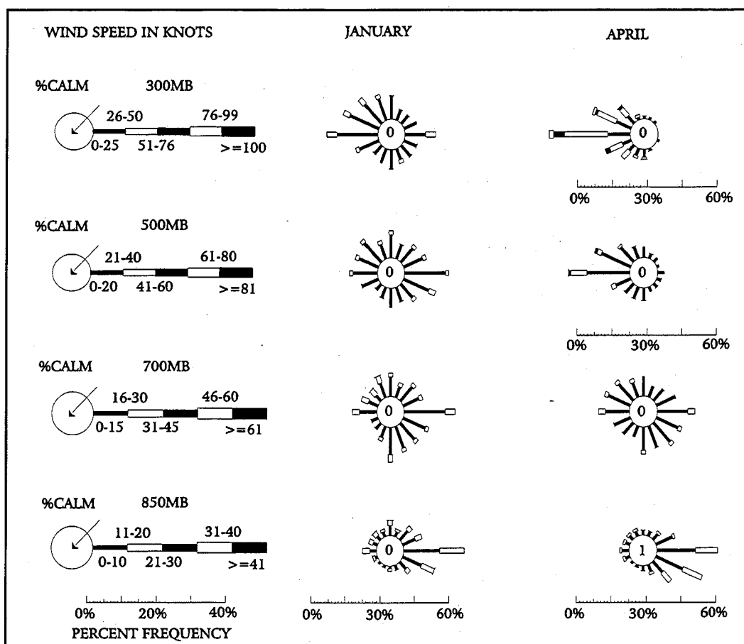
Figure 7-7. January and April Upper-Air Wind Roses at Antananarivo.
