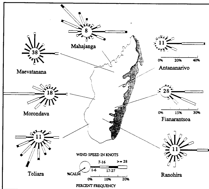
Figure 7-15. October Surface Wind Roses.
