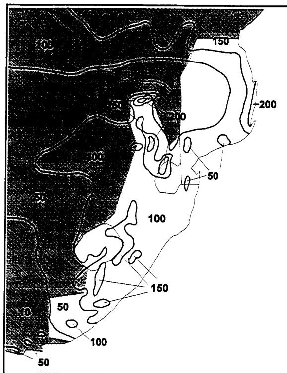
Figure 6-7. January Mean Precipitation.
