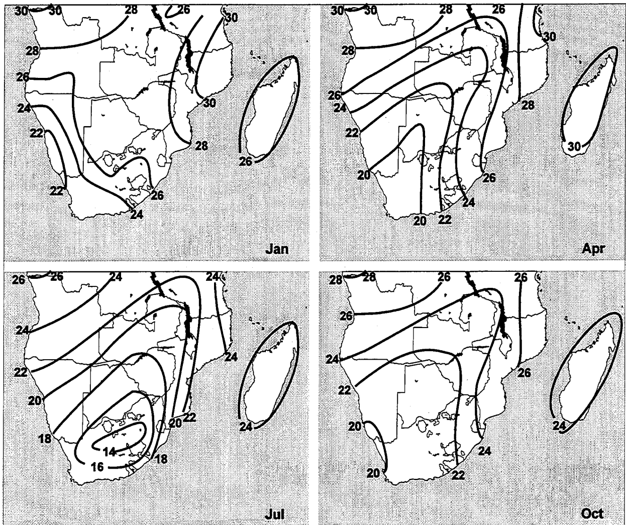
Figure 2-36. Average Daily High WBGT ( ^{\circ} C).
