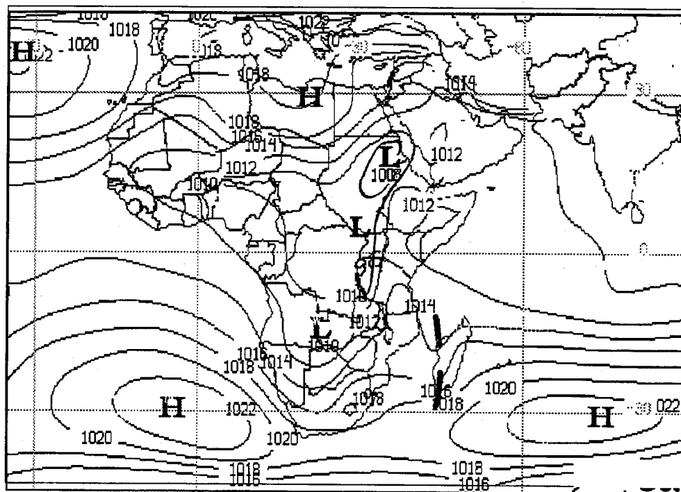
Figure 2-4b. Mean July and October Positions of Major Pressure Systems Affecting Southern Africa.
