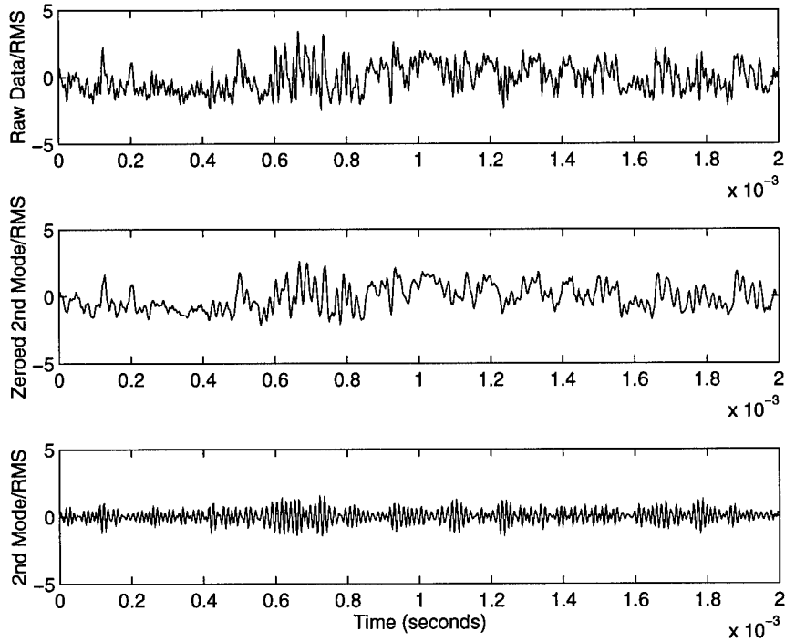
Figure A.28 : Data Signals for Station 32; Re_{\infty}=4,265,000/m
