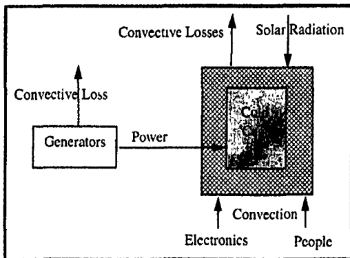
Figure 4 The HMMWV Thermal Space
