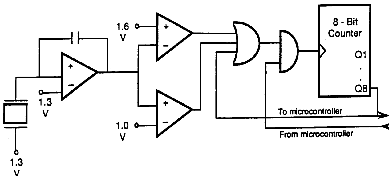
Figure 2-3. Shock Recording Circuitry
