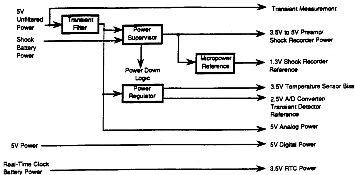
Figure 2-2. Power Regulation Electronics
