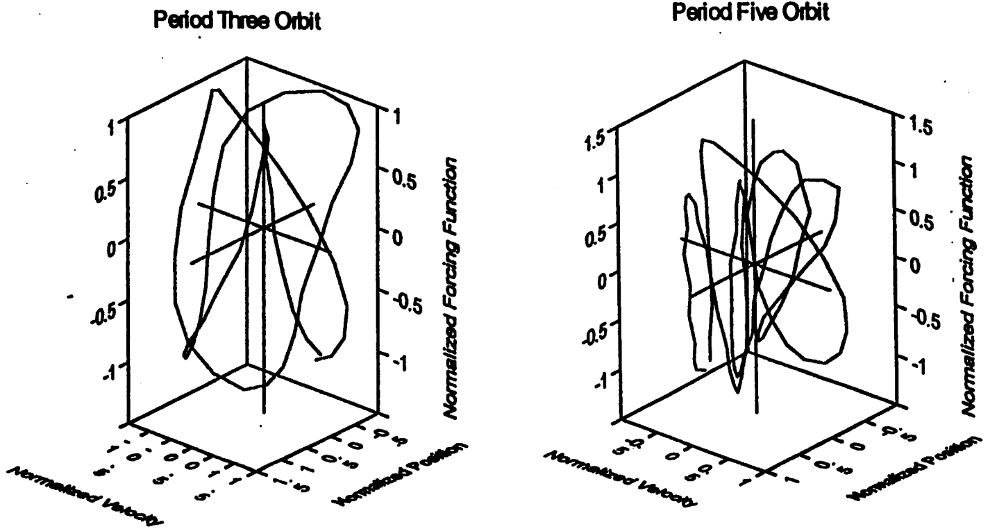
Figure 19. Experimental Period 3 and Period 5 Orbits
