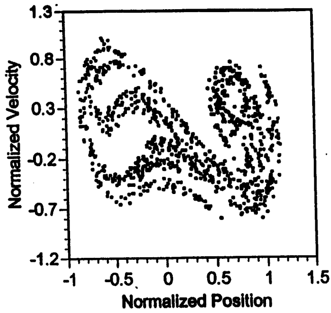
Figure 18. Experimental Poincaré Section of the Magnetoelastic Attractor
