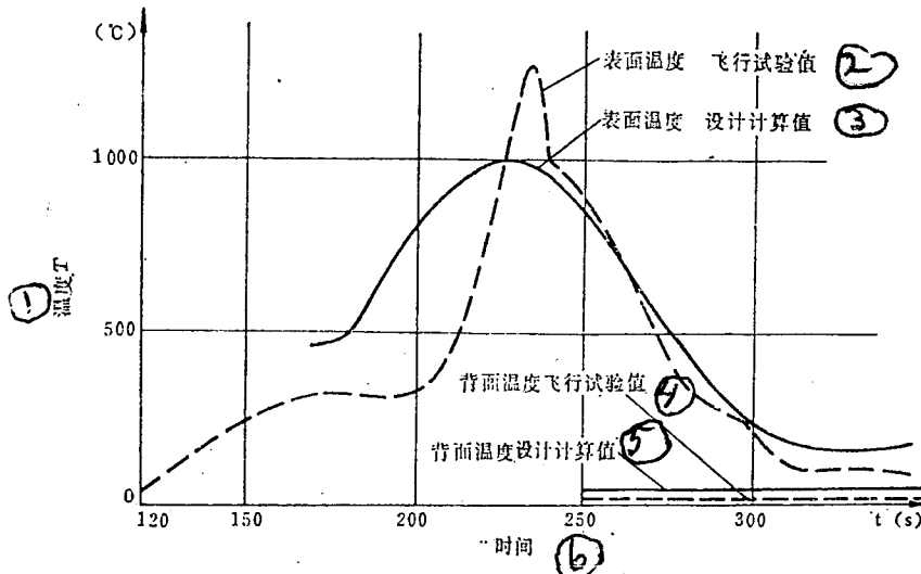
Fig. 6 Skirt Section Surface and Back Surface Temperature Curves
