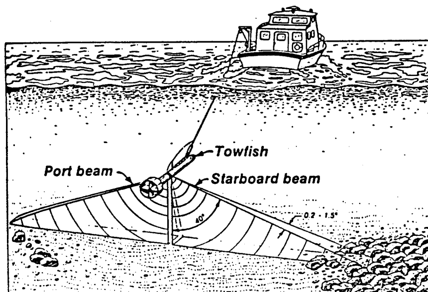
Figure 6-2. Side scan sonar in operation (Buffkin 1990).
