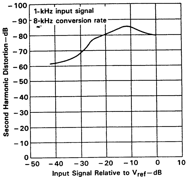
A/D SECOND HARMONIC DISTORTION vs INPUT SIGNAL
