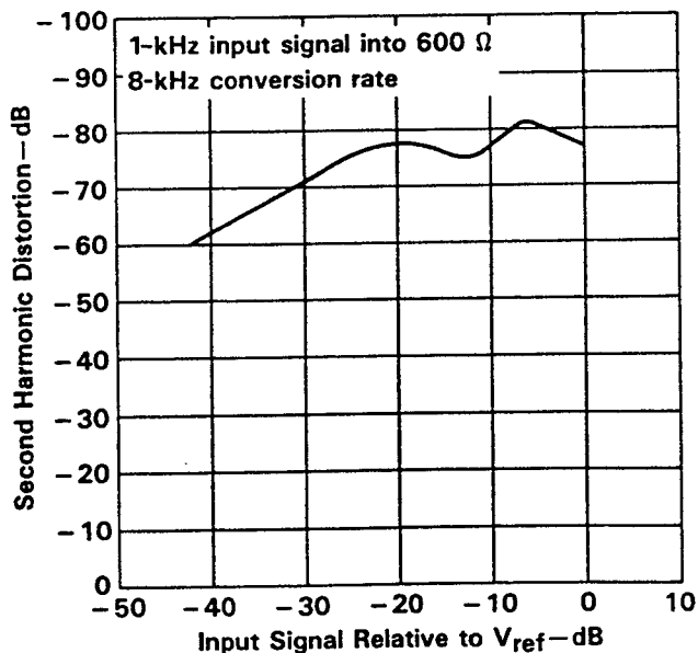
D/A SECOND HARMONIC DISTORTION vs INPUT SIGNAL
