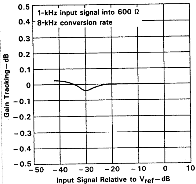
D/A GAIN TRACKING (GAIN RELATIVE TO GAIN AT 0 dB INPUT SIGNAL LEVEL)
