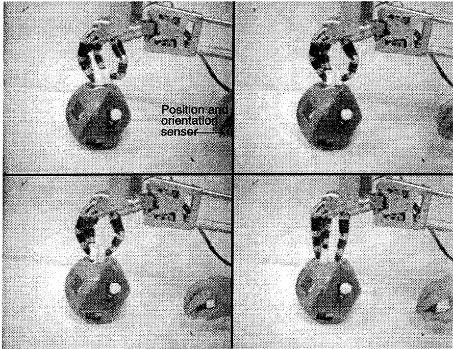
Figure 15: Telemanipulated insertion
