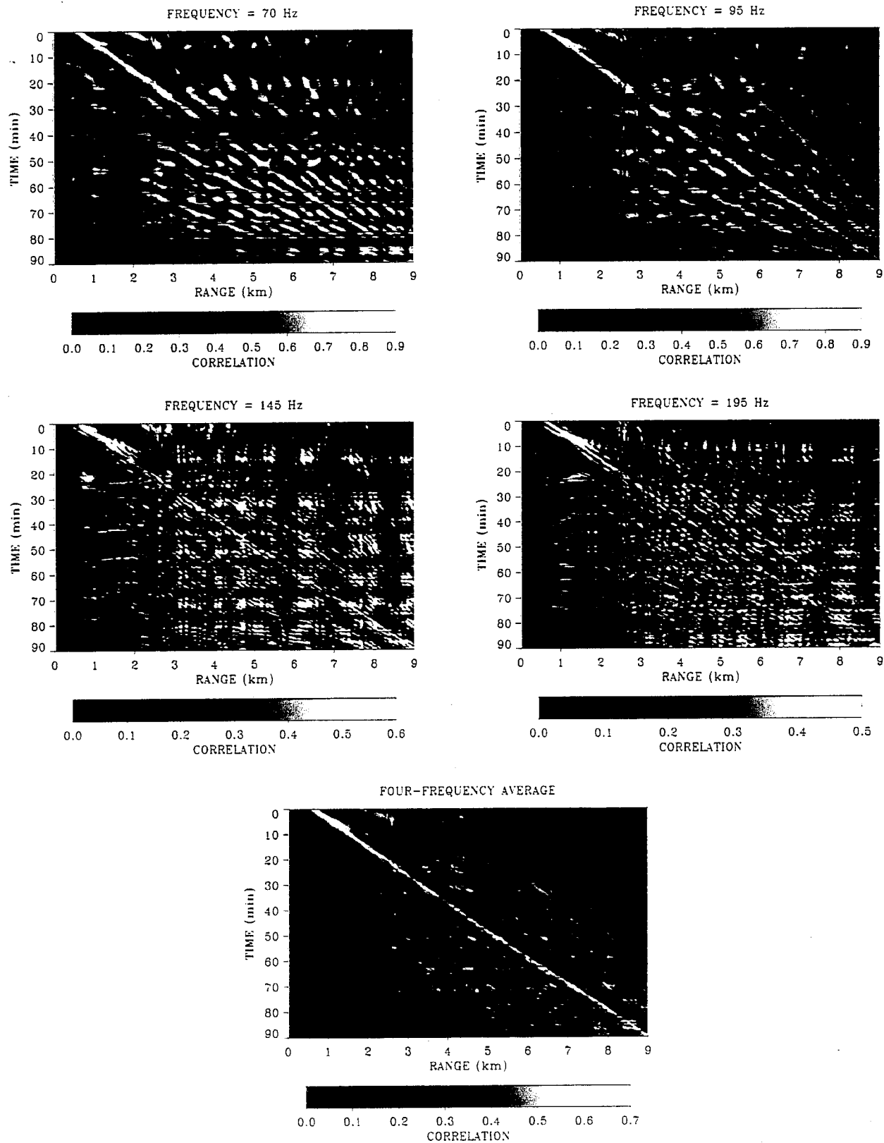
Figure 13. Track A to E, 0956 to 1126, source depth = 21 m.
