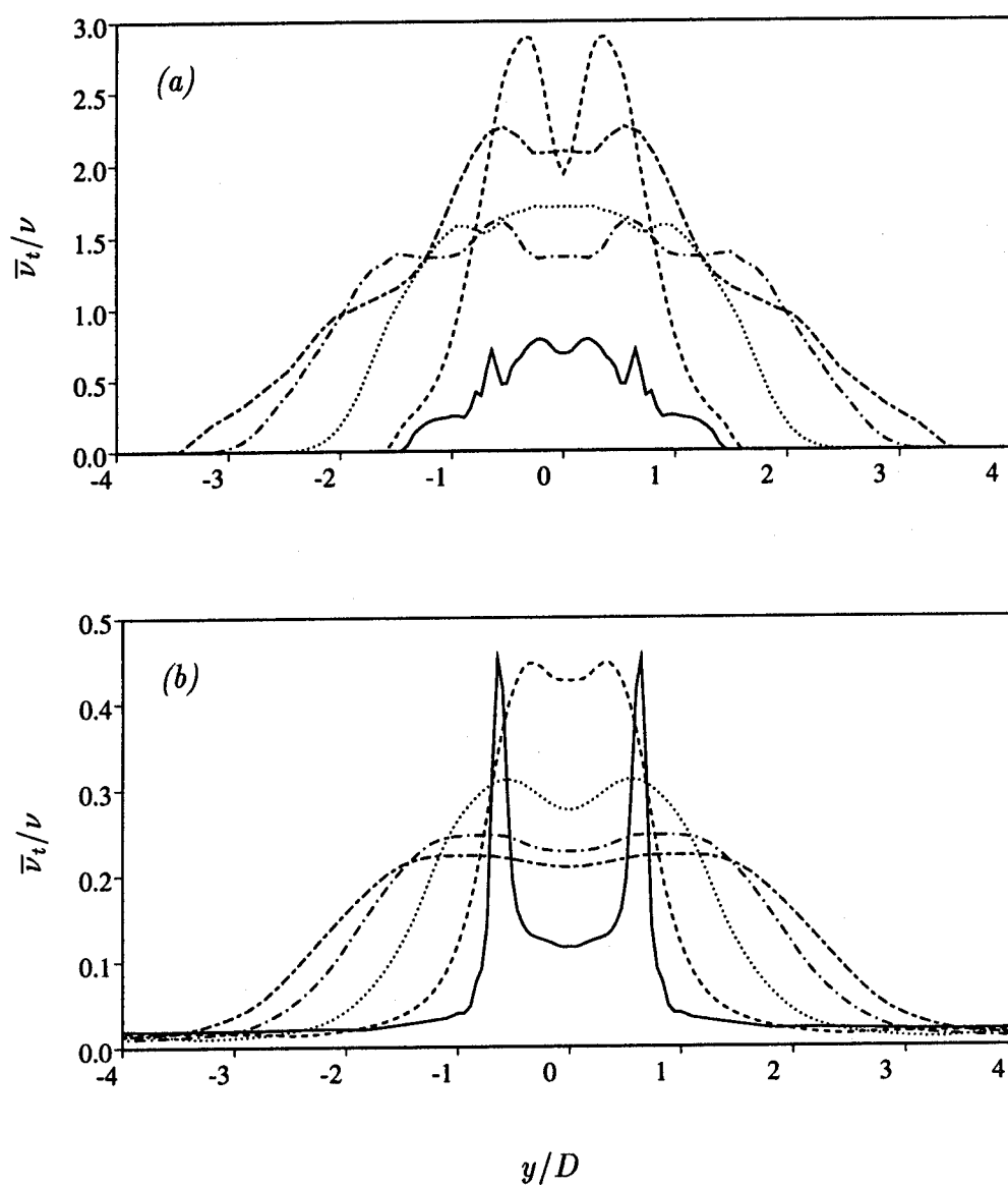
Figure 36: Re = 3,900 ; Time and spanwise-averaged eddy viscosity profiles (a): Dynamic model; (b): Fixed coefficient model — : x/D = 1 ; ---- : x/D = 2 ; ... : x/D = 4 -.- : x/D = 7 ; --- : x/D = 10
