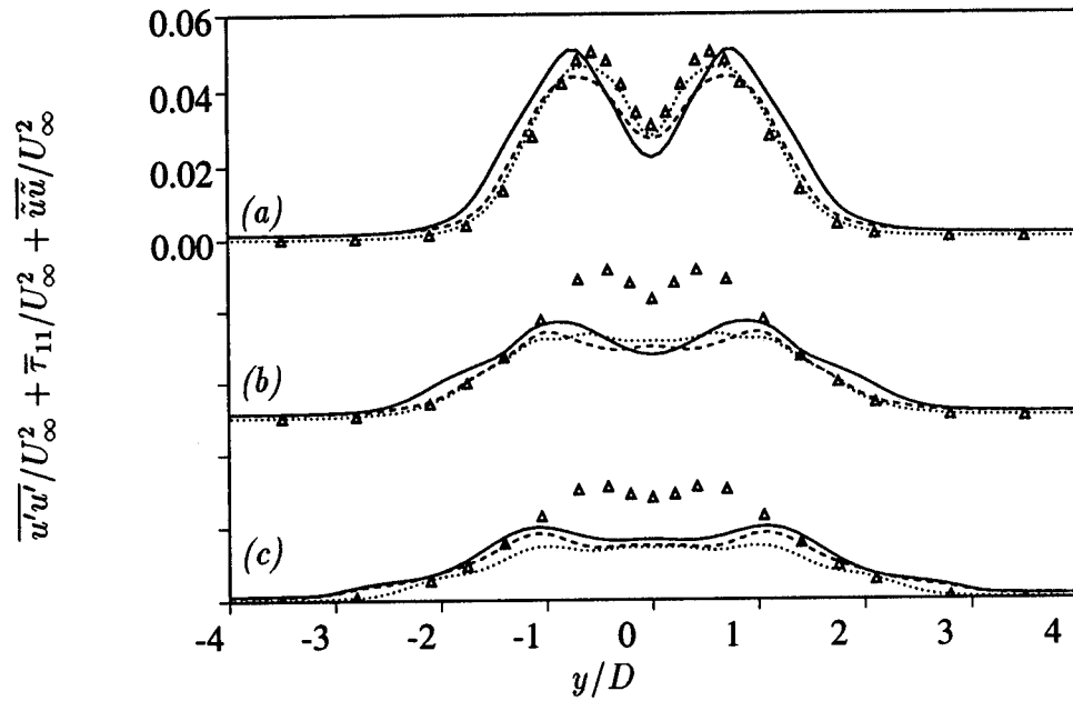
Figure 28: Re = 3,900 ; Total streamwise Reynolds stresses at x/D = 4 (a); 7 (b); 10 (c)
