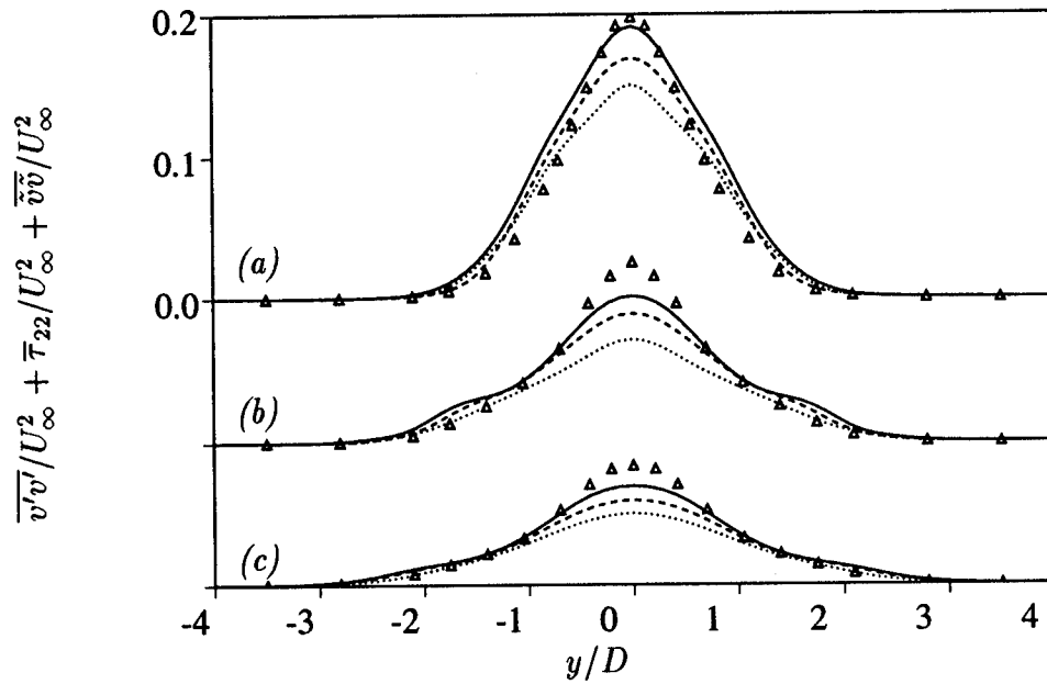
Figure 29: Re = 3,900 ; Total vertical Reynolds stresses at x/D = 4 (a); 7 (b); 10 (c)
