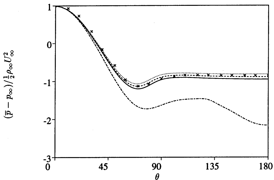
Figure 17: Re = 3,900 ; Wall pressure coefficient
