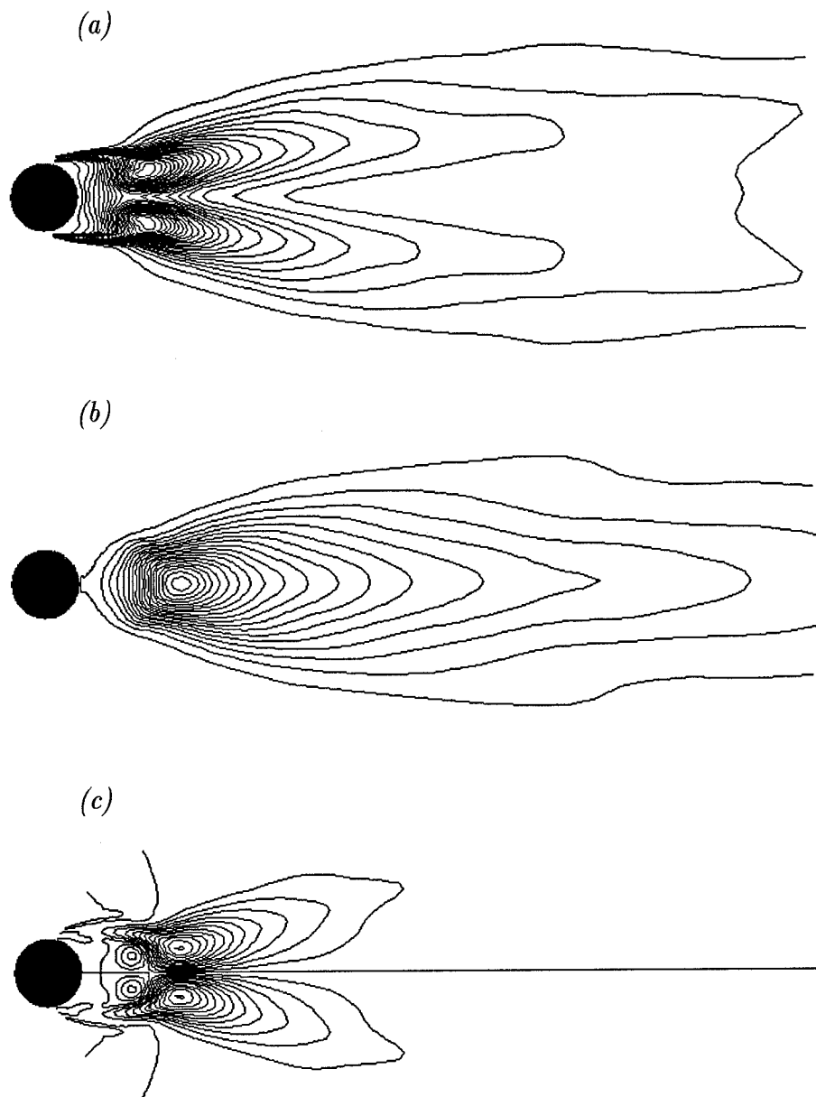
Figure 32: Re = 3,900 ; Time and spanwise averaged total Reynolds stresses in the first ten diameters of the wake
