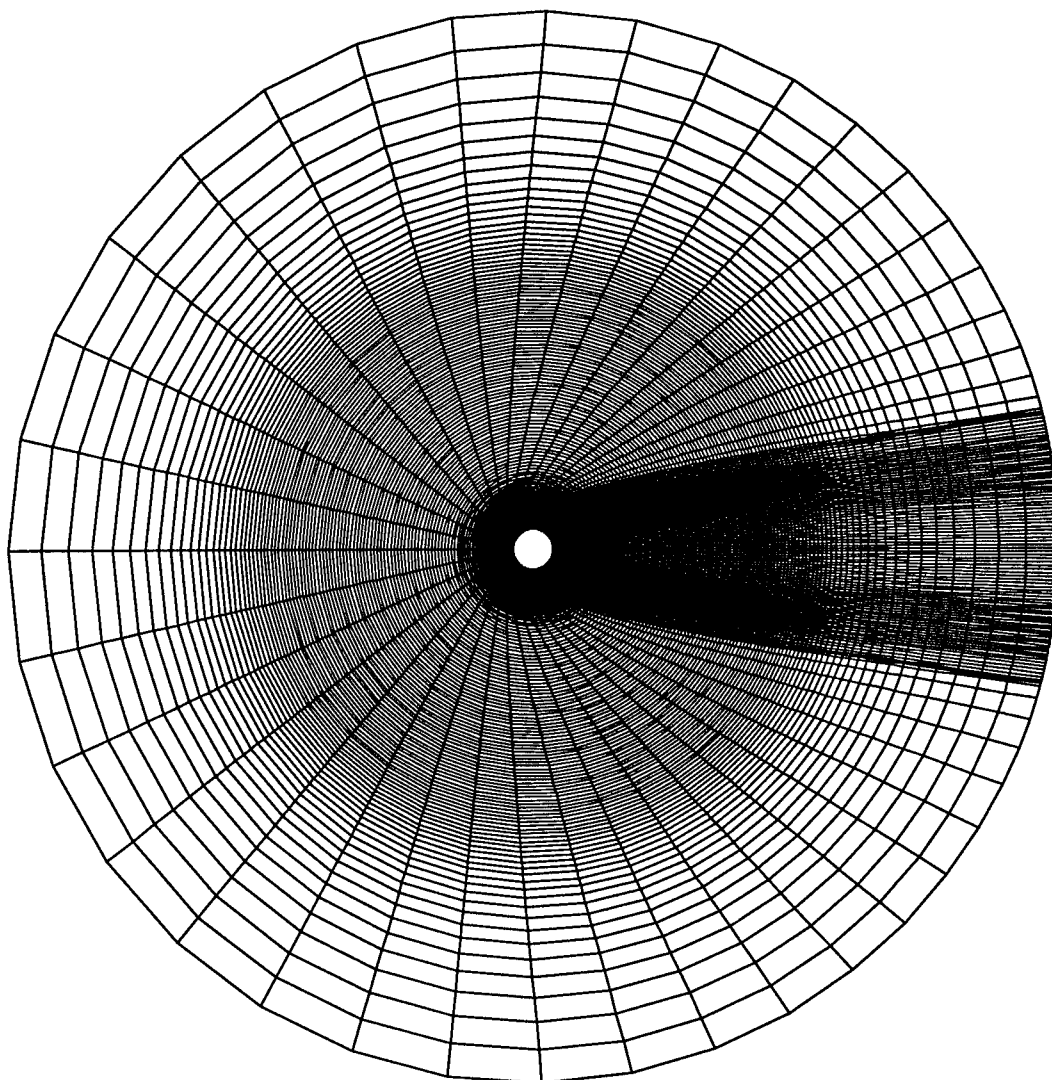
Figure 83: 174 \times 128 \times 48 planar grid within 13D of the cylinder
