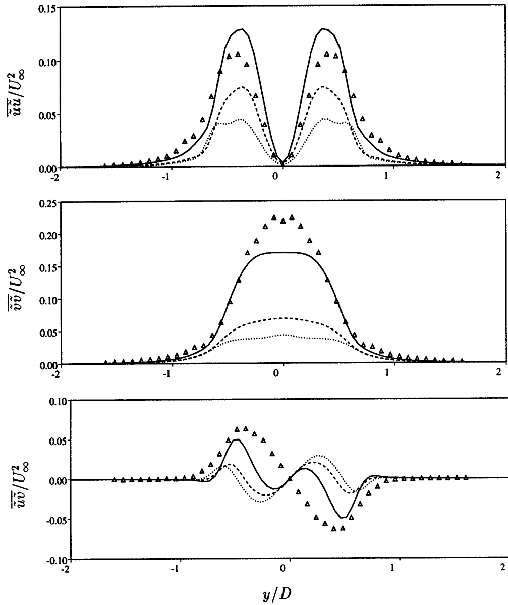
Figure 23: Re = 3,900 ; Periodic Reynolds stresses at x/D = 1.54 — : Dynamic model; ---- : No model; ... : Fixed coefficient model \triangle : Lourenco & Shih
