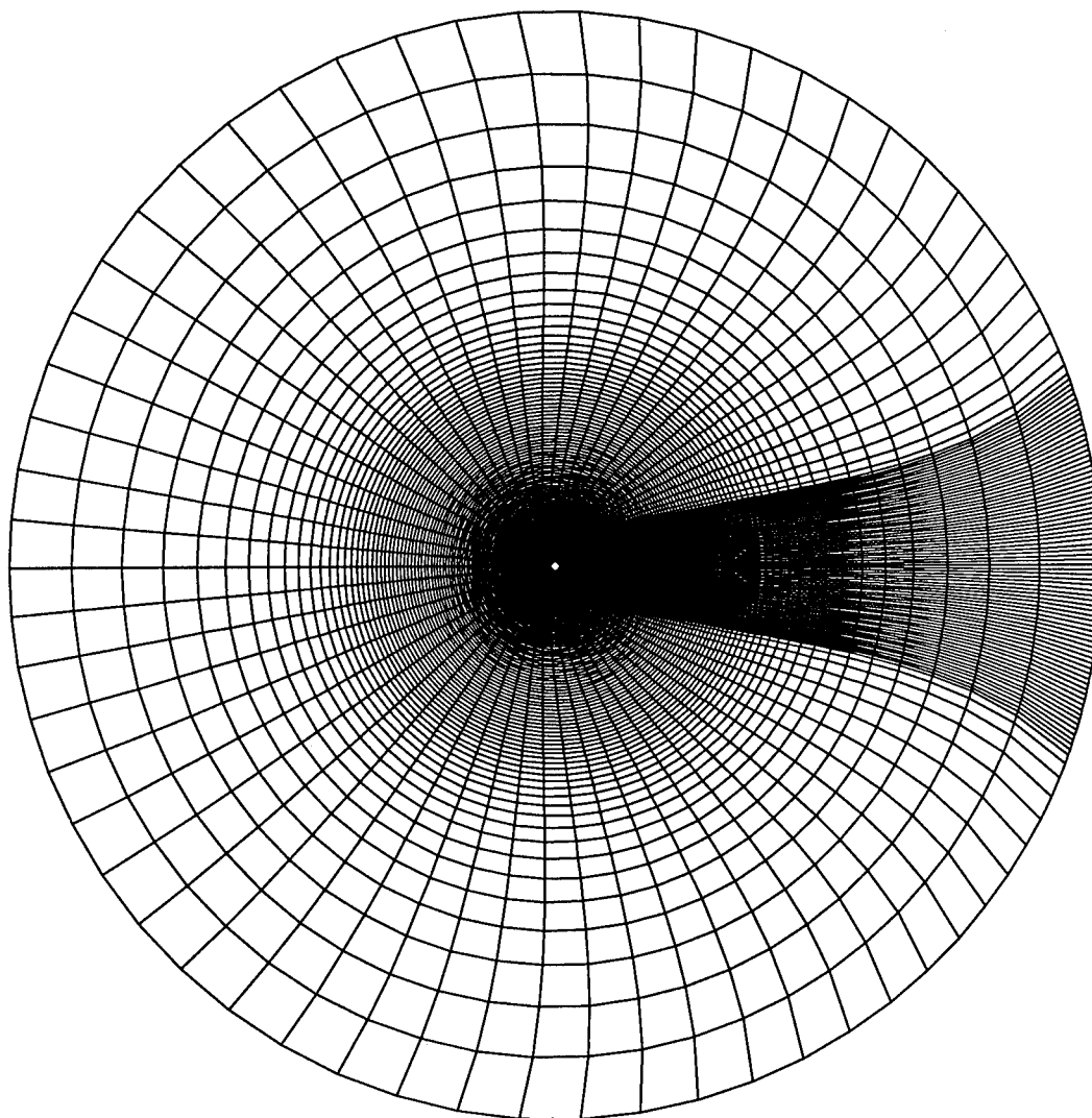
Figure 86: 144 \times 136 \times 48 grid on the entire domain
