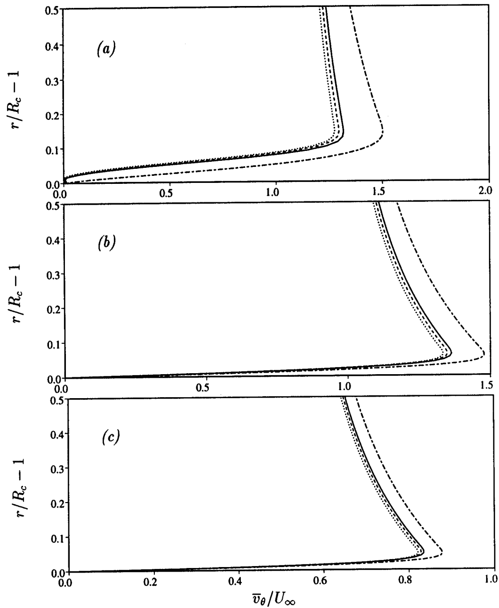
Figure 18: Re = 3,900 ; Tangential velocity in the cylinder surface boundary layer
