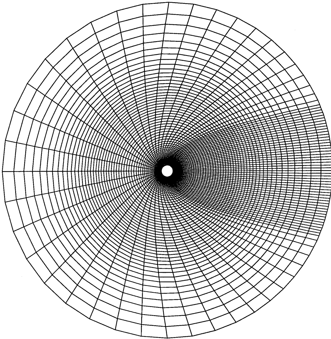
Figure 81: 88 \times 90 \times 32 and 88 \times 90 \times 48 meshes within 13D of the cylinder
