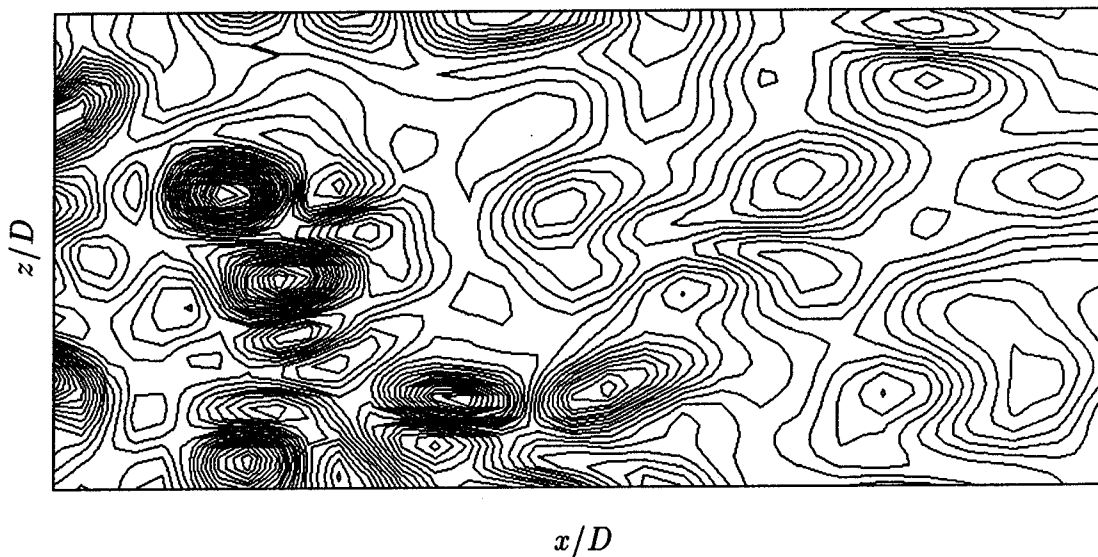
Figure 42: Re = 3,900 ; Instantaneous vertical vorticity at y = 0 , 5 \leq x/D \leq 10 , 0 \leq z \leq L_z . Dynamic model simulation.
