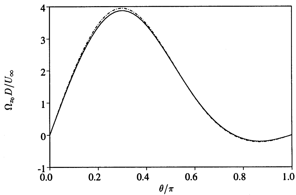
Figure 89: Re=20 ; Wall vorticity — : R_D/R_c = 60 ; ---- : R_D/R_c = 120 ; -·- : R_D/R_c = 300
