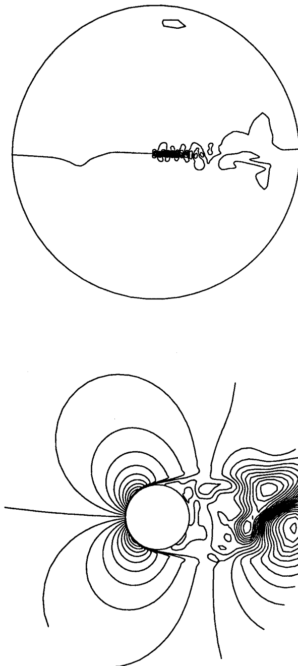
Figure 74: Re = 3,900 ; Instantaneous vertical velocity ( \rho v ) 144 \times 136 \times 48 Dynamic model simulation top : whole grid; bottom : cylinder vicinity
