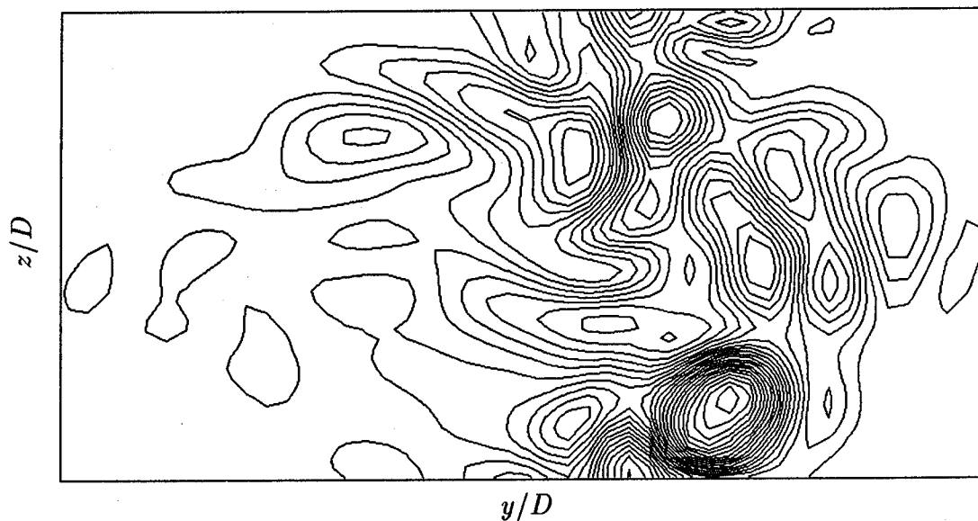
Figure 43: Re = 3,900 ; Instantaneous streamwise vorticity at r/D = 10 , -5 \leq y/D \leq 5 , 0 \leq z \leq L_z . Dynamic model simulation.
