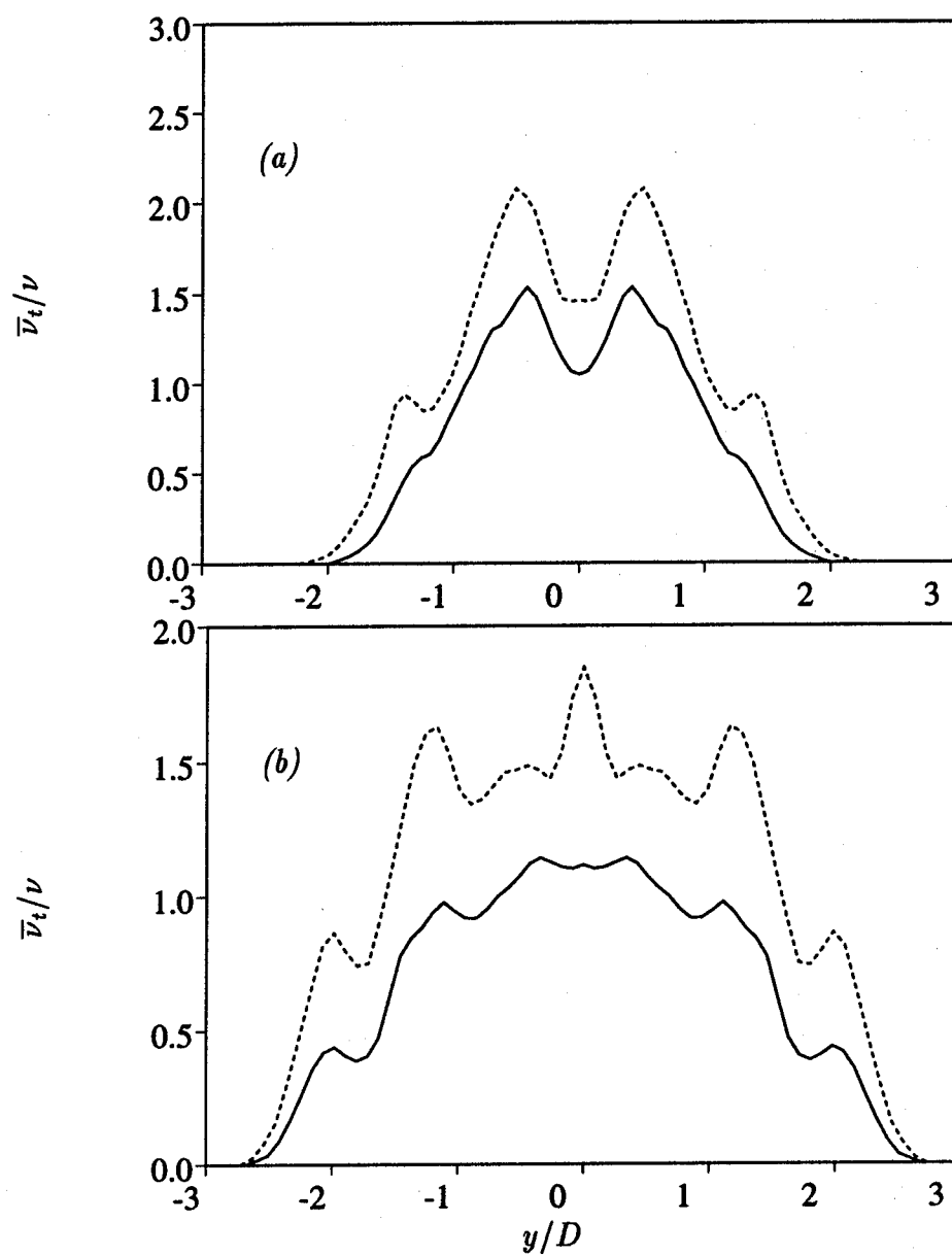
Figure 117: Eddy viscosity averaged over 1 shedding cycle — : No stretching; ---- : Stretched mesh x/D = 3.5 (a), 5.5 (b)
