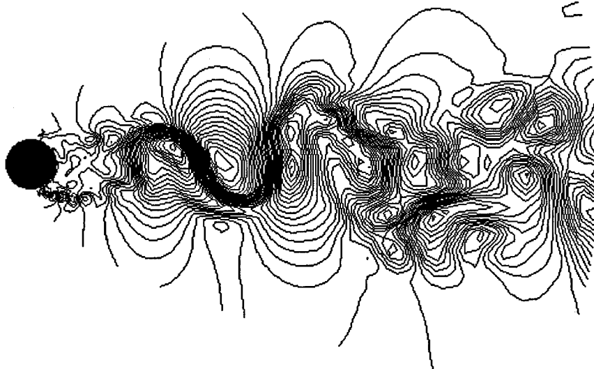
Figure 58: Re = 3,900 ; Instantaneous vertical velocity contours in the first 10 diameters of the vertical plane z = 0 (seventh-order scheme)
