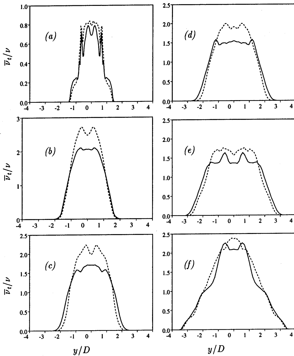
Figure 62: Re = 3,900 ; Mean eddy viscosity profiles
