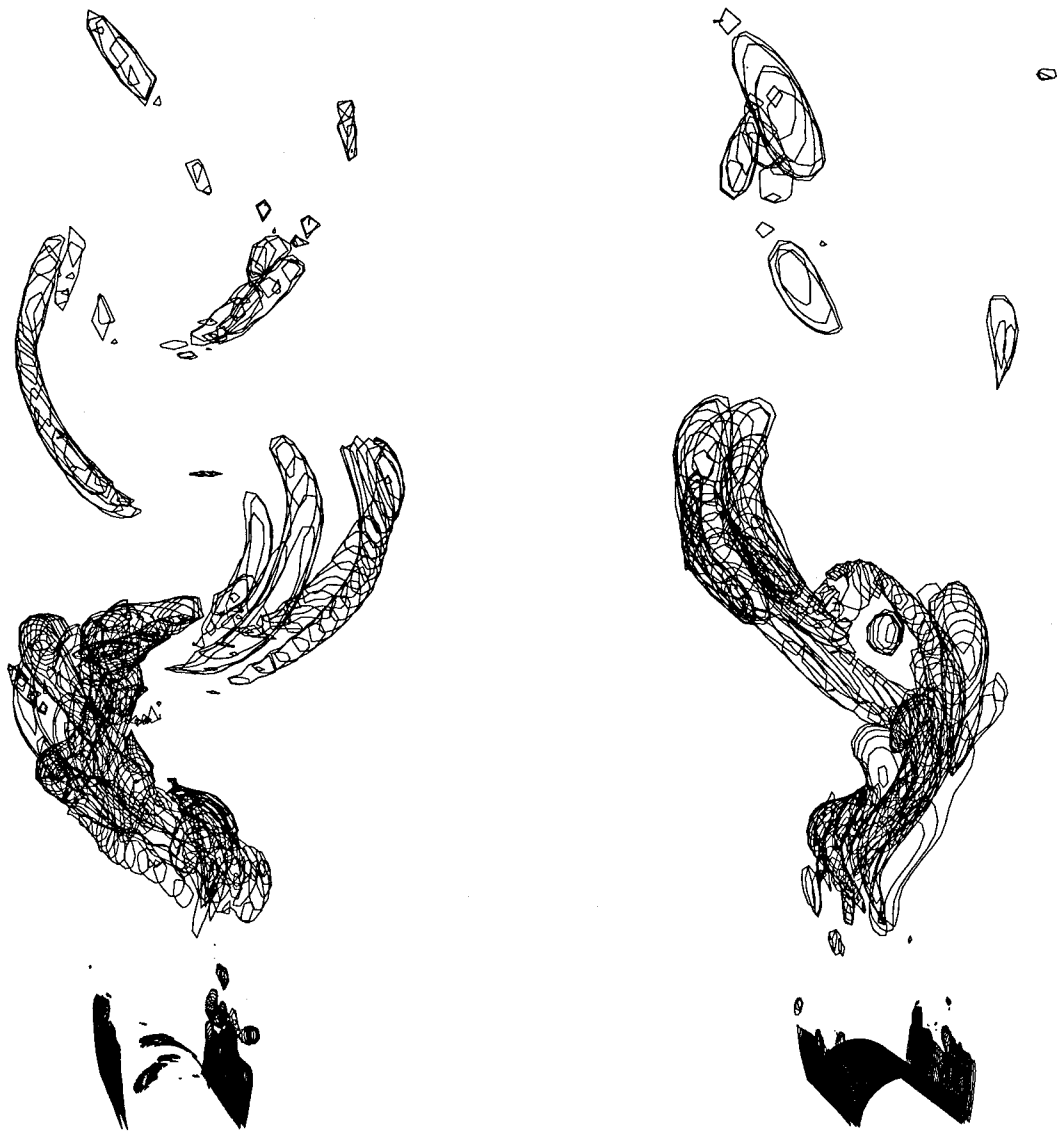
Figure 56: Re = 3,900 ; Instantaneous constant vorticity contours |\vec{\omega}D/u_d| = 6 left: 7 th order-accurate simulation; right: 5 th order-accurate simulation
