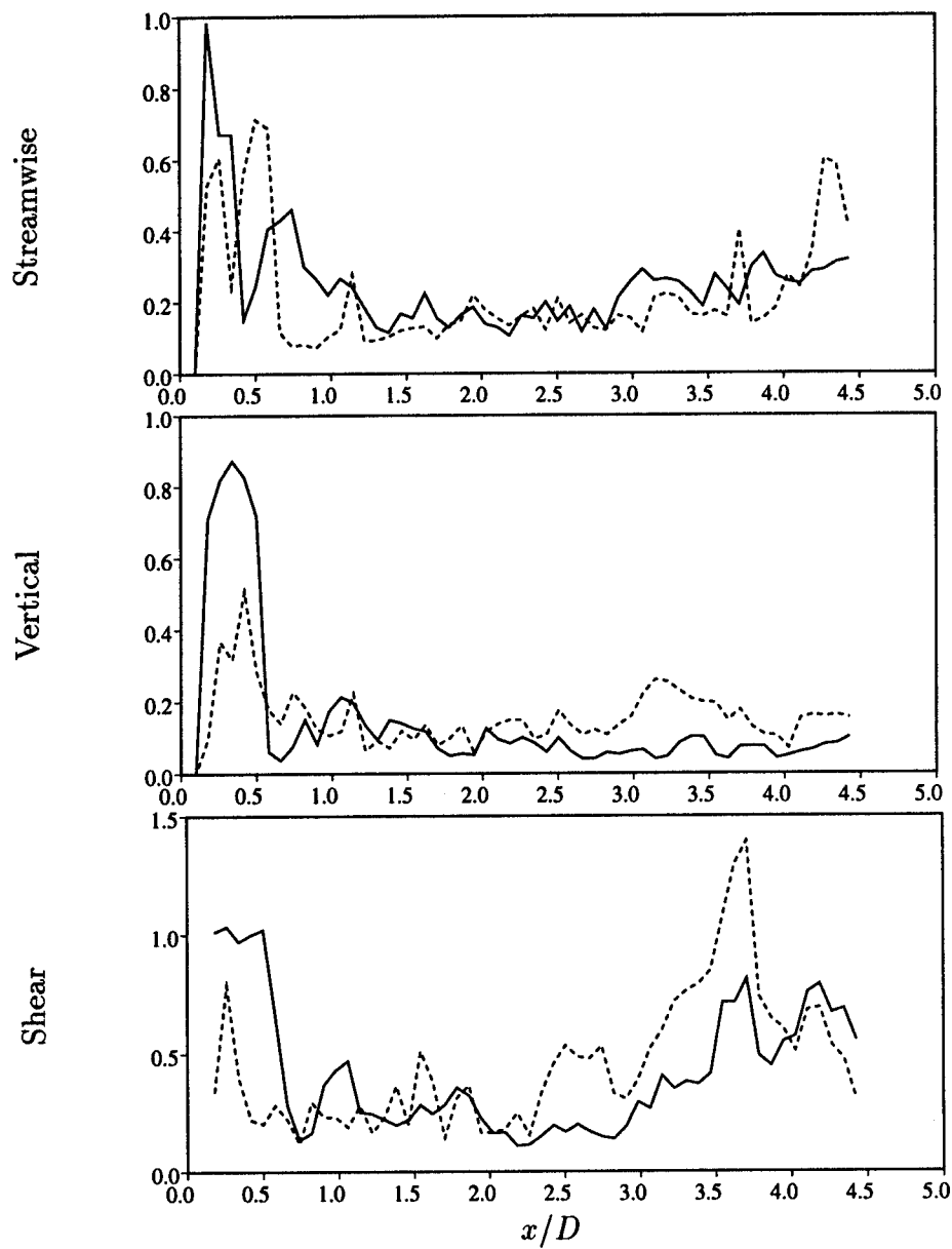
Figure 11: PIV experiment. Symmetry errors in periodic and turbulent Reynolds stresses
