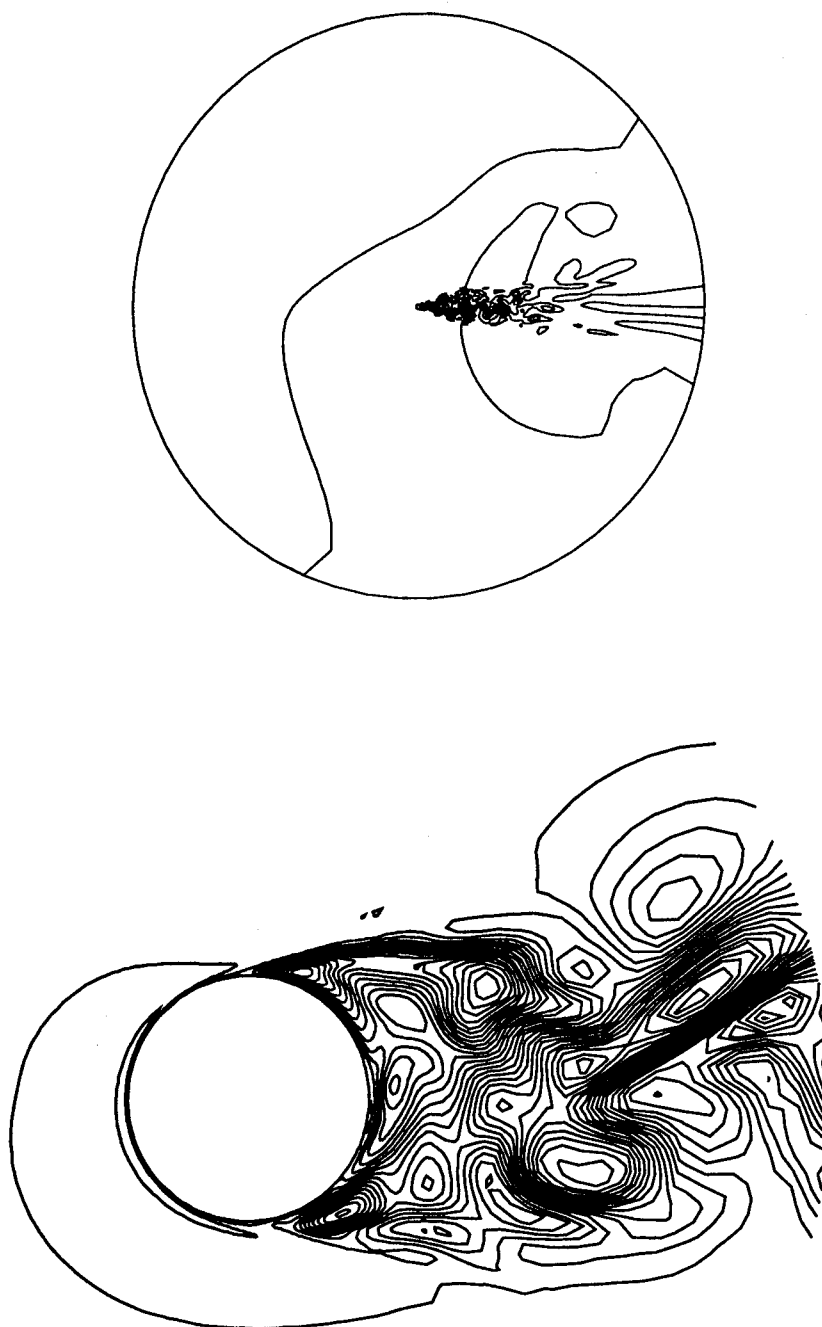
Figure 75: Re = 3,900 ; Instantaneous spanwise velocity ( \rho w ) 144 \times 136 \times 48 Dynamic model simulation top : whole grid; bottom : cylinder vicinity
