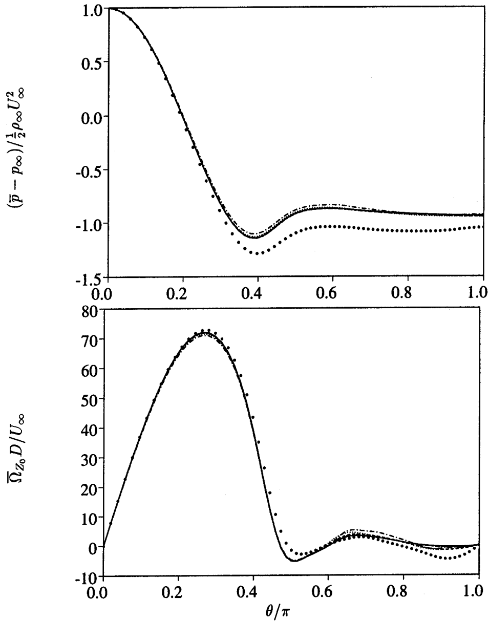
Figure 106: Wall pressure and vorticity convergence Shedding cycles: \bullet : 1; --- : 2; \cdots : 3; - \cdot - : 4; ---- : 5; —— : 6
