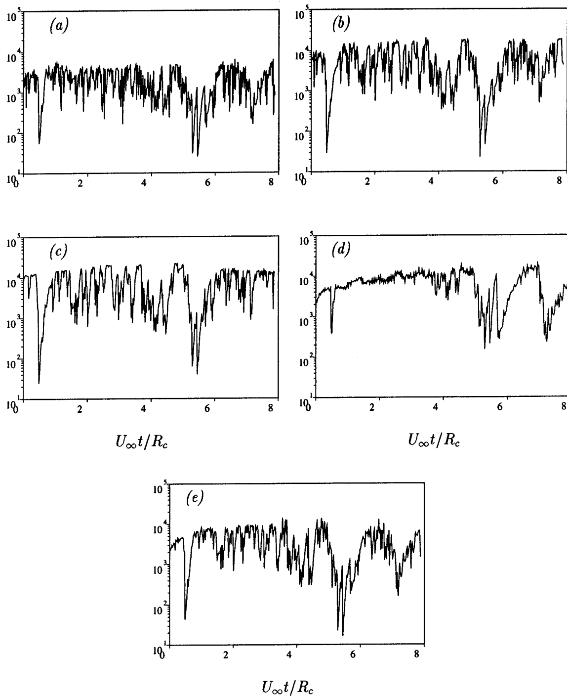
Figure 105: Sub-iteration convergence factor ( \|R^{n,1}\|_1 / \|R^{n,3}\|_1 ) time history ( 88 \times 90 \times 48 ) Simulation; Continuity (a); Streamwise Momentum (b) Vertical Momentum (c); Spanwise Momentum (d); Energy (e)
