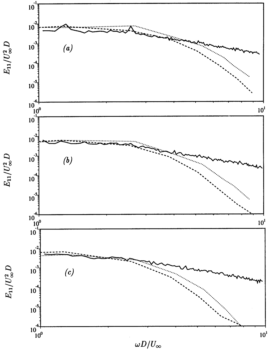
Figure 59: Re = 3,900 ; One-dimensional frequency spectra E_{11}(\omega) at (a): x/D = 5 ; (b) : x/D = 7 ; (c): x/D = 10 \cdots : 7 th order scheme; ---- : 5 th order scheme; — : Ong & Wallace
