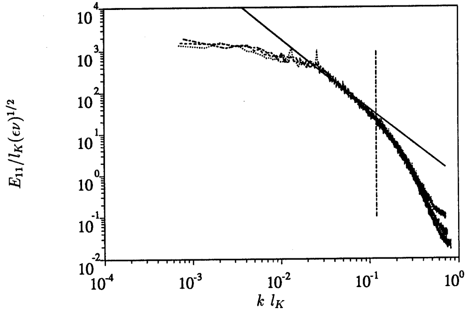
Figure 40: Re = 3,900 ; Experimental velocity power spectra E_{11} at y = 0 (Ong & Wallace, 1994); \cdots : x/D = 5 ; ---- : x/D = 7 ; -.- : x/D = 10 ; — : k^{-5/3} ; ---- grid cutoff at x/D = 10
