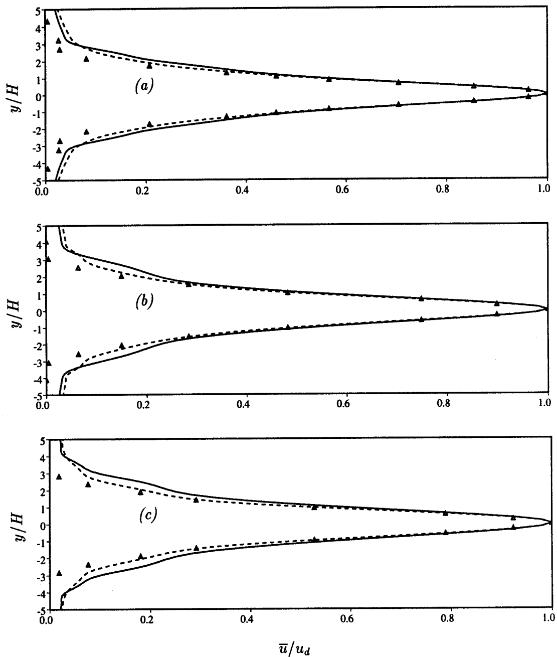
Figure 67: Re = 3,900 ; Streamwise velocity at x/D = 5 (a); 7 (b); 10 (c) — : 5 th order scheme; ---- : 7 th order scheme \triangle : Ong & Wallace
