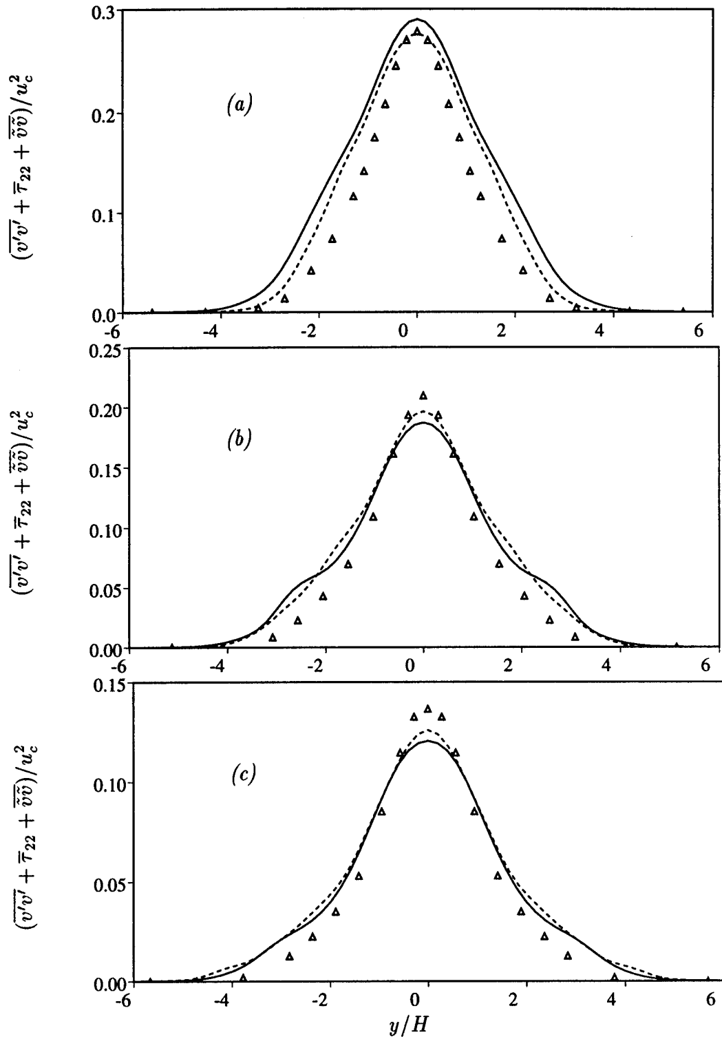
Figure 69: Re = 3,900 ; Vertical Reynolds stresses at x/D = 5 (a); 7 (b); 10 (c) — : 5 th order scheme; ---- : 7 th order scheme; \triangle : Ong & Wallace
