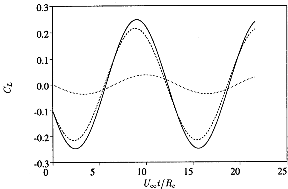
Figure 91: Re=80 ; Lift coefficient ---- : Pressure lift; ... : Viscous lift; — : Total lift
