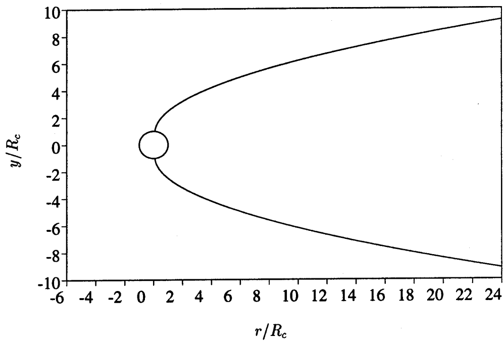
Figure 79: Near-wake envelope
