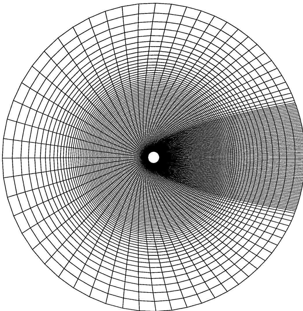
Figure 82: 116 \times 136 \times 48 mesh within 13D of the cylinder
