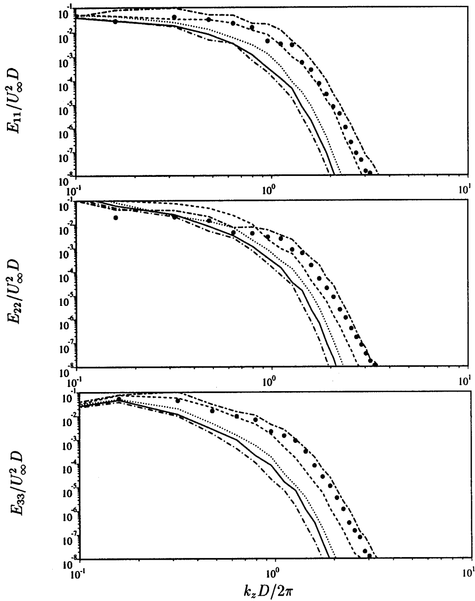
Figure 46: Re = 3,900 ; One-dimensional spectra E_{11} , E_{22} and E_{33} at y = 0 from the dynamic model simulation
