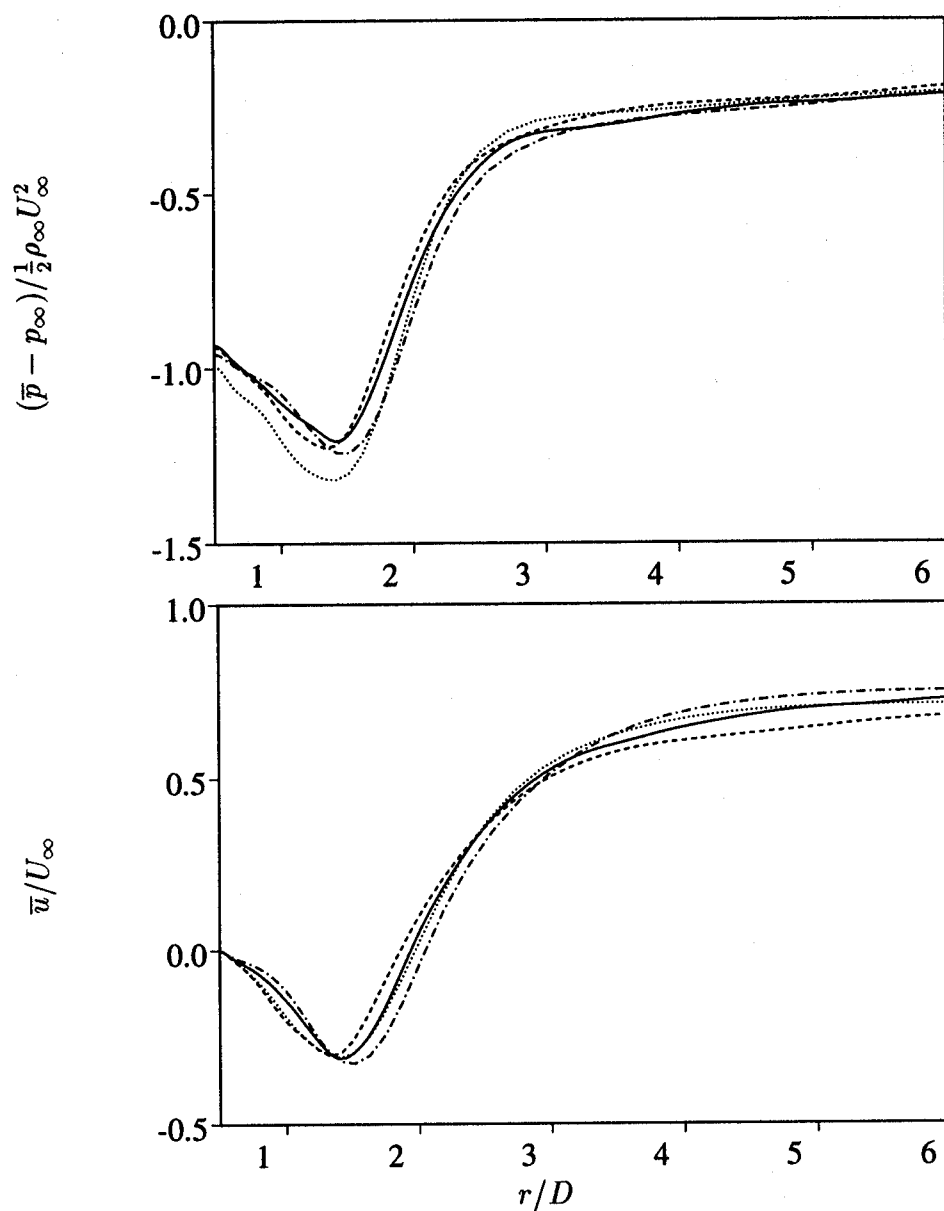
Figure 110: Rear axis pressure coefficient and streamwise velocity — : 88 \times 90 \times 32 ; \cdots : 88 \times 90 \times 48 - - - : 116 \times 136 \times 48 ; — : 174 \times 128 \times 48
