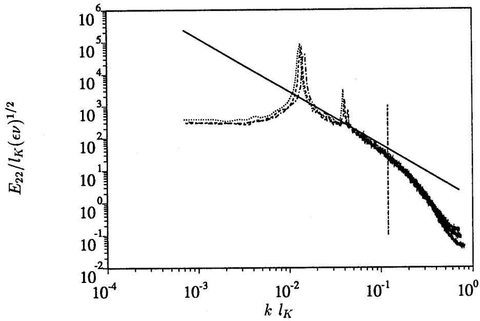
Figure 41: Re = 3,900 ; Experimental velocity power spectra E_{22} at y = 0 (Ong & Wallace, 1994); \cdots : x/D = 5 ; ---- : x/D = 7 ; -.- : x/D = 10 ; — : k^{-5/3} ; ---- grid cutoff at x/D = 10
