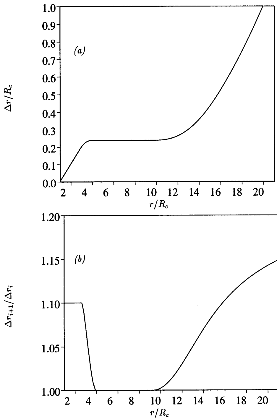
Figure 80: Near-wake radial spacing (a) and stretching ratio (b) distributions for the 116 \times 136 planar mesh
