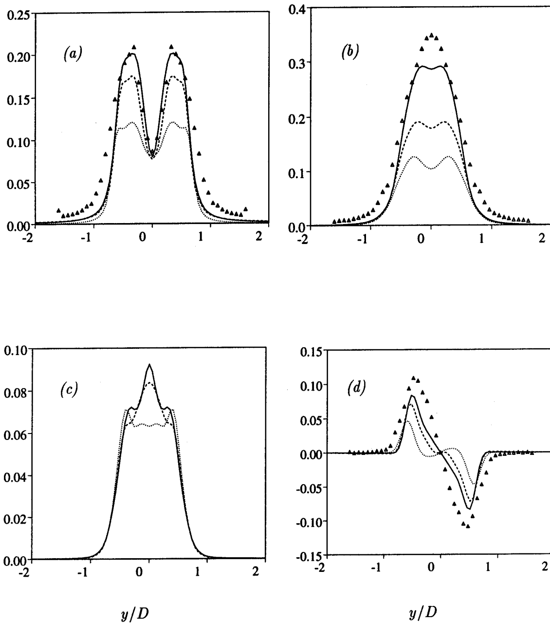
Figure 22: Re = 3,900 ; Total Reynolds stresses at x/D = 1.54
