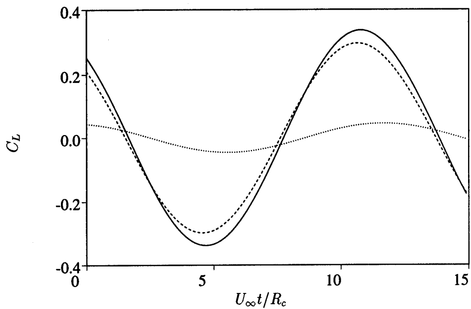
Figure 95: Re=100 ; Lift coefficient ---- : Pressure lift; ... : Viscous lift; — : Total lift
