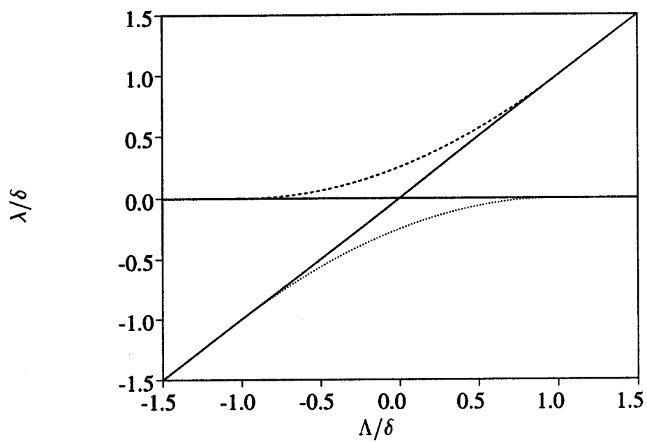
Figure 71: Eigenvalue smoothing near singular points ----- : \lambda^+/\delta ; ..... : \lambda^-/\delta
