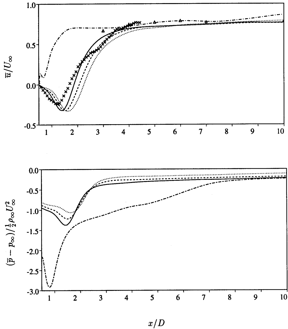
Figure 15: Re = 3,900 ; Centerline streamwise velocity and pressure coefficient — : Dynamic model; ---- : No model; ... : Fixed coefficient model -.- : 2D no model; \times : Lourenco & Shih; \triangle : Ong & Wallace
