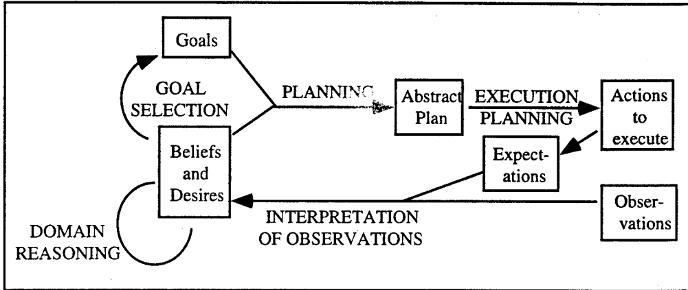
Figure 3: A model of a simple deliberative agent
