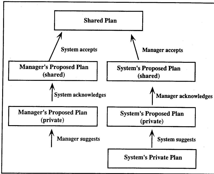
Figure 5: The different plan modalities in handling suggestions
