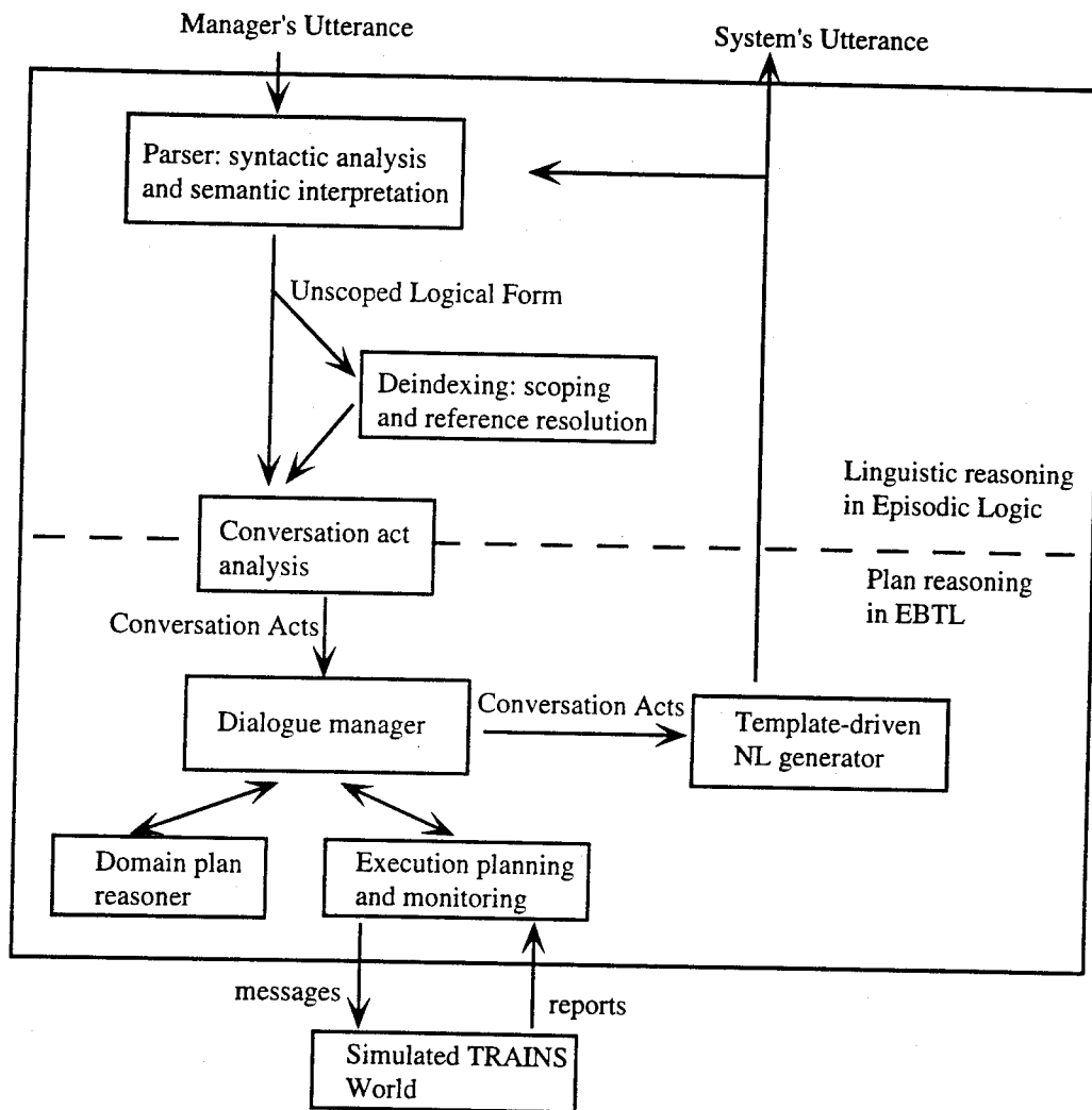
Figure 11: The TRAINS-93 System Architecture
