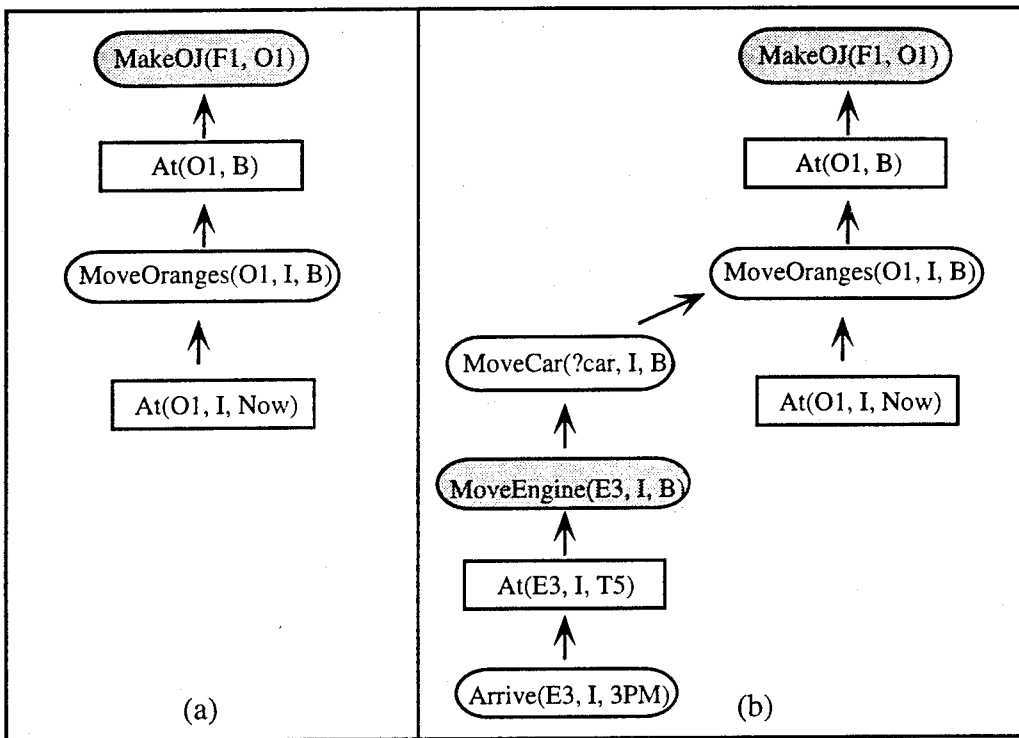
Figure 21: The plans after utterances (a) 1.3 and (b) 1.4 in the TRAINS-91 dialogue
