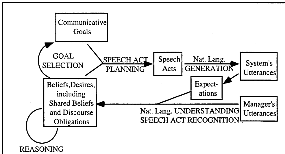
Figure 4: A model of TRAINS as a conversational agent
