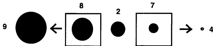
Figure 4: The Trajectory Mapping "TM" procedure. Two samples are picked at random and their extrapolants are found, as illustrated using the pair 8 and 7. Then, continuing to use the same feature for linking the samples, an interpolant is chosen.
