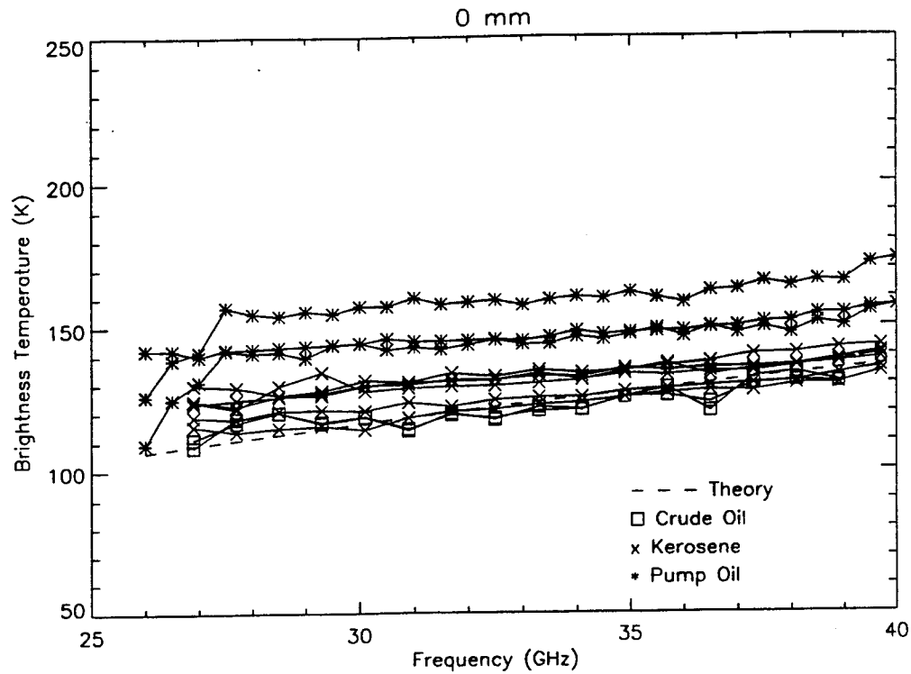
Figure 4-1. Oil Type Comparison, Water Only Measurement
