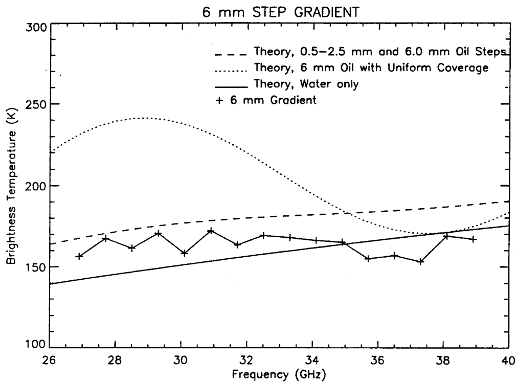
Figure C-24. Step Gradient, 6 mm Oil in Center Ring
