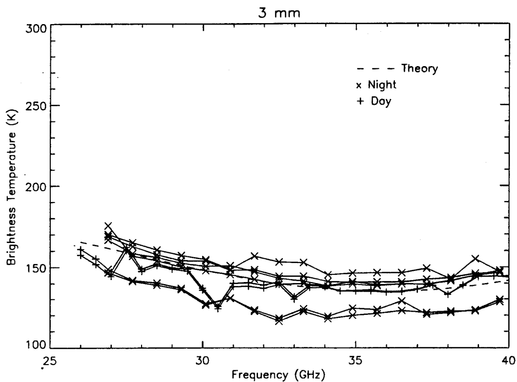
Figure A-12. Diurnal Comparison, 3 mm Uniform Thickness
