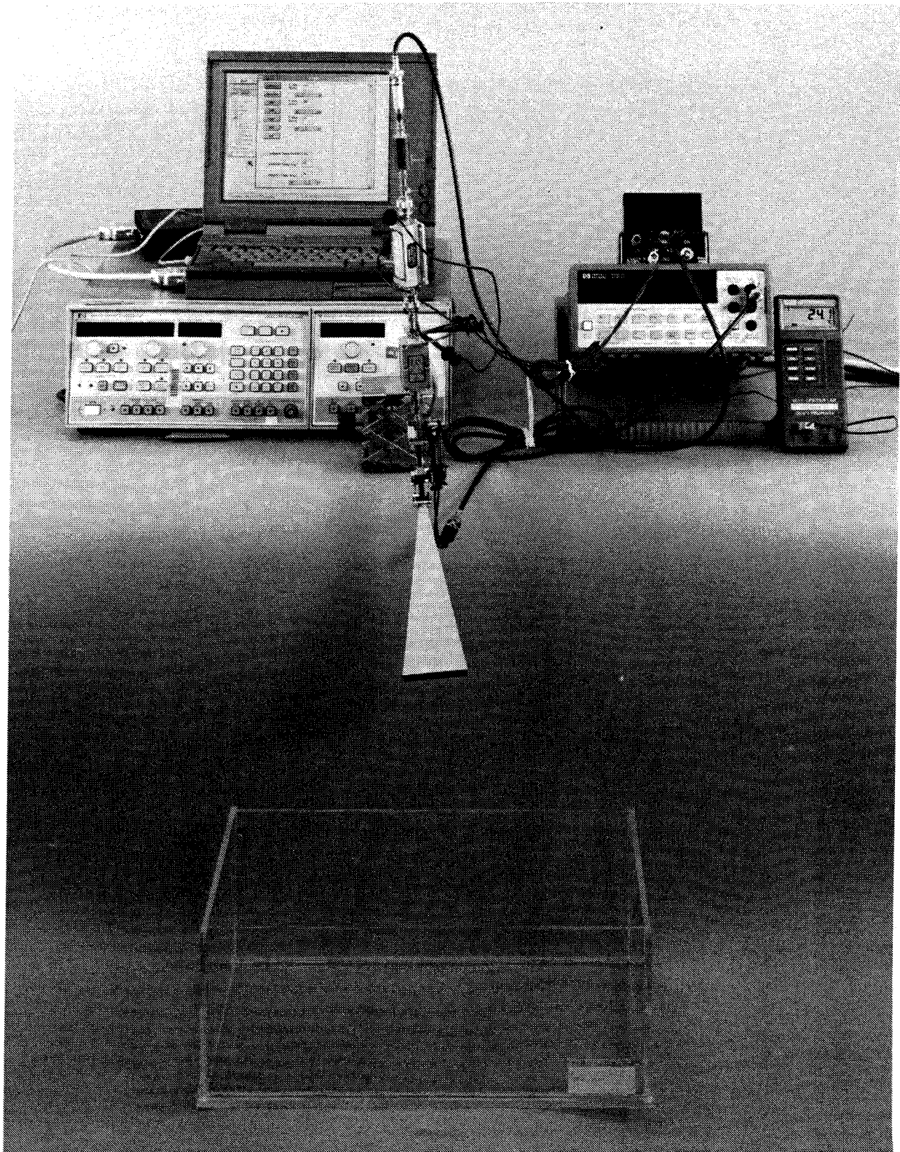
Figure 3-4. Interim FSR System During Receiver Characterization Tests
