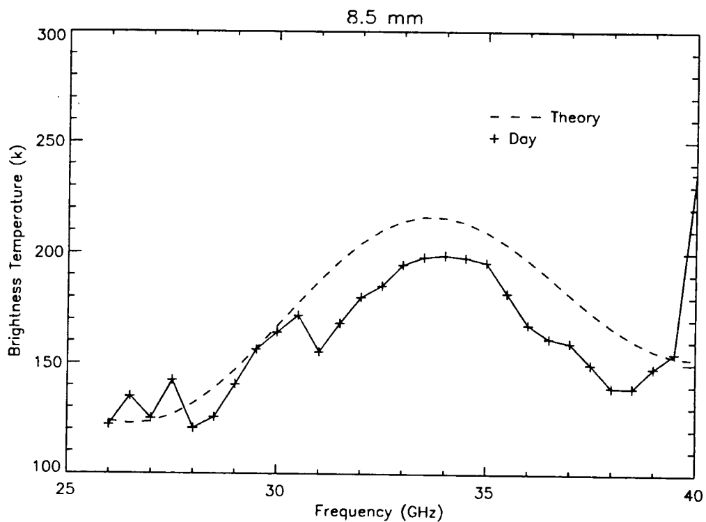
Figure A-22. Diurnal Comparison, 8.5 mm Estimated Thickness
