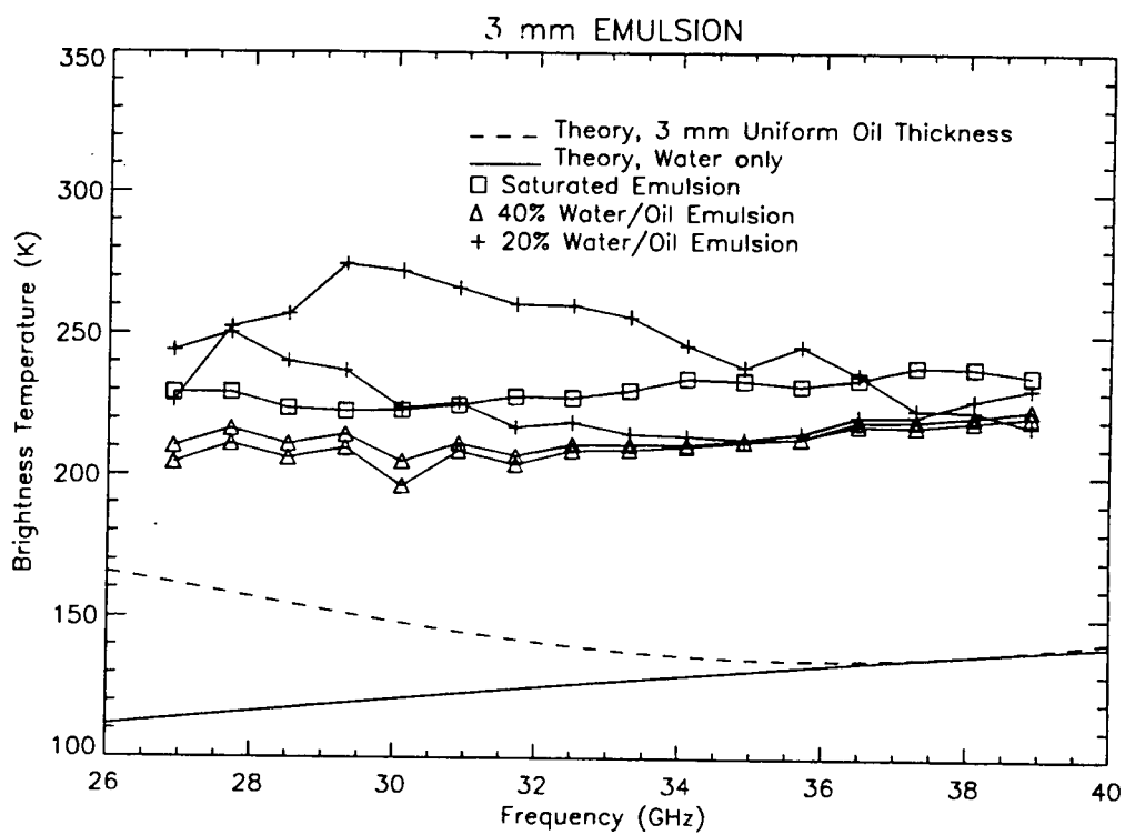
Figure B-3. Emulsified Oil, 3 mm Thickness
