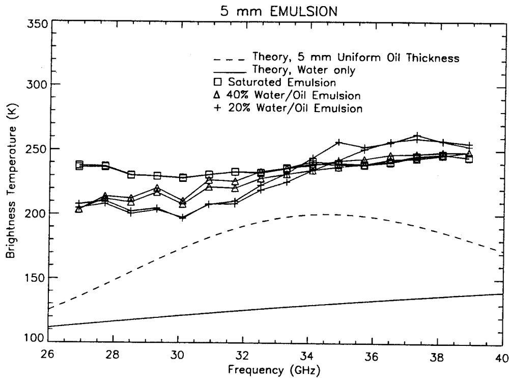
Figure 4-14. Emulsified Oil, 5 mm Thickness
