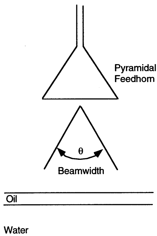
Figure 3-11. Antenna Beamwidth
