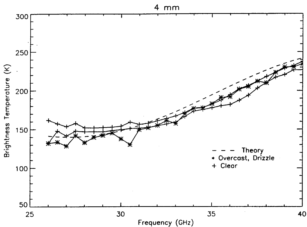
Figure A-24. Weather Comparison, 4 mm Uniform Thickness
