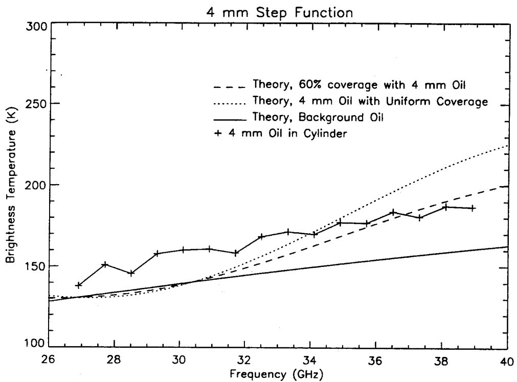
Figure C-16. Step Function, 4 mm Oil
