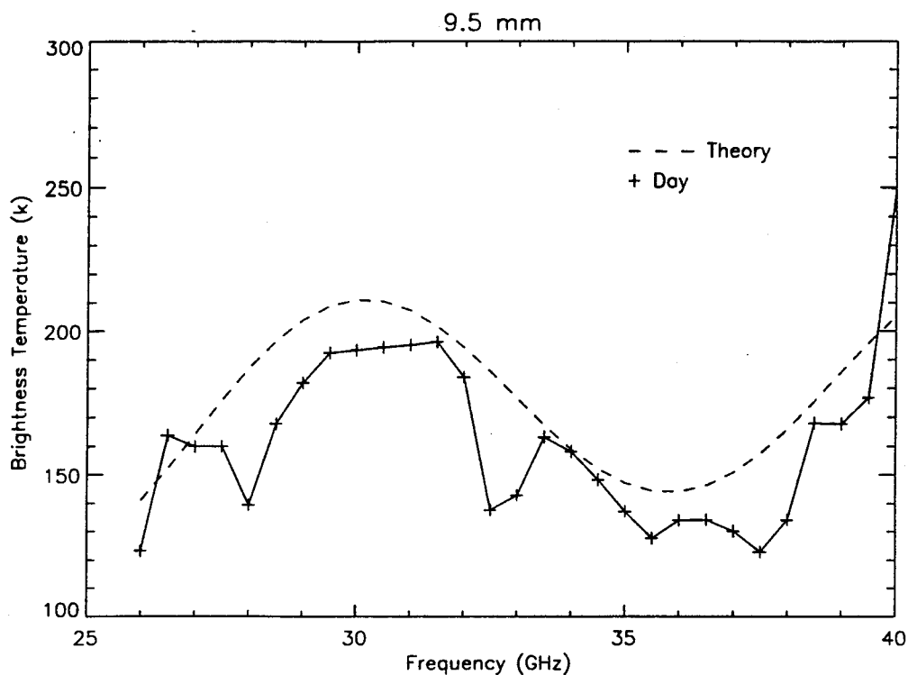
Figure A-23. Diurnal Comparison, 9.5 mm Estimated Thickness
