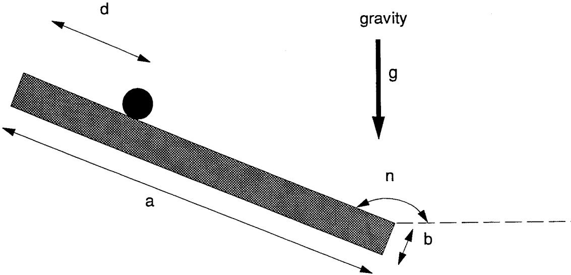
Figure 2-2: Particle on an Inclined Plane
