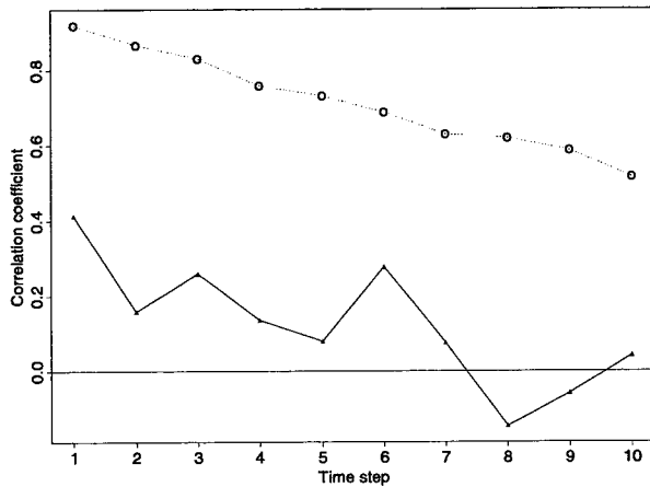
Figure 7: Plot of the correlation coefficient as a function of prediction-time step for the random noise observed in a semiconductor device. The embedding dimension is set to 3. Solid circles and solid line: Predictions on a test set of 50 points are made from a training set of 50 examples. Open circles dashed line: Predictions on a test set of 500 points and a training set of 500 examples.
