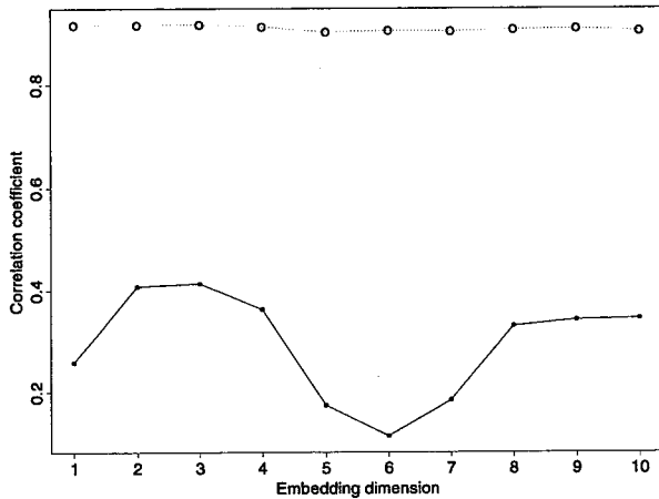
Figure 6: Plot of the correlation coefficient as a function of embedding dimension for colored noise with fractal dimension of 1.603. The random noise is not synthetic but a leakage-current fluctuations observed for a semiconductor device (Miyano et al., 1992). Solid circles and solid line: Predictions on a test set of 50 points are made from a training set of 50 examples. Open circles dashed line: Predictions on a test set of 500 points and a training set of 500 examples.
