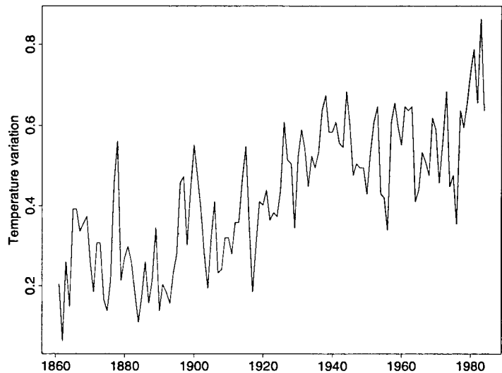
Figure 1: The global temperature variation as reported by Jones et al. (1986).
