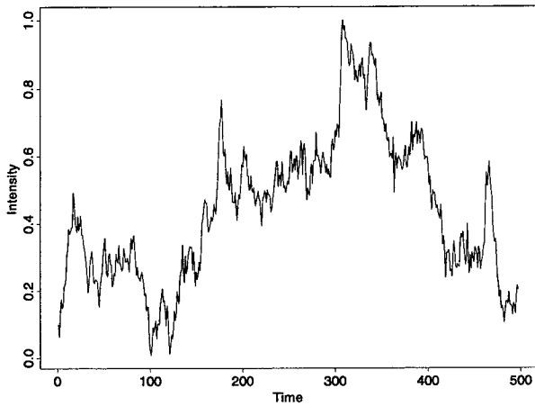
Figure 11: The f^{-1.8} -noise observed for a semiconductor device (Miyano, 1994; Miyano et al., 1992).
