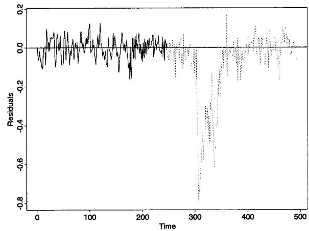
Figure 13: Residuals of the approximation of f^{-1.8} -noise by a Gaussian Hyper Basis Functions.
