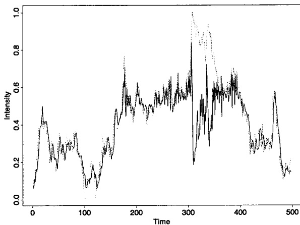
Figure 12: Results of training (from 0 to 249) and predictions (from 250 to 500) of the f^{-1.8} -noise using Gaussian Hyper Basis Functions without linear terms. The embedding dimension is set to 3. The network is trained for first 250 library patterns, i.e., the time series from time = 0 to 250. The predictions agree well with the targets except for the portion from time = 300 to 350 during which the network forecasts lower values than observed.
