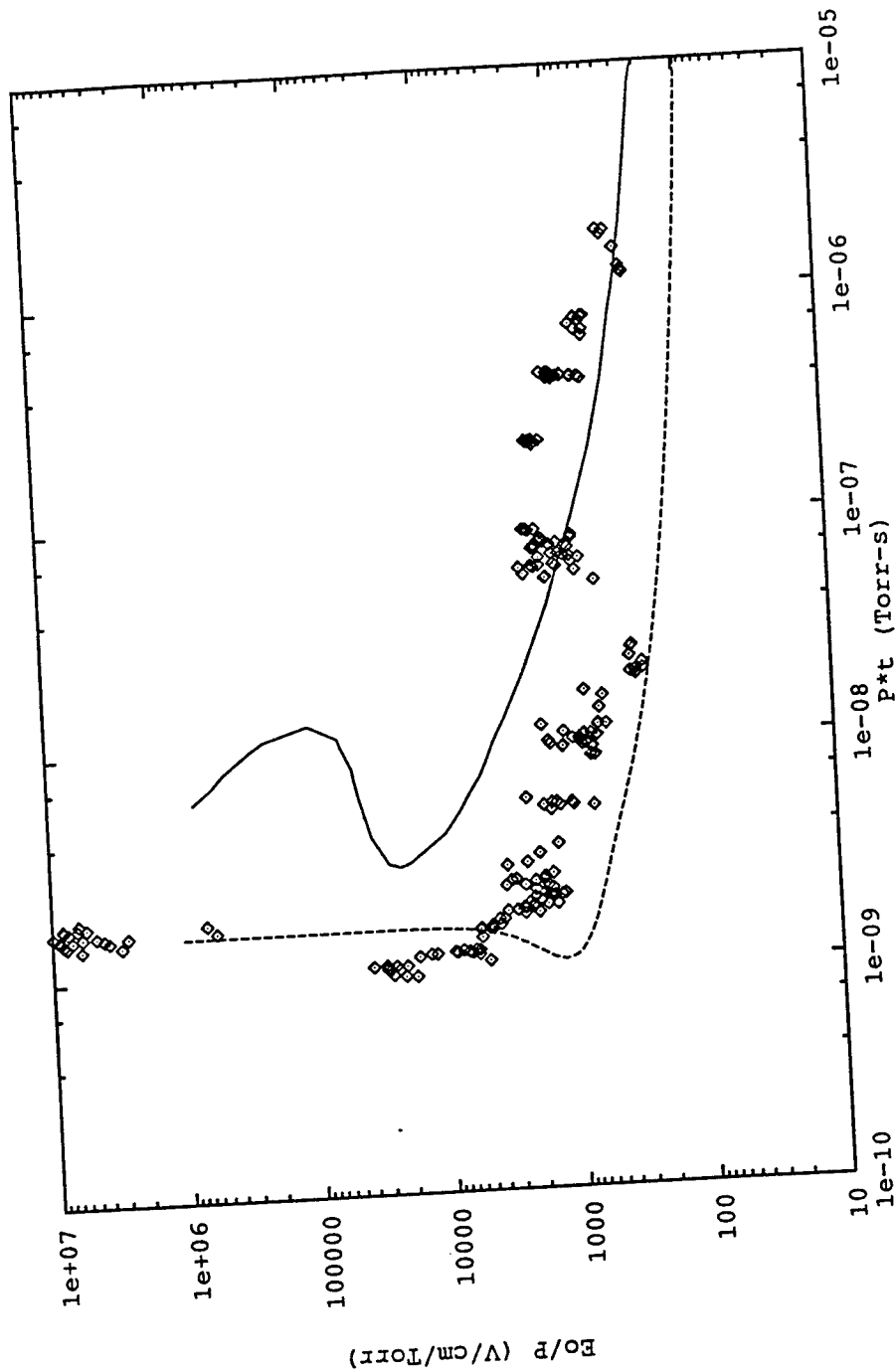
Figure 22. Edited E_0/P vs. P \tau_p Data Compared to Classical and Relativistic Theory
