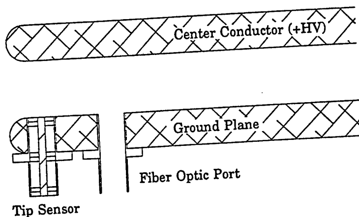
Figure 16. Tip Sensor.
