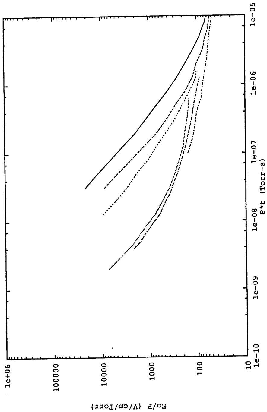
Figure 1. Prior E_0/P vs. P^*t_p Compilation of Previous Research
