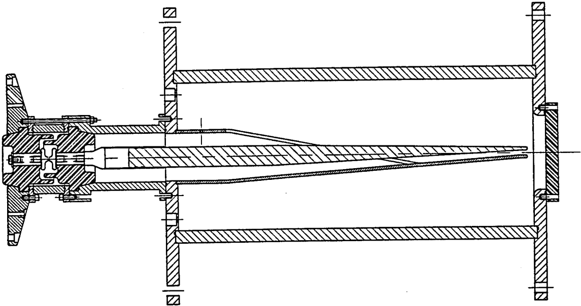
Figure 12. Test Chamber.
