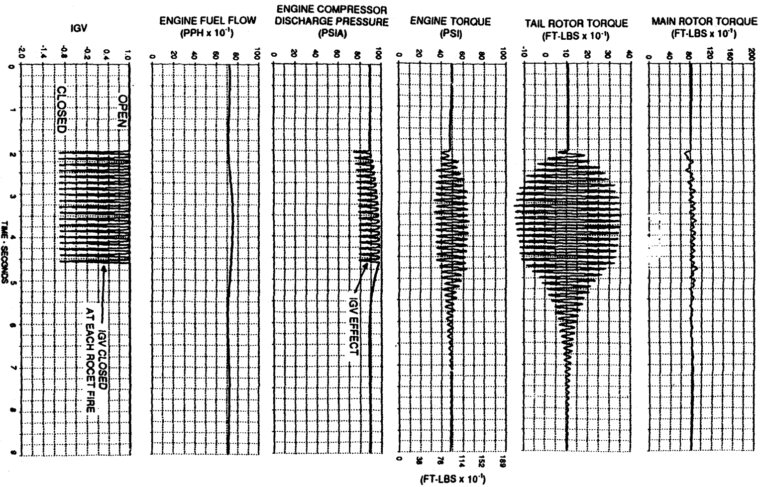
SIMULATION OF MULTIPLE (19) ROCKET FIRES (With IGV Synched to Rocket Fire)
