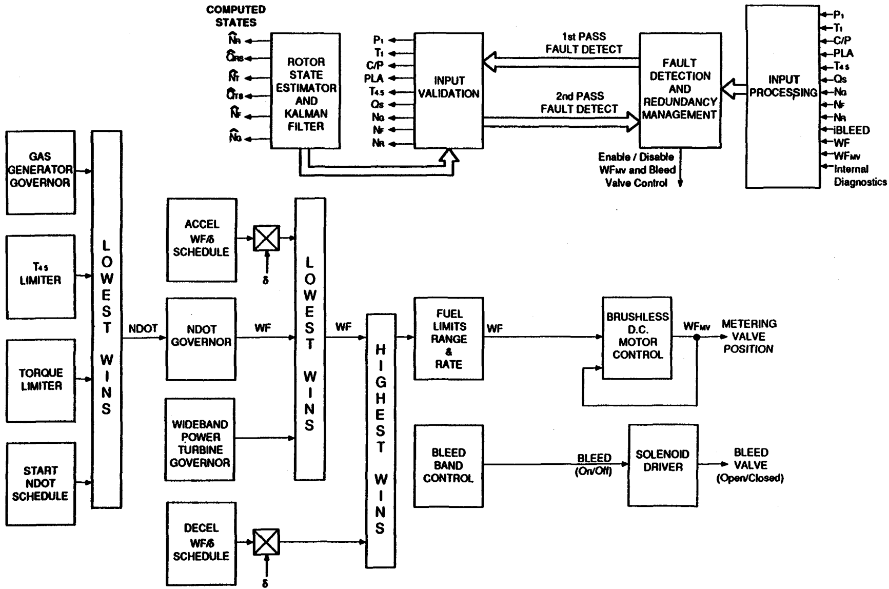
T53 FADEC ... SOFTWARE ARCHITECTURE Figure 25
