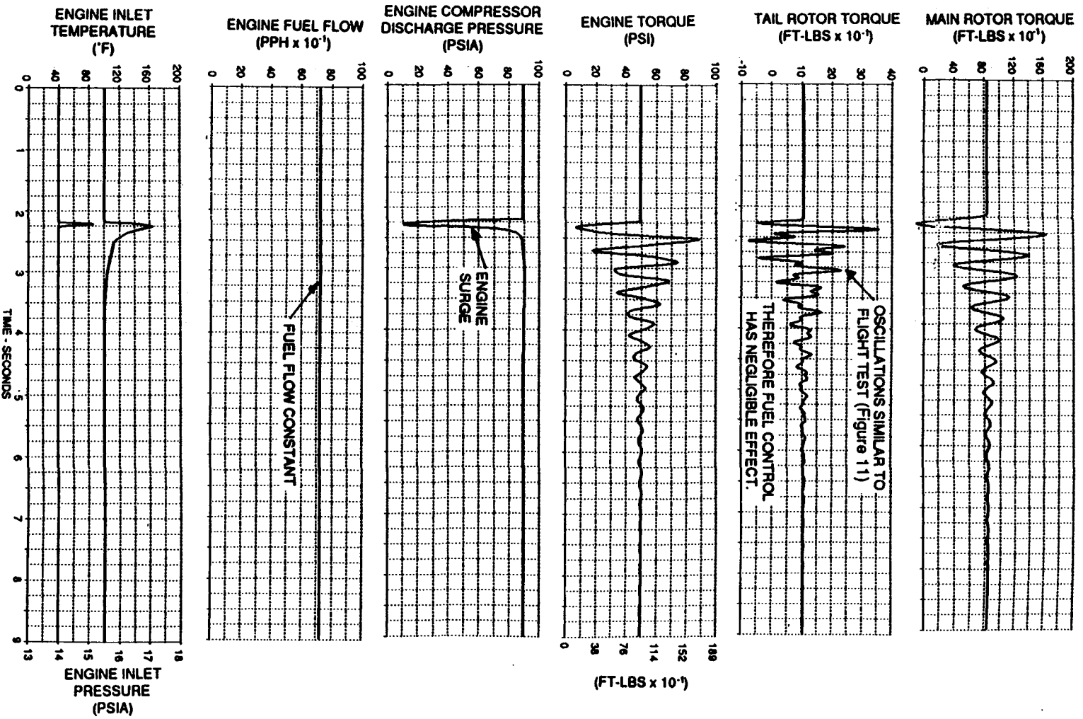
SIMULATION OF ROCKET FIRE FLIGHT TEST (1 PAIR) (With Fuel Flow Constant)
