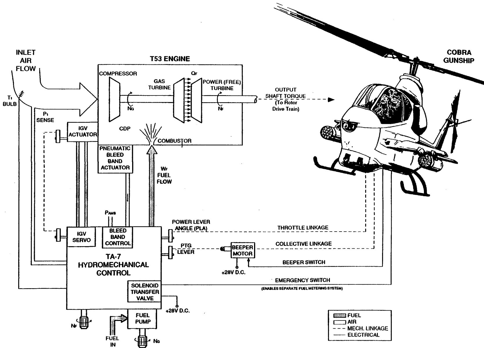
AH-1 / T53 ENGINE CONTROL SYSTEM
