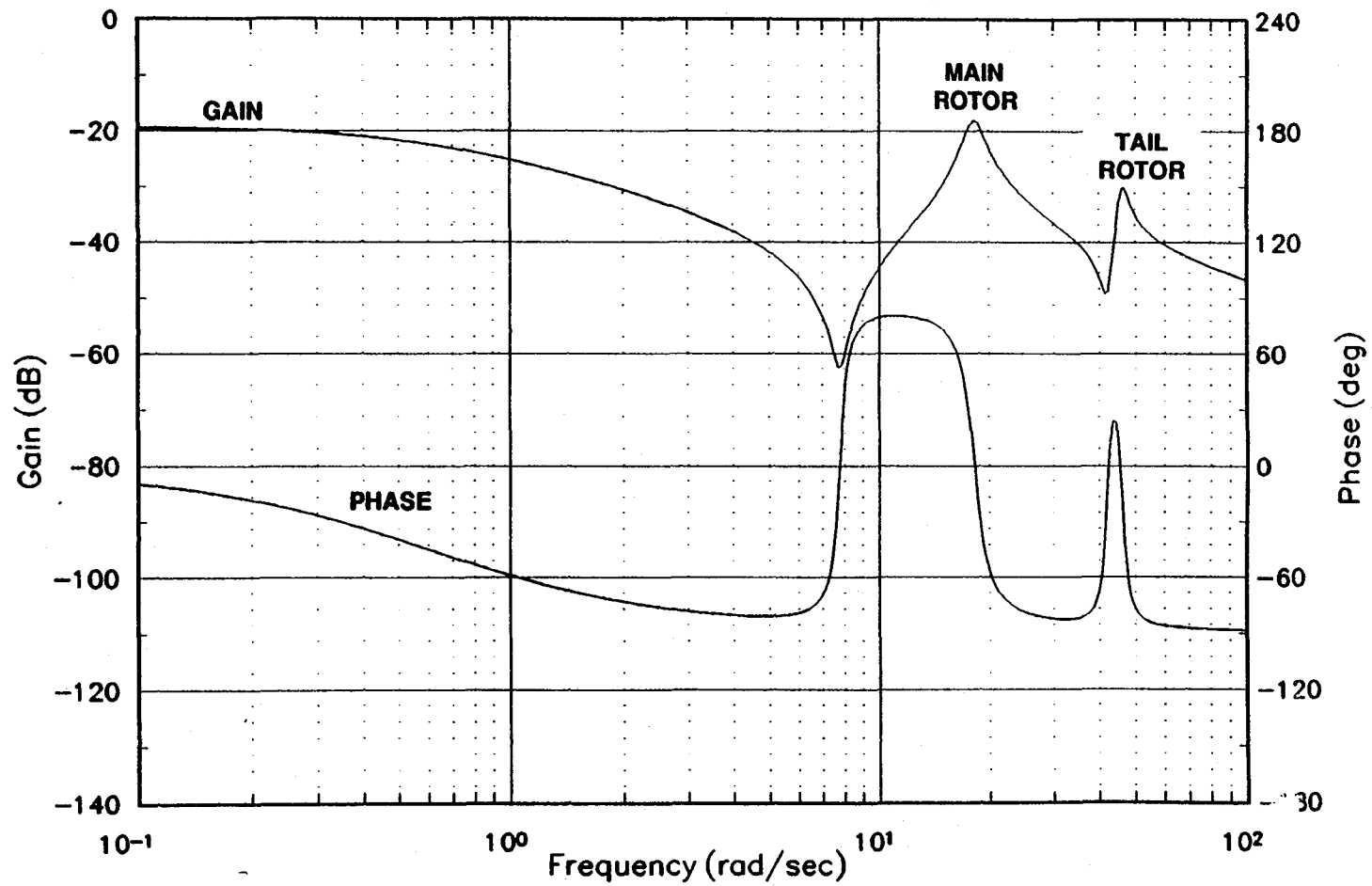
AH-1/T53 ROTOR DRIVE TRAIN FREQUENCY RESPONSE - NF/QF
