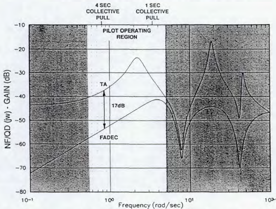
TORQUE DISTURBANCE REJECTION COMPARISON - NF/QD WIDEBAND GOVERNOR vs. TA CONTROL
