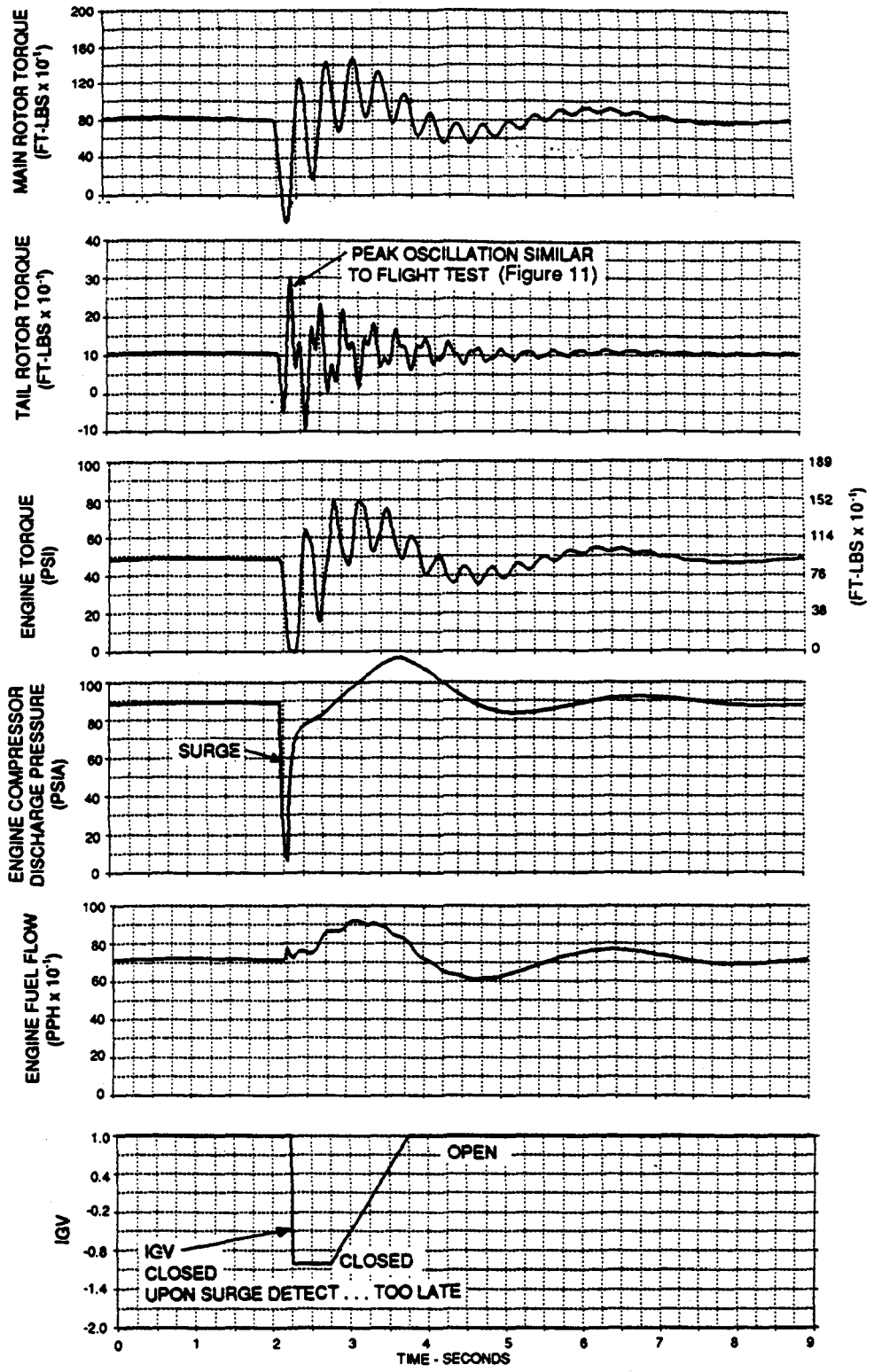
SIMULATION OF ROCKET FIRE FLIGHT TEST (1 PAIR) (With IGV Synced to Surge)
