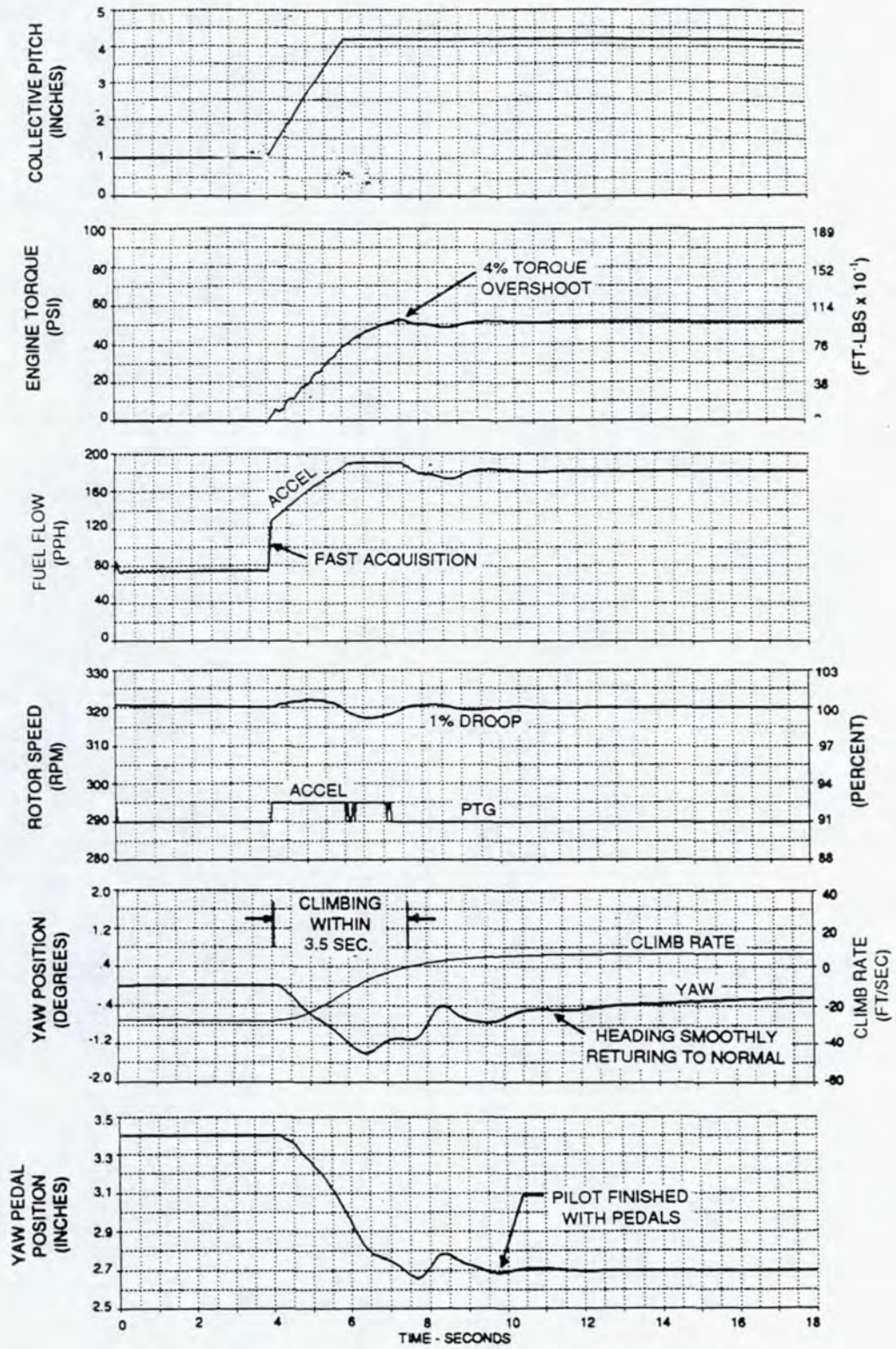
WIDEBAND ELECTRONIC PTG PERFORMANCE 2 Second Collective Pull from Low to High Power
