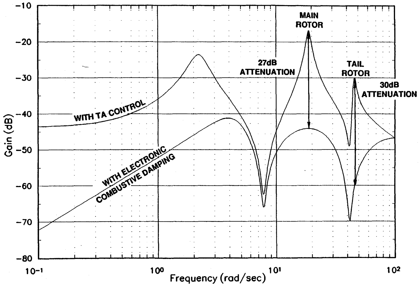
EFFECT OF ACTIVE DAMPING ON AH-1/T53 ROTOR TORSIONALS TORQUE DISTURBANCE REJECTION - NF/QD
