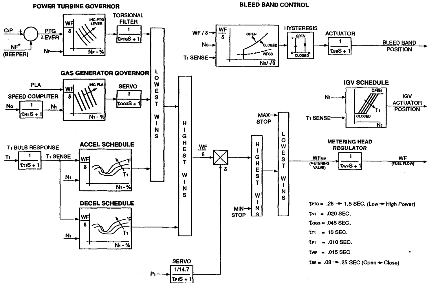
TA CONTROL SYSTEM . . . SIMPLIFIED FUNCTIONAL BLOCK DIAGRAM
