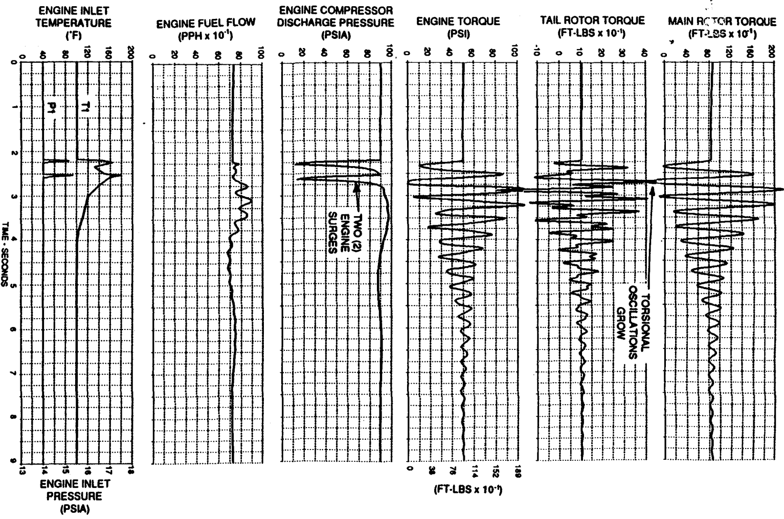
SIMULATION OF MULTIPLE ROCKET FIRES (3 PAIR)
