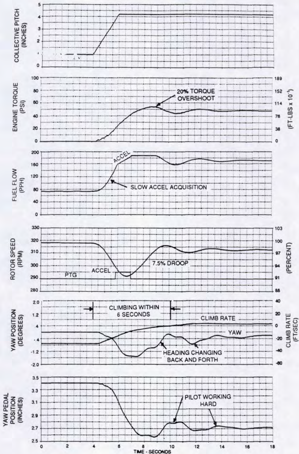
TA HYDROMECHANICAL PTG PERFORMANCE 2 Second Collective Pull from Low to High Power Figure 22
