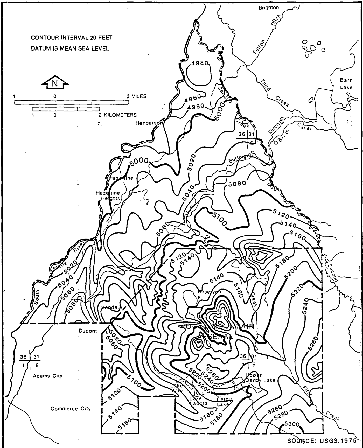
Figure 1.5-3 ELEVATIONS OF BEDROCK SURFACE
