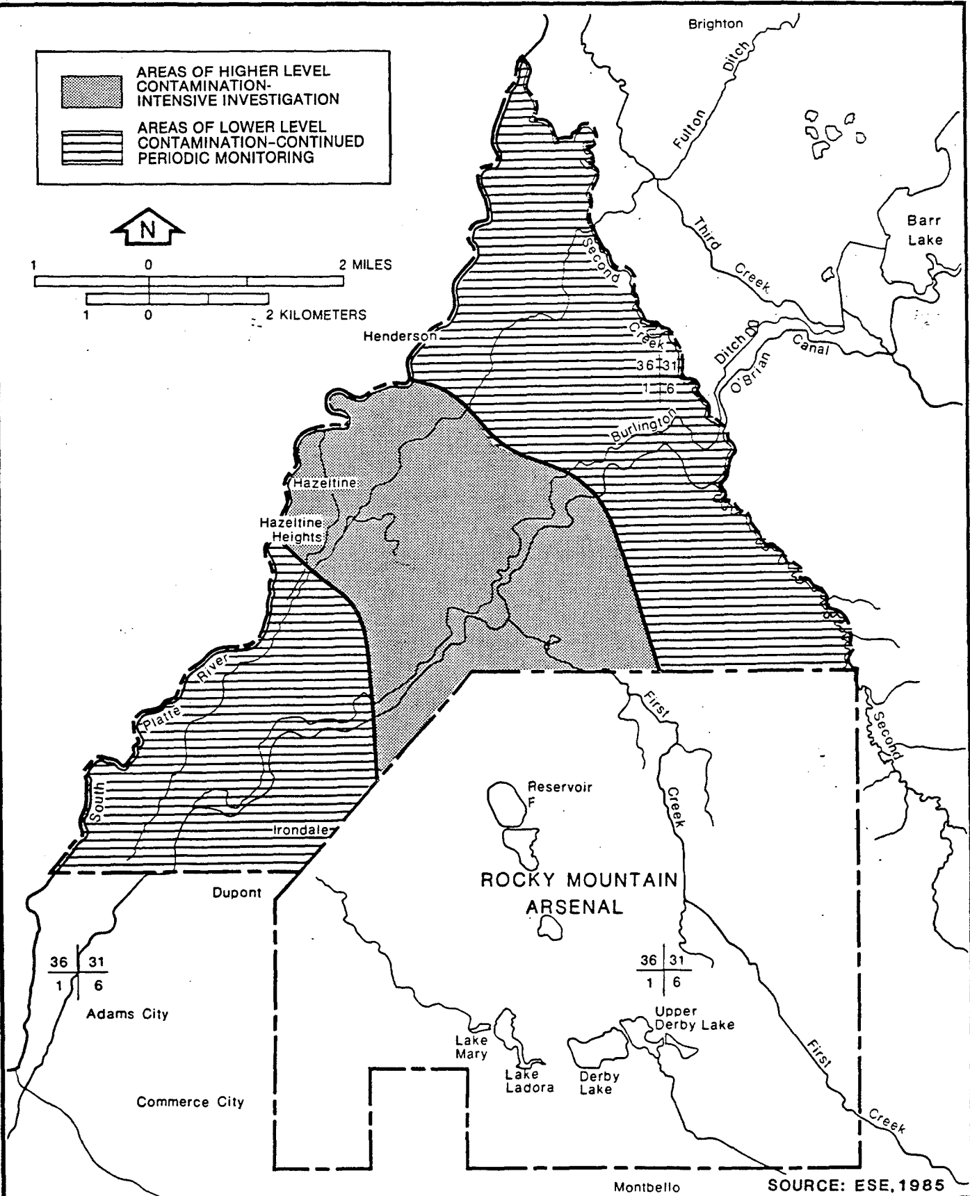
Figure 1.1-2 RELATIVE CONTAMINANT LEVELS STUDY AREA PHASE I
