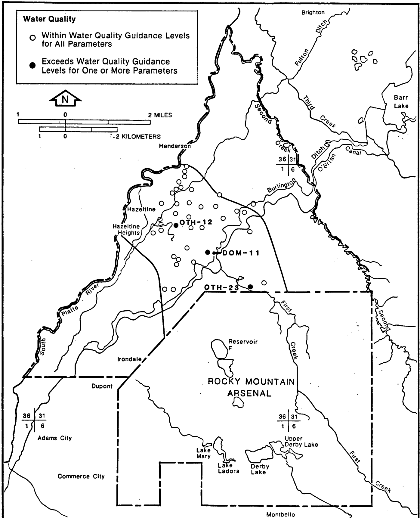
Figure 7.2-1 WATER QUALITY IN ALLUVIAL WELLS RMA CONSUMPTIVE USE PHASE II PROGRAM SEPTEMBER-OCTOBER 1985 SOURCE: ESE, 1986
