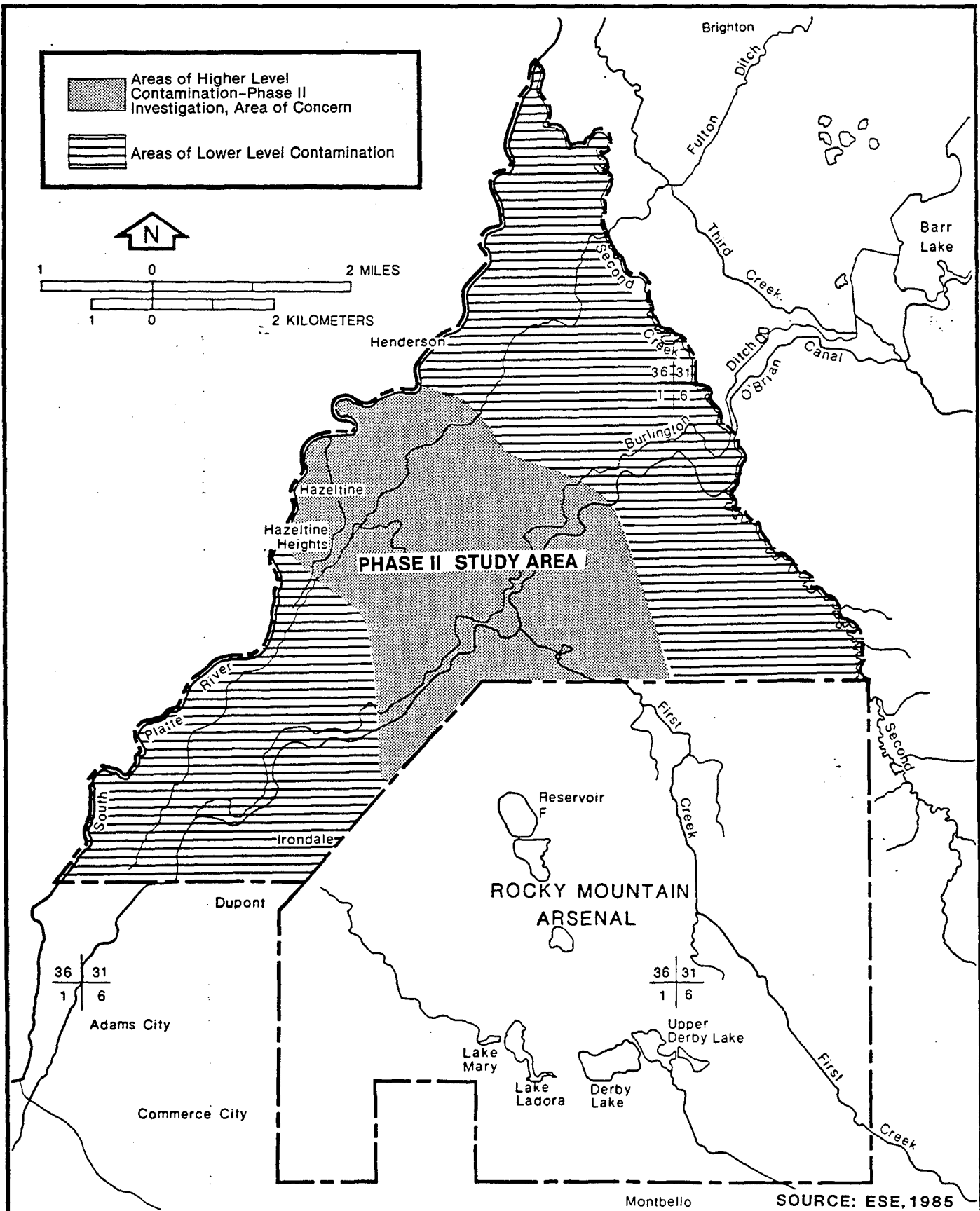
Figure 2.0-1 CONTAMINATED AREAS OFFPOST OF RMA
