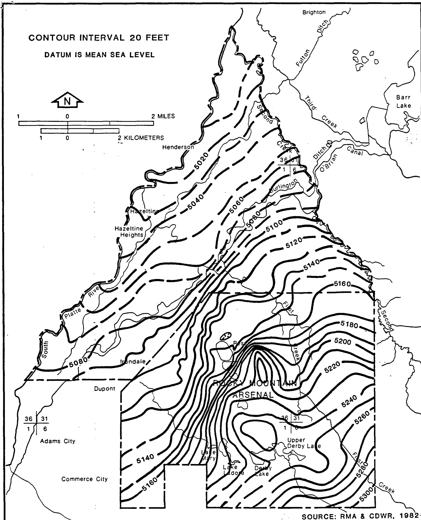
Figure 1.5-4 WATER TABLE CONTOUR MAP OF STUDY AREA
