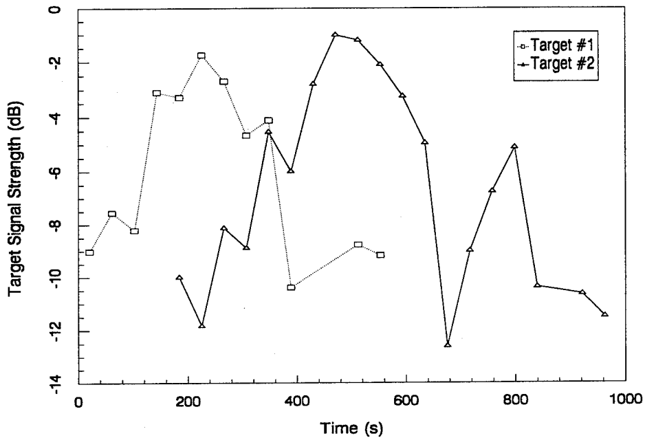
Figure 18 Signal Strengths of Tareget #1 and #2 in DT15
