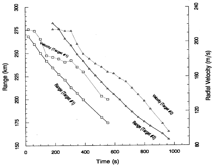
Figure 13 Ranges and Radial Velocities of Target #1 and #2 in DT15
