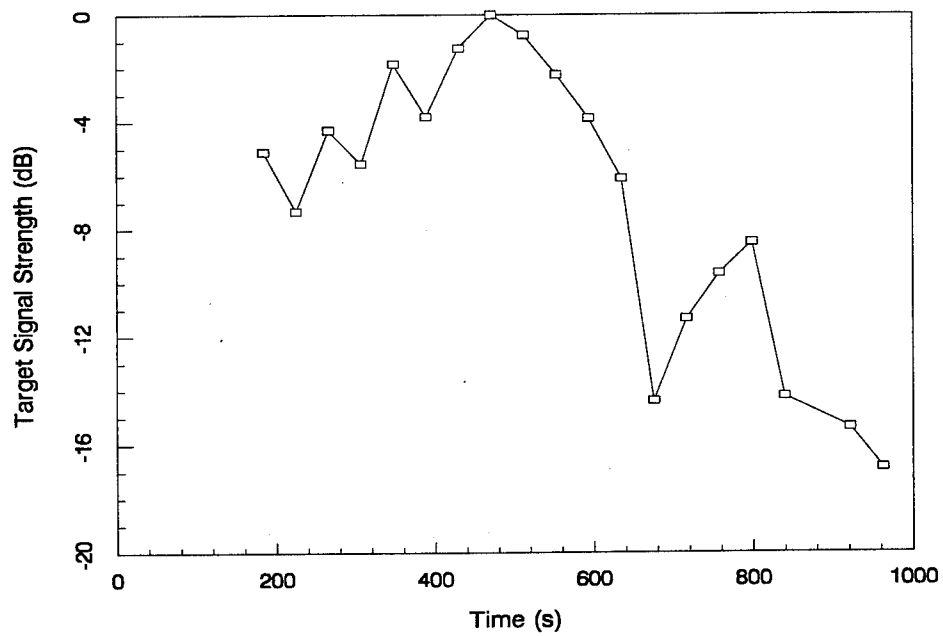
Figure 19 Range-Corrected Signal Strength of Target #2 in DT15 (Normalized to the peak value)
