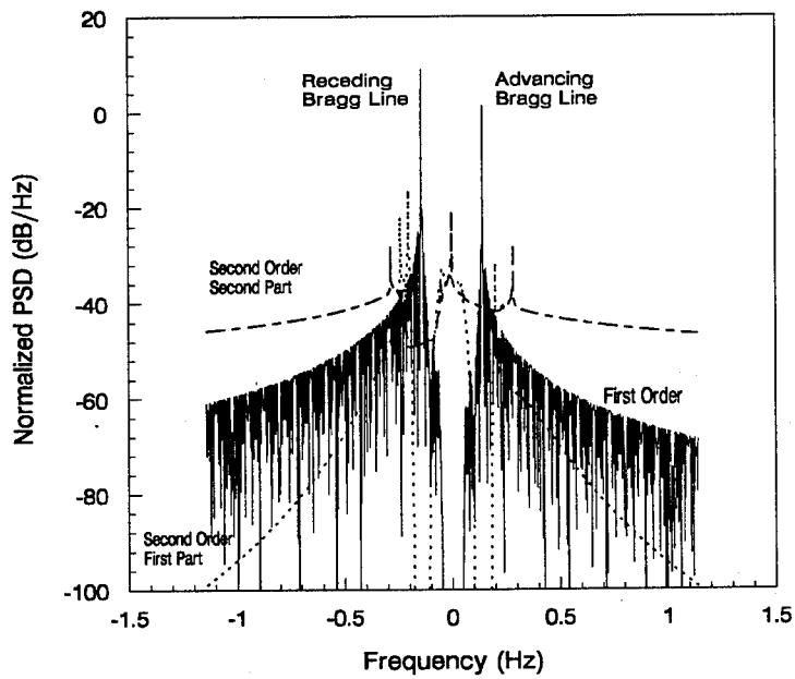
Figure 4 Theoretical Spectra of Sea Clutter from 1.95 MHz HFSWR under a Fully Developed Sea Condition
