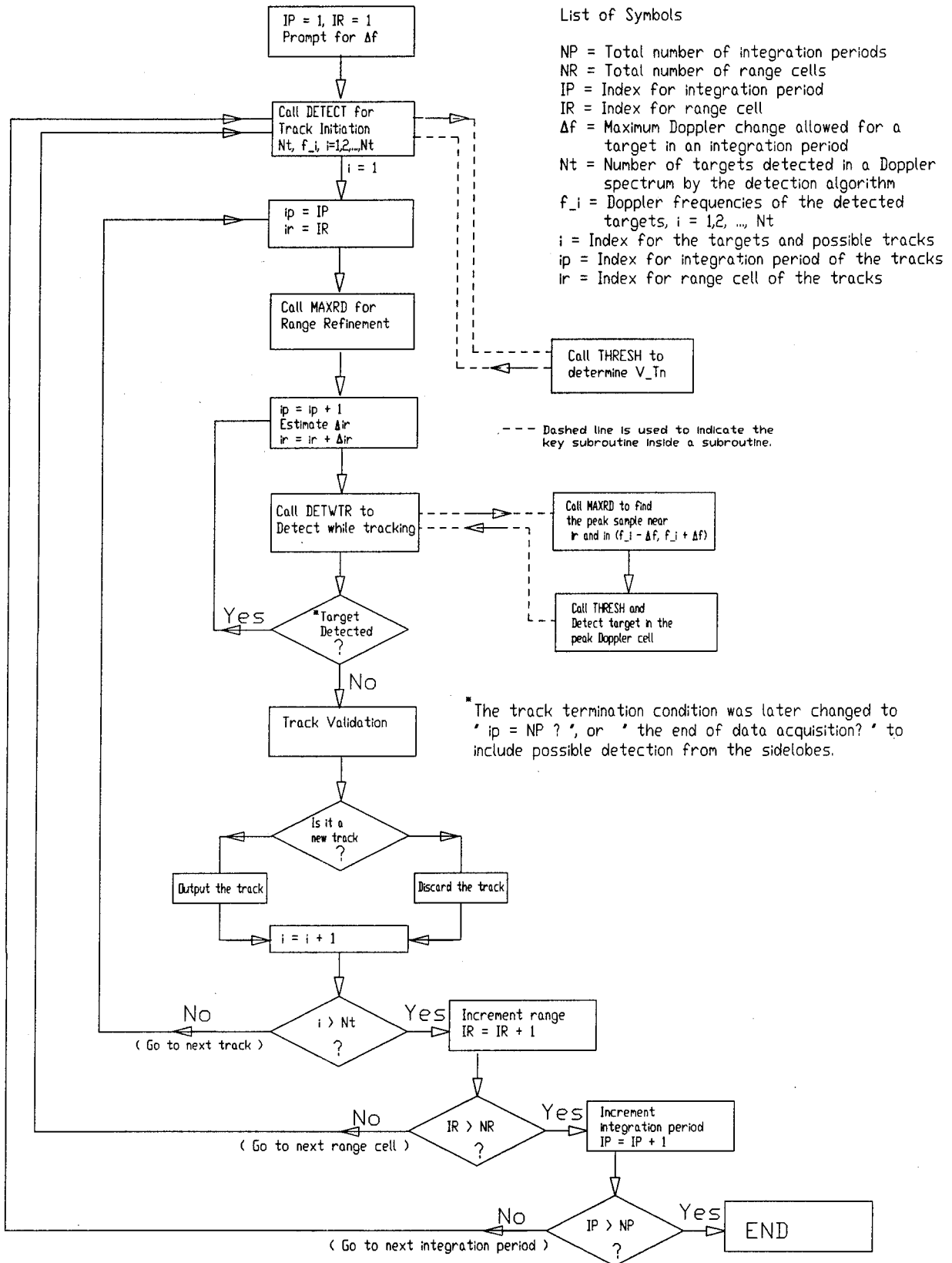
Figure 9 Block Diagram for Tracking Algorithm
