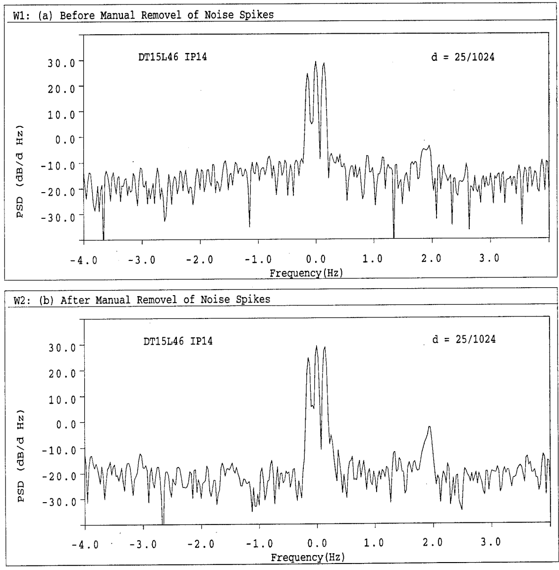
Figure 22 A Doppler Spectrum of DT15 before and after Removal of Noise Spikes
