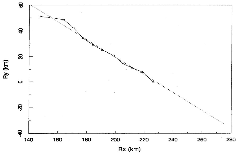
Figure 20 Track of Target #2 in DT15 in the Rectangular Coordinates
