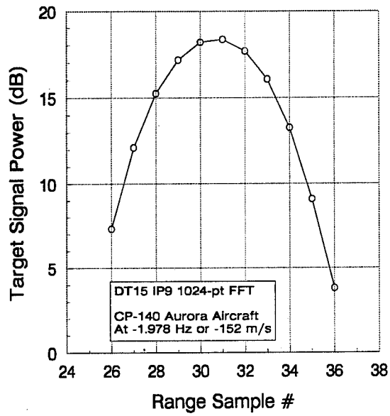
Figure 3 Interpolation of Target Signal Across Range
