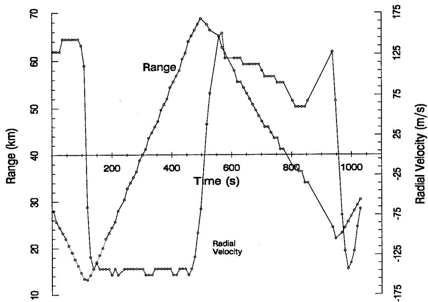
Figure 12 Range and Radial Velocity of the Aurora Aircraft in DT15
