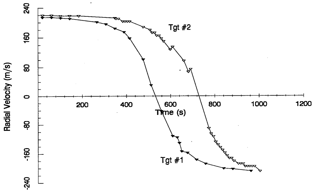
Figure 15 Radial Velocities of Target #1 and #2 in DT39
