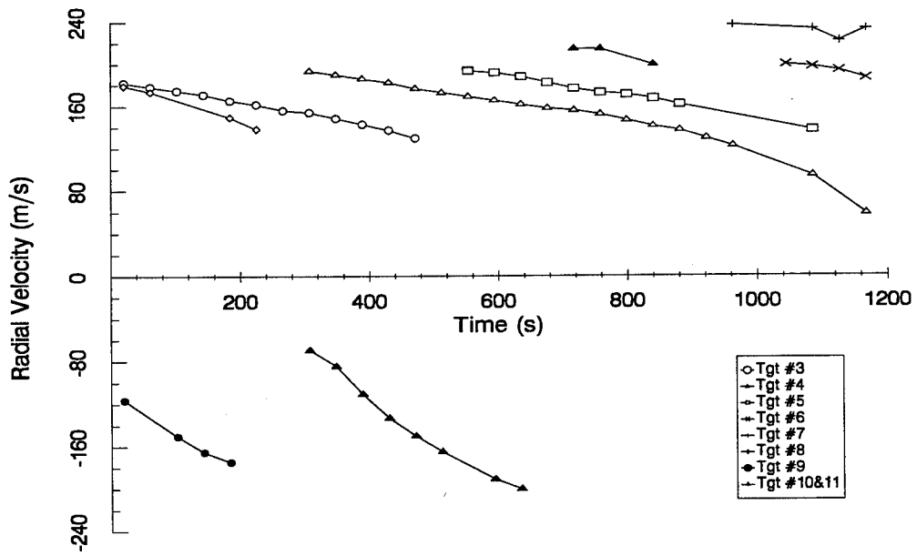
Figure 16 Radial Velocities of the Other Aircraft Targets in DT39
