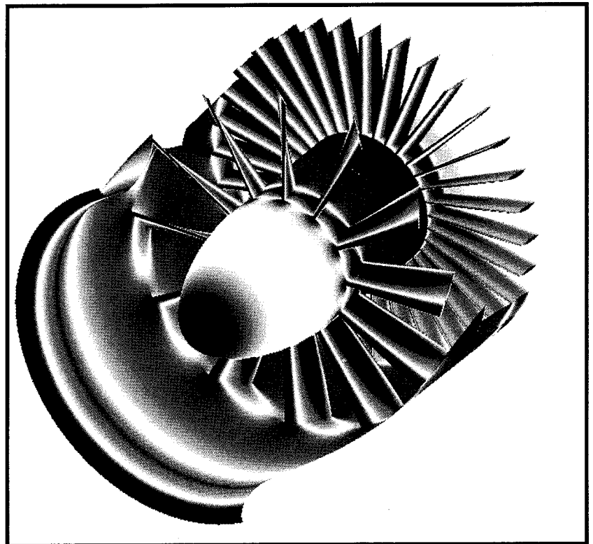
Pressure Field in a NASA 1.15 Pressure Ratio Fan
