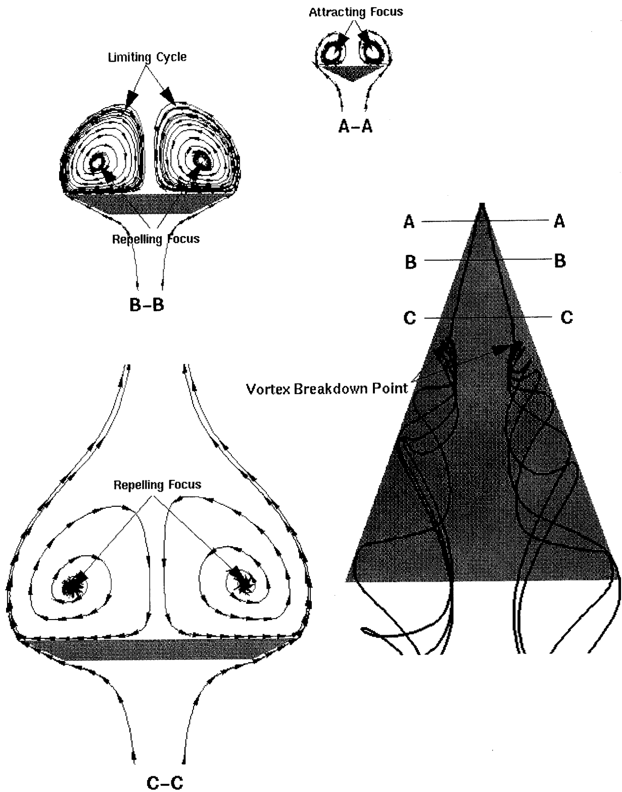
Figure 2.16 Vortical Flow Over a 70° Delta Wing at \alpha=40^\circ , Re=1.5 \times 10^6
