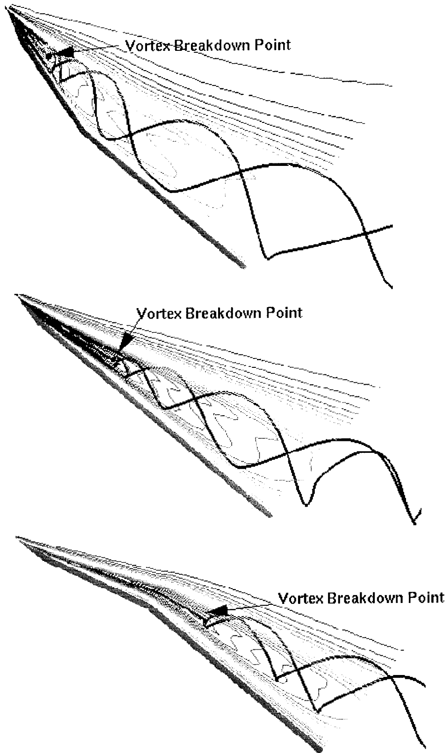
Figure 2.12 Distribution of Total Pressure Across the Plane of Vortex Core Over a 70^\circ Delta Wing at \alpha=40^\circ
