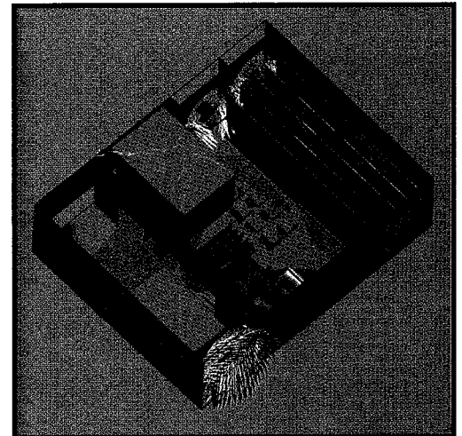
Fan Induced Cooling Flow with Conjugate Heat Transfer in a Computer Box
