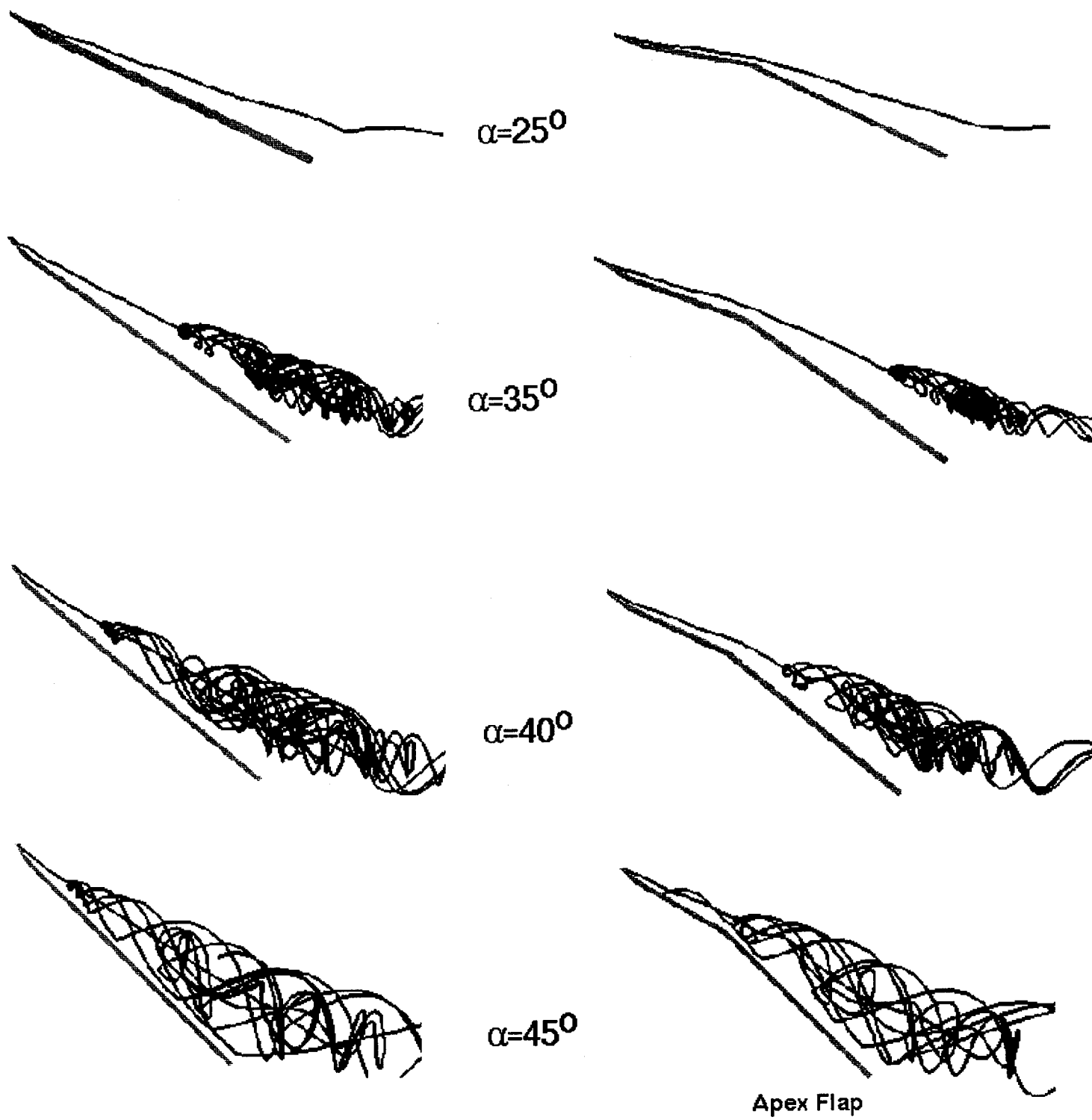
Figure 2.13 Effect of Apex Flap With 15^\circ Downward Deflection on the Vortex Breakdown Over a 70^\circ Delta Wing at Several Angles of Attack
