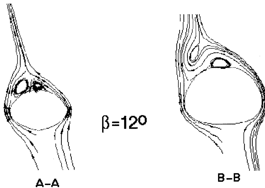
Figure 3.6 Cross Flow Topology Over Standard F-16 Forebody at \alpha=40^\circ .
