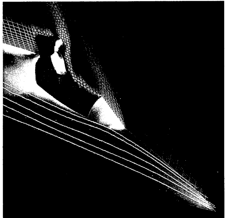
Unstructured (above), Hybrid Unstructured/Structured (below) Grid Model of Pilot Ejection from an F16 (Simulation using CFD-FASTRAN, CFDRC's High Accuracy Compressible Flow Solver).
