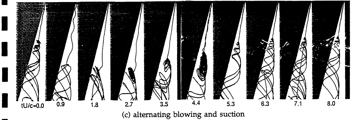
Figure 2-9. Computational Flow Visualization of Vortex Breakdown After Onset of Steady (a) Suction (b) Blowing and (c) Alternating Blowing and Suction Along the Half Length of the Leading Edge at tU/c = 0.0 and Abrupt Cessation at tU/c = 3.5
