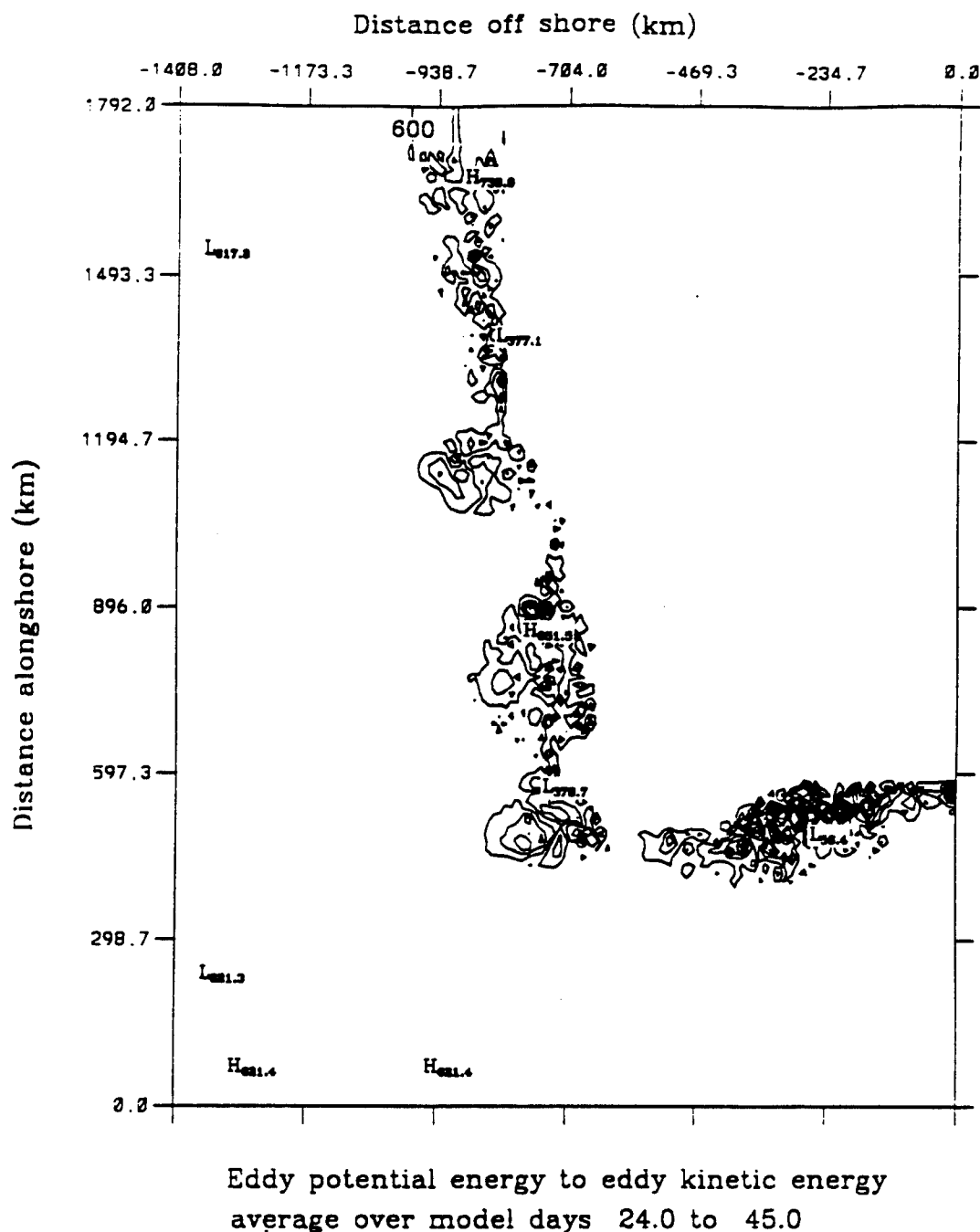
Figure 4.18b Experiment 4: Energy transfers of eddy potential to eddy kinetic energy (i.e., baroclinic energy transfer) for model days 24 to 45. The contour interval is 1 \text{ ergs cm}^{-3} \text{ s}^{-1} .
