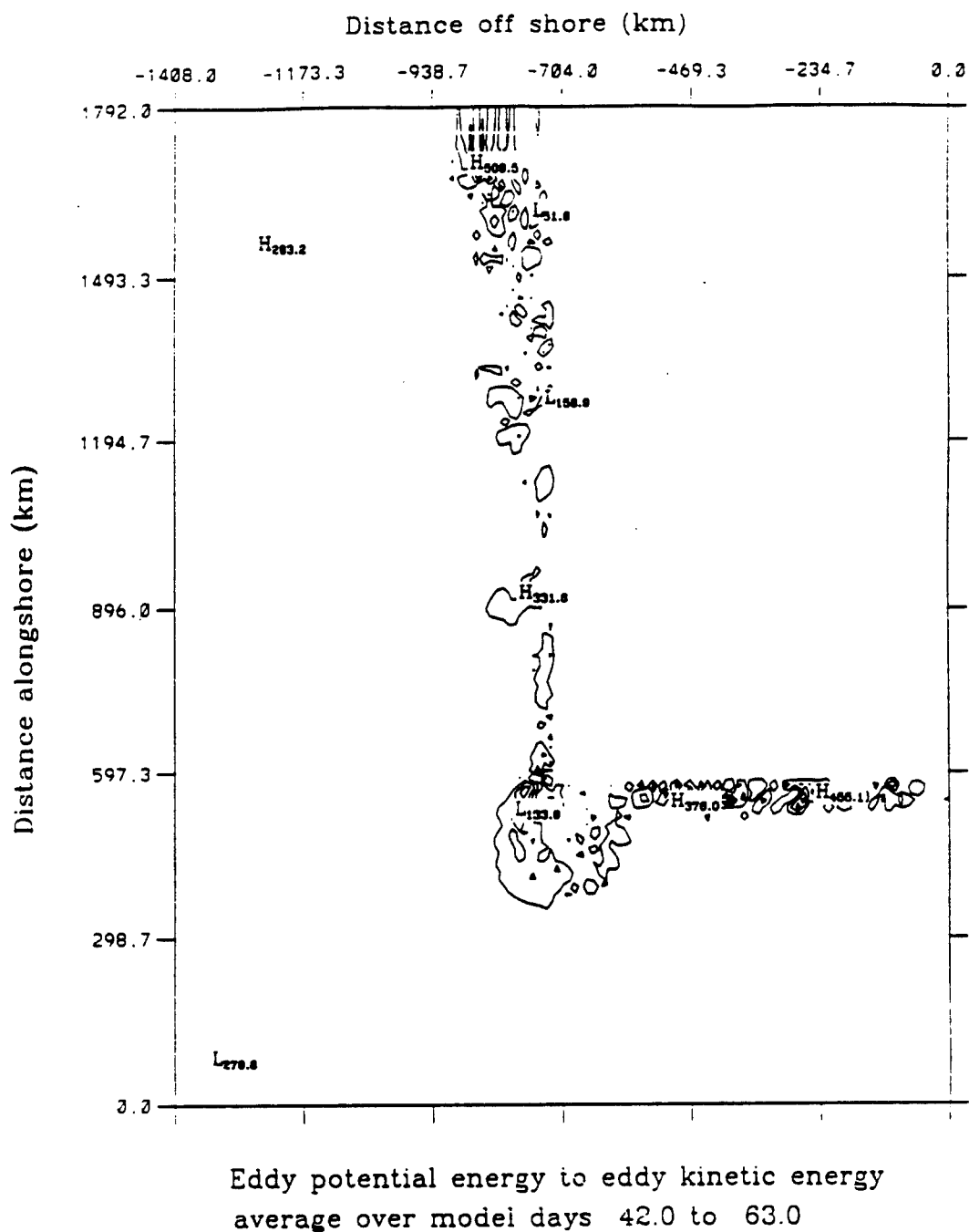
Figure 4.13b Experiment 3: Energy transfers of eddy potential to eddy kinetic energy (i.e., baroclinic energy transfer) for model days 42 to 63. The contour interval is 1 \text{ ergs cm}^{-3} \text{ s}^{-1} .
