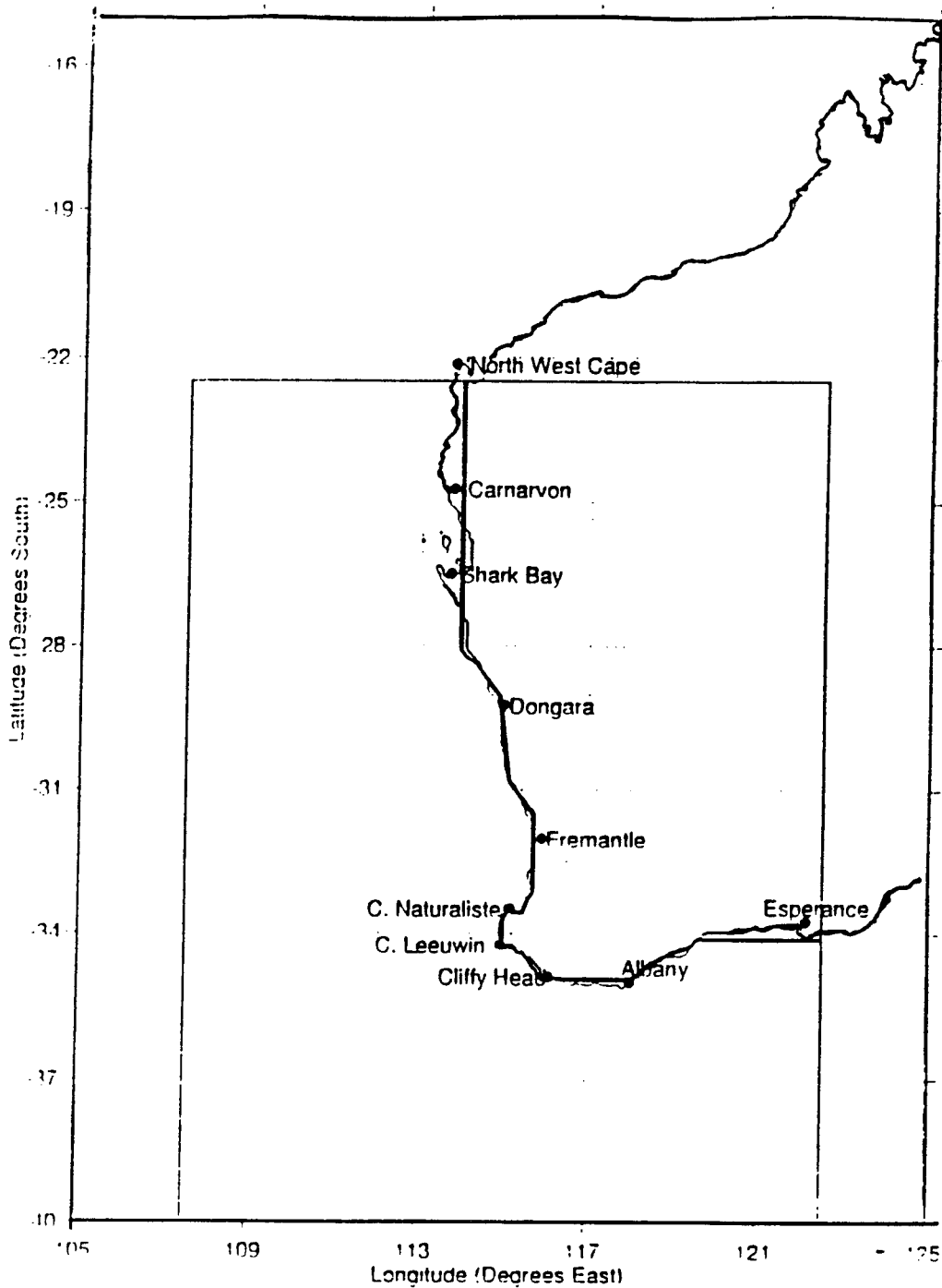
Figure 3.2: The "irregular coastline" (a second order model simulation) features the general characteristics and irregularities (e.g., coastal indentation south of Shark Bay, Dongara, Fremantle, Clifly Head, and Albany) along the western and southern coast of Australia (including a realistic representation of Cape Leeuwin).
