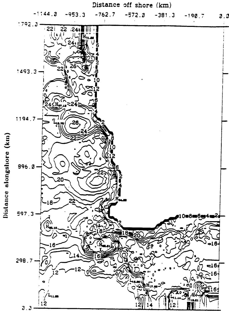
Temperature contour at model day 150.0
