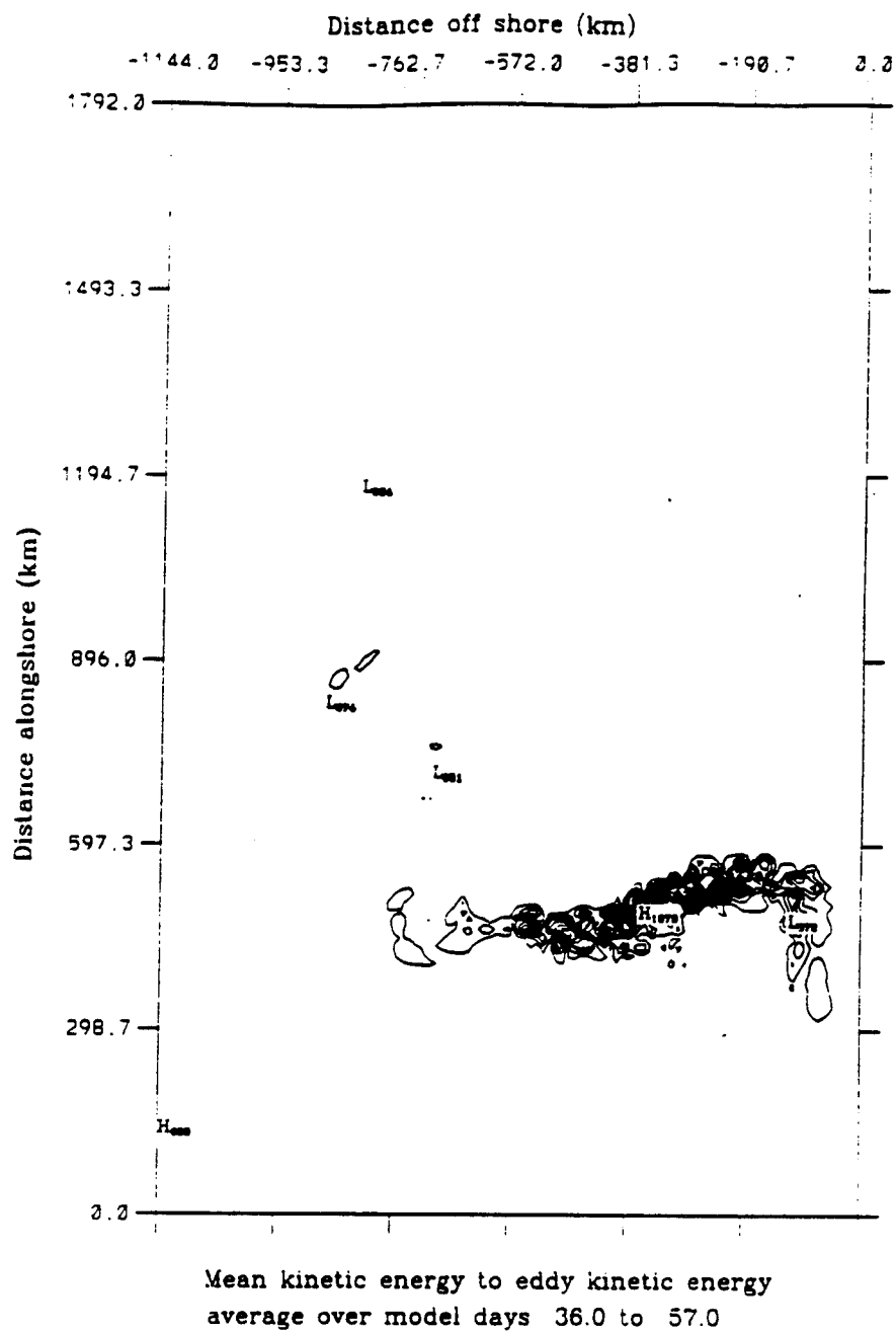
Figure 4.23a Experiment 5: Energy transfers of mean to eddy kinetic energy (i.e., barotropic energy transfer) for model days 36 to 57. The contour interval is 1 ergs cm -3 s -1 .
