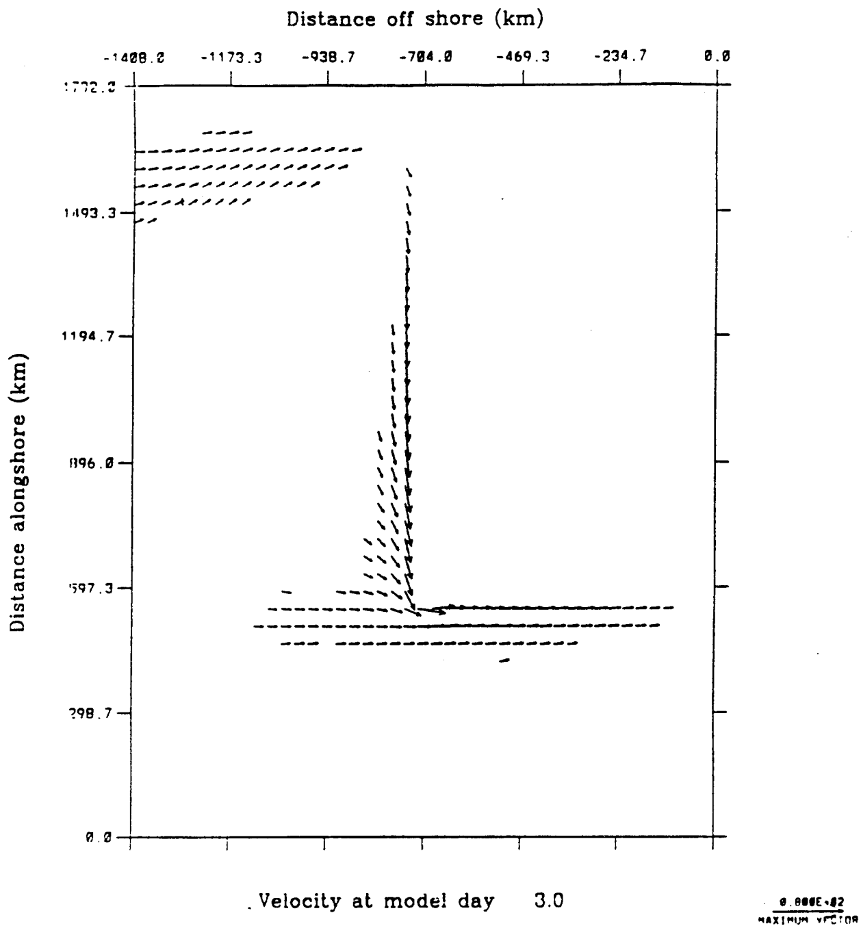
Figure 4.1a Experiment 1: Surface velocity vectors at day 3. To avoid clutter, velocity vectors are plotted at every third grid point in both the cross-shore and alongshore direction, and velocities less than 5 \text{ cm s}^{-1} are not plotted.
