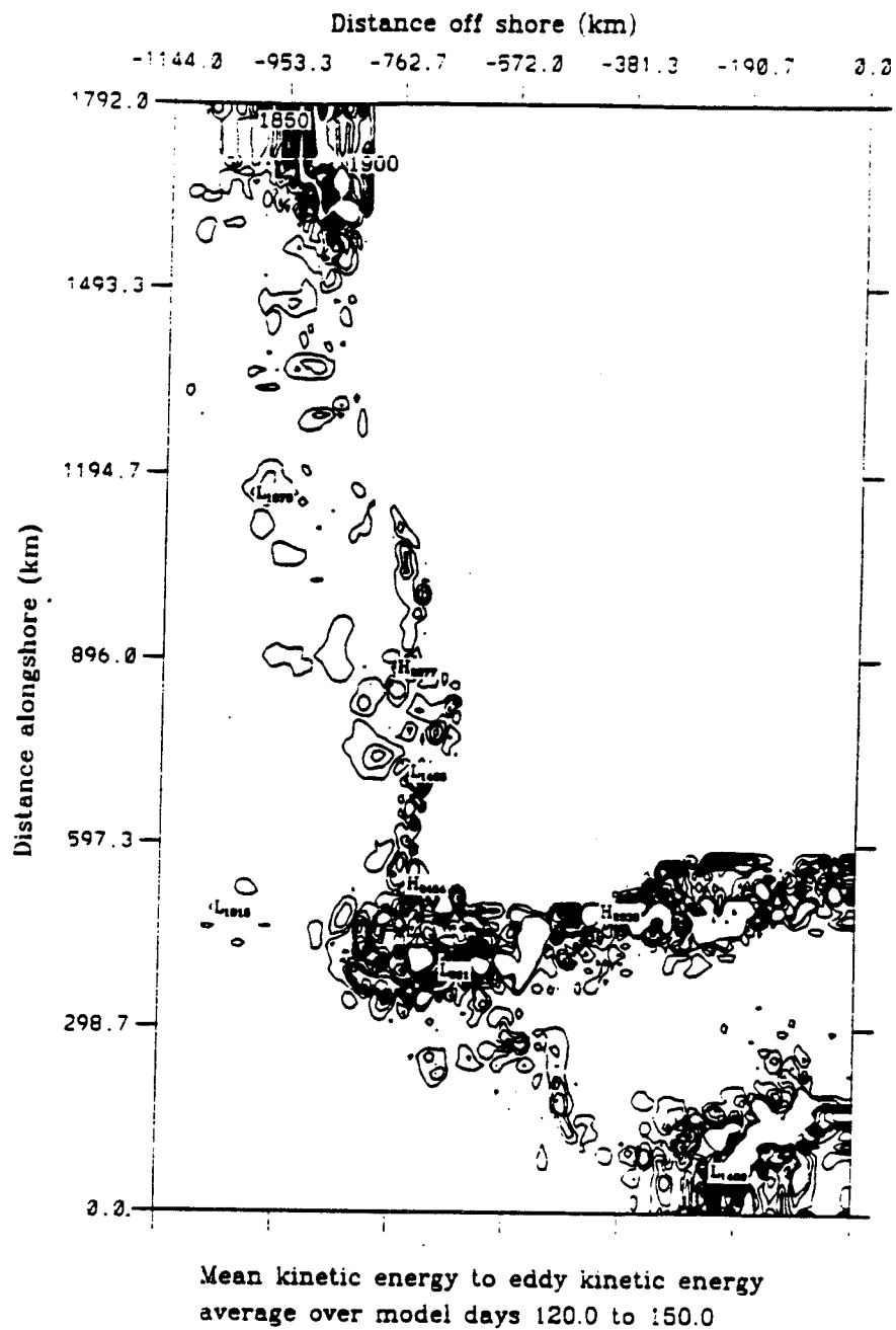
Figure 4.24a Experiment 5: Energy transfers of mean to eddy kinetic energy (i.e., barotropic energy transfer) for model days 120 to 150. The contour interval is 1 ergs cm -3 s -1 .
