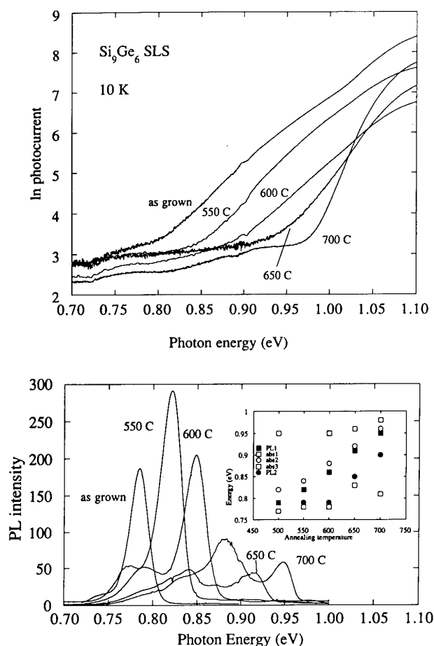
Figure 3. Photocurrent spectra (top) and PL spectra (bottom) for a \text{Si}_9\text{Ge}_6 SLS as a function of isochronal annealing at various temperatures. In the inset in the lower part the onset energies as determined from a fitting procedure from the photocurrent spectra are compared with various PL energies.
