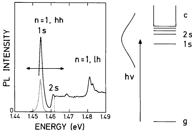
Figure 2. Photoluminescence excitation spectrum (full curve) and photoluminescence spectrum (dotted curve) of an \text{In}_{0.08}\text{Ga}_{0.92}\text{As}/\text{GaAs} multi quantum well sample at T = 5\text{ K} (left-hand side) and schematic representation of the excitation process using pulses of about 110 fs duration with the corresponding spectrum.
