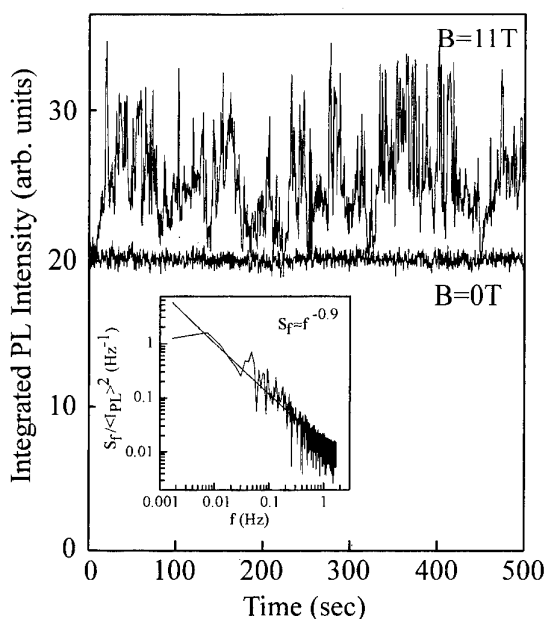
Figure 7. The time dependence of the PL signal in the indirect regime ( V_g = -0.5 V) at T = 350 mK for B_{\perp} = 11 T and at B = 0 . The excitation density for B = 0 is six times higher than for B_{\perp} = 11 T to get approximately the same signal level. Inset: power spectrum of the noise for B_{\perp} = 11 T.
