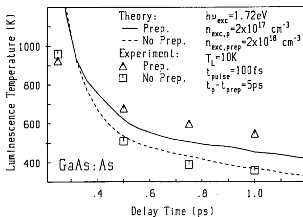
Figure 2. Plasma cooling with and without prepump.
