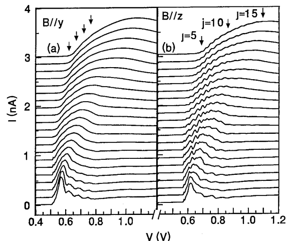
Figure 7. I(V) at T = 0.3 K in the presence of a magnetic field between B = 0 T (lowest curve) and B = 10 T (top curve) in 0.5 T steps. The field is oriented perpendicular to the current flow and either perpendicular (a) or parallel (b) to the axis of the quantum wire.
