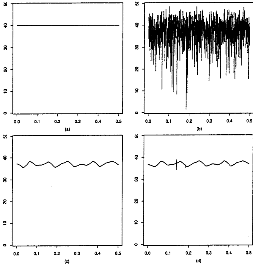
Figure 2: (a). log spectrum of a white noise signal, (b). log periodogram, (c). WaveShrink estimate based the new thresholding scheme, and (d). WaveShrink estimate based on Gaussian theory.
