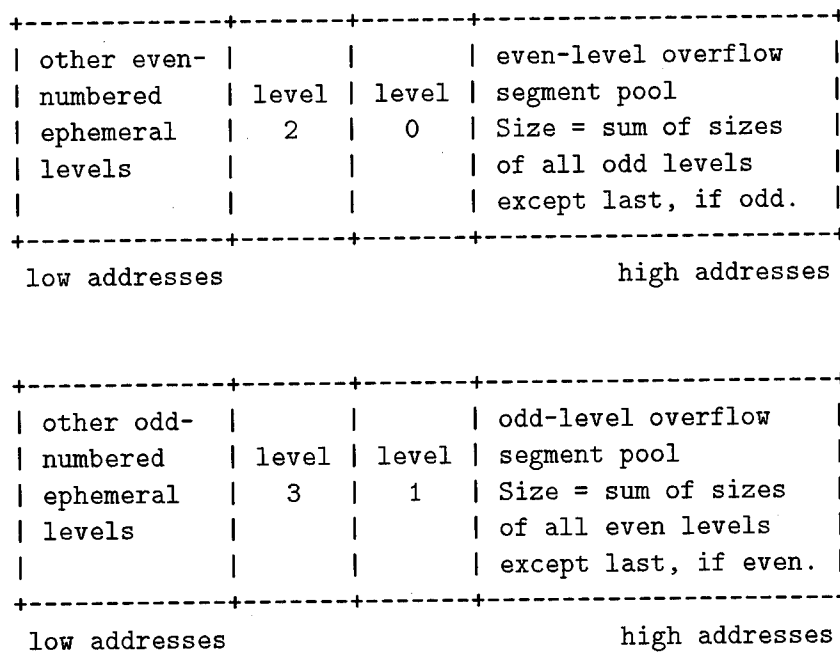
Figure 3: Layout of ephemeral spaces and overflow segment pools in Lucid Common LISP.
