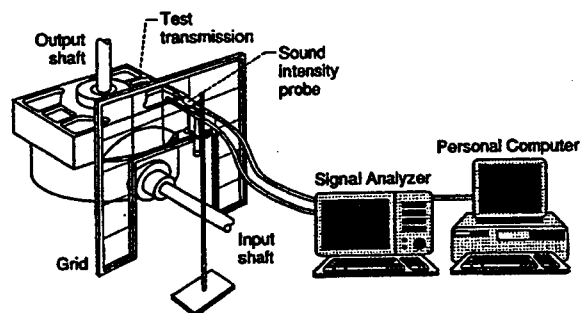
Fig. 4. Sound intensity measurement system.
