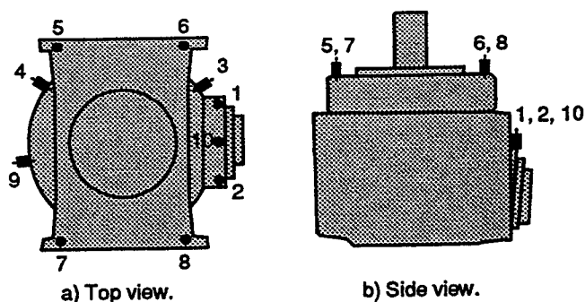
Fig. 5. Accelerometer locations of OH-58D transmission.
