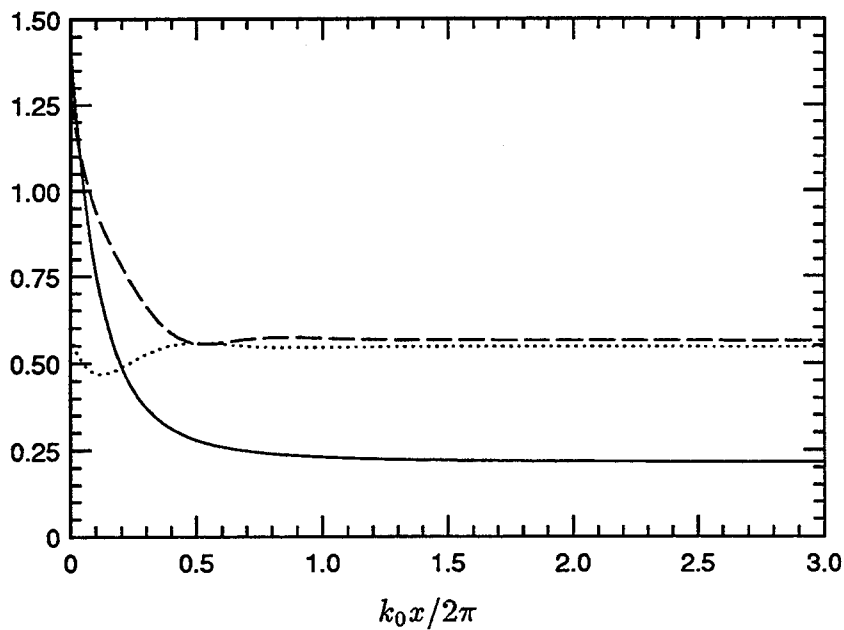
FIG. 18. The variation of thermodynamic fluctuations behind a Mach 1.5 shock wave. The incident fluctuations correspond to A_r = 0.58 and \phi_r = 0 . All three curves are normalized with \sqrt{q'_1}/U_1 . — ( p'_2/P_2 ), ---- ( \rho'_2/\bar{\rho}_2 ), ..... ( T'_2/\bar{T}_2 ).
