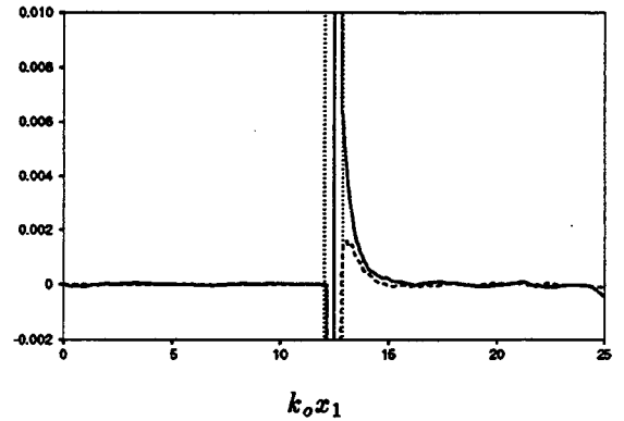
FIGURE 3(B). Evolutions of pressure-dilatation correlation and entropy-dilatation correlation for M_1 = 2.0 : — p' u_k'' / \gamma \bar{p} u_o k_o , ---- -s' u_k'' / c_p u_o k_o . Vertical lines denote the boundaries of shock intermittency.
