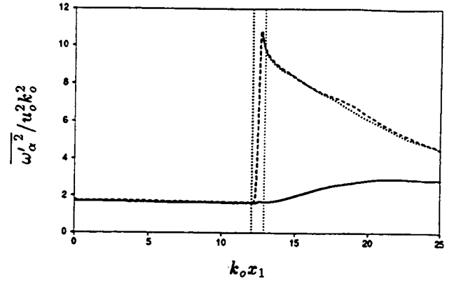
FIGURE 4(A). Evolution of the vorticity fluctuation variances with M_1 = 2.0 : — \overline{\omega'_1{}^2} , --- \overline{\omega'_2{}^2} , ..... \overline{\omega'_3{}^2} .
