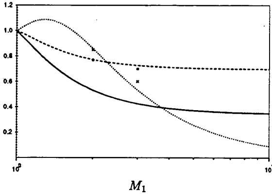
FIGURE 7(B). Change of Taylor microscales and dissipation length scale across the shock wave predicted by LIA. — \lambda_1 , --- \lambda_2 & \lambda_3 , ..... l_c . Symbols for DNS: • \lambda_2 , × l_c .
