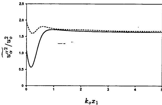
FIGURE 2(C). Evolution of velocity fluctuation variances behind the shock wave predicted by LIA ( M_1 = 2.0 ). — \overline{u_1''^2} , --- \overline{u_2''^2} & \overline{u_3''^2} .
