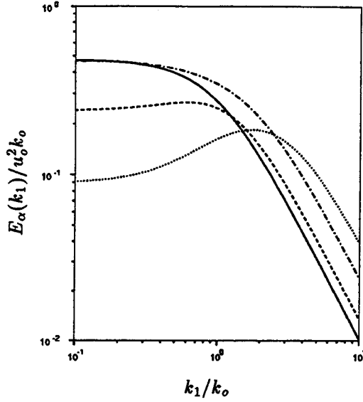
FIGURE 5(A). LIA prediction of the shock-normal direction (vs. k_1 ) one dimensional energy spectra change across the shock wave for M_1 = 2.0 : E_1 : — upstream, --- downstream, E_2 & E_3 : ..... upstream, ..... downstream.
