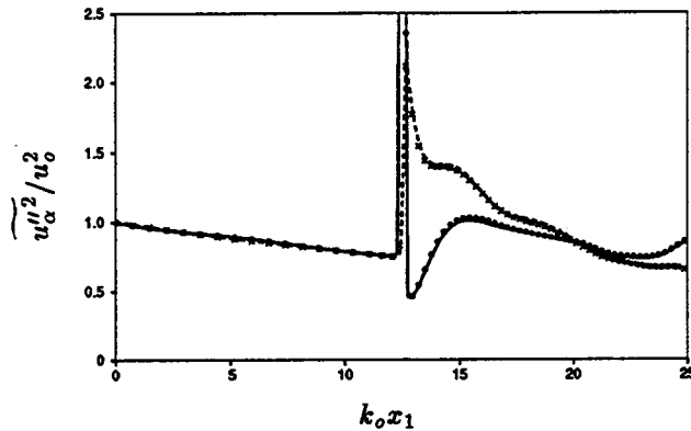
FIGURE 1. Evolution of the velocity fluctuation variances ( M_1 = 2.0 , M_t = 0.07 ): lines denote results from shock resolving simulation and symbols from shock capturing simulation. —, •: R_{11} , ----, ×: R_{22} .
