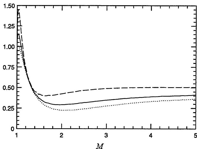
FIG. B.12. Far-field kinetic energy as a function of Mach number. All components are normalized with the incident energy and M^2 . ---- (\overline{u^2}/M^2 \overline{u_0^2}) , ..... (\overline{v^2}/M^2 \overline{v_0^2} = \overline{w^2}/M^2 \overline{w_0^2}) , — (\overline{q^2}/M^2 \overline{q_0^2}) . The three curves asymptote to 0.49, 0.40 and 0.43 respectively ( \gamma = 1.4 ).
