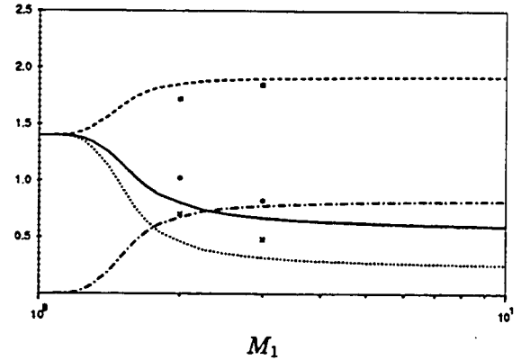
FIGURE 11. Downstream polytropic exponents and entropy fluctuation contribution predicted by LIA. — n_{pp} , ---- n_{pT} , ..... c_{pT} , — Entropy fluctuation contribution. Symbols for DNS: • n_{pp} , □ n_{pT} , × c_{pT} .
