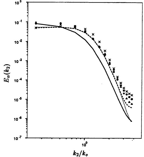
FIGURE 6. Changes in one dimensional spectra across the shock wave which is at k_o x_s = 12.29 : lines for upstream spectra at k_o x_1 = 10.59 , and symbols for downstream spectra at k_o x_1 = 13.68 . —, •: E_2(k_2) , ---, x: E_1(k_2) , ..... , Δ: E_3(k_2) .
