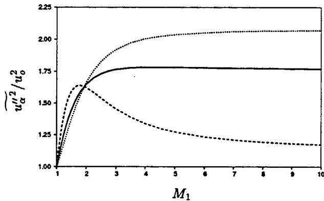
FIGURE 2(B). Amplification of velocity fluctuation variances across the shock wave predicted by LIA far away from the shock. — q^2/q_o^2 , --- \overline{u_1''^2} , ..... \overline{u_2''^2} & \overline{u_3''^2} .
