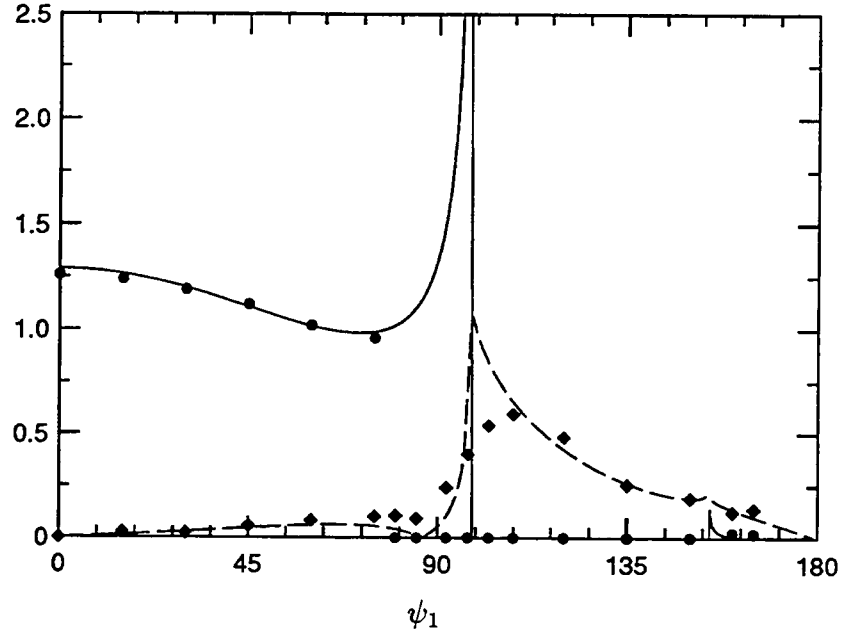
FIG. B.2. Comparison of the predictions of the linear analysis to computed results. The lines are values obtained from analysis while the symbols represent computed values. All quantities are normalized by p_1/P_1 . — (\theta_2/\theta_1) , ---- (\omega_2/\theta_1) . \theta_2 and \omega_2 denote the rms dilatation and vorticity behind the shock wave respectively.
