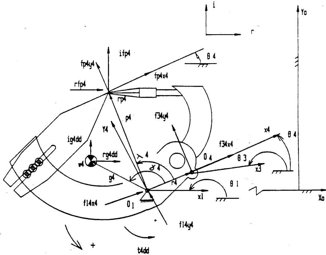
Figure A.10: Reaction Forces on Link 4
