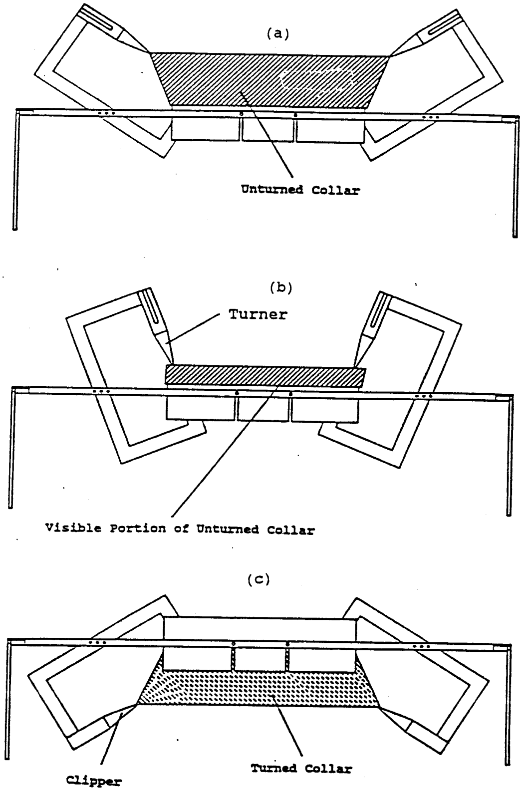
Figure 2.15: Pivot Turning Concept
