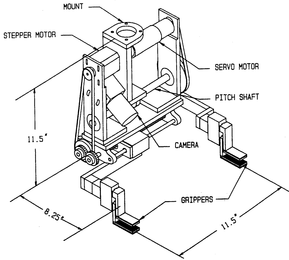
Figure 3. Collar-handling End-effector
