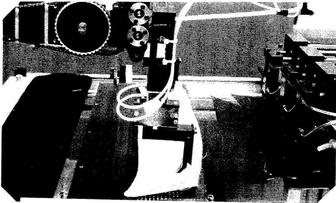
(b) Pressing device loaded with turned collar
