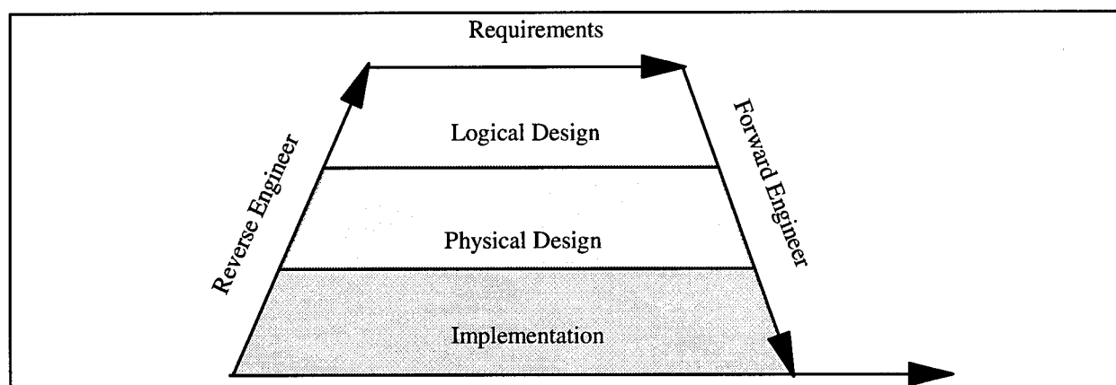
Figure 2. Software Reengineering and Levels of Information
