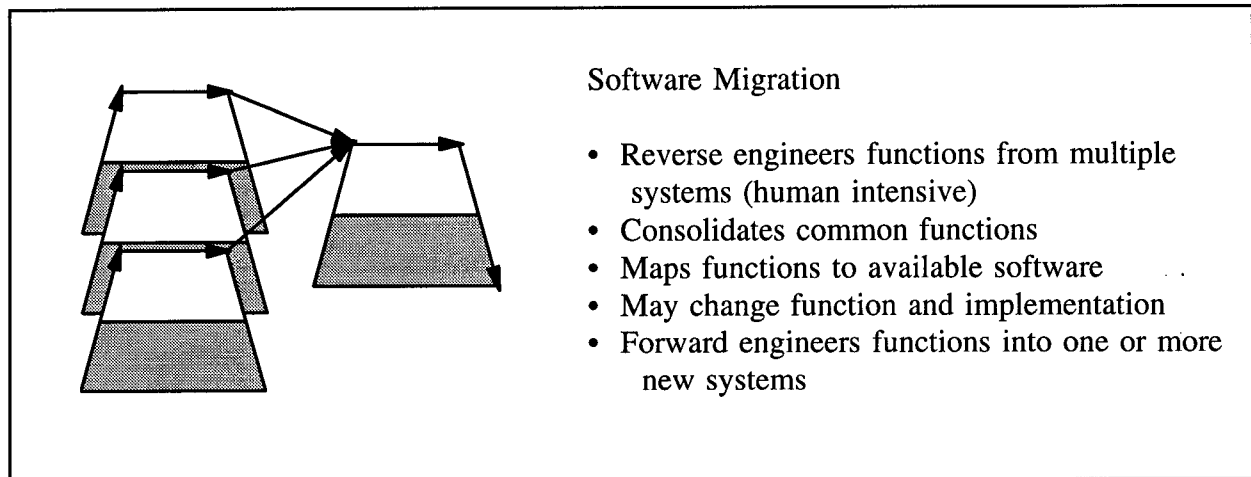
Figure 9. Software Migration
