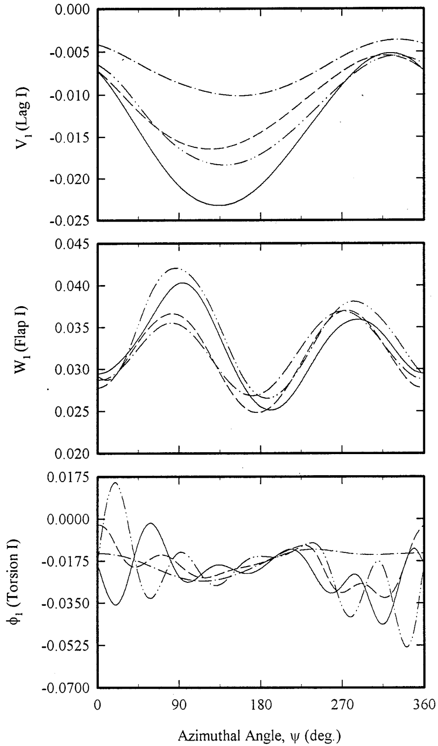
Figure 4: Effects of Aerodynamic Modeling on Periodic Responses for \mu = 0.3 and C_T/\sigma_s = 0.1 . (concluded in the next page)
