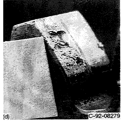
Figure 3.—(a) Heavy pitting on two teeth in Run 1 at 131 hr into run. (b) Example of spalling at end of Run 1. (c) Example of Run 2 moderate pitting. (d) Example of Run 3 heavy pitting.
