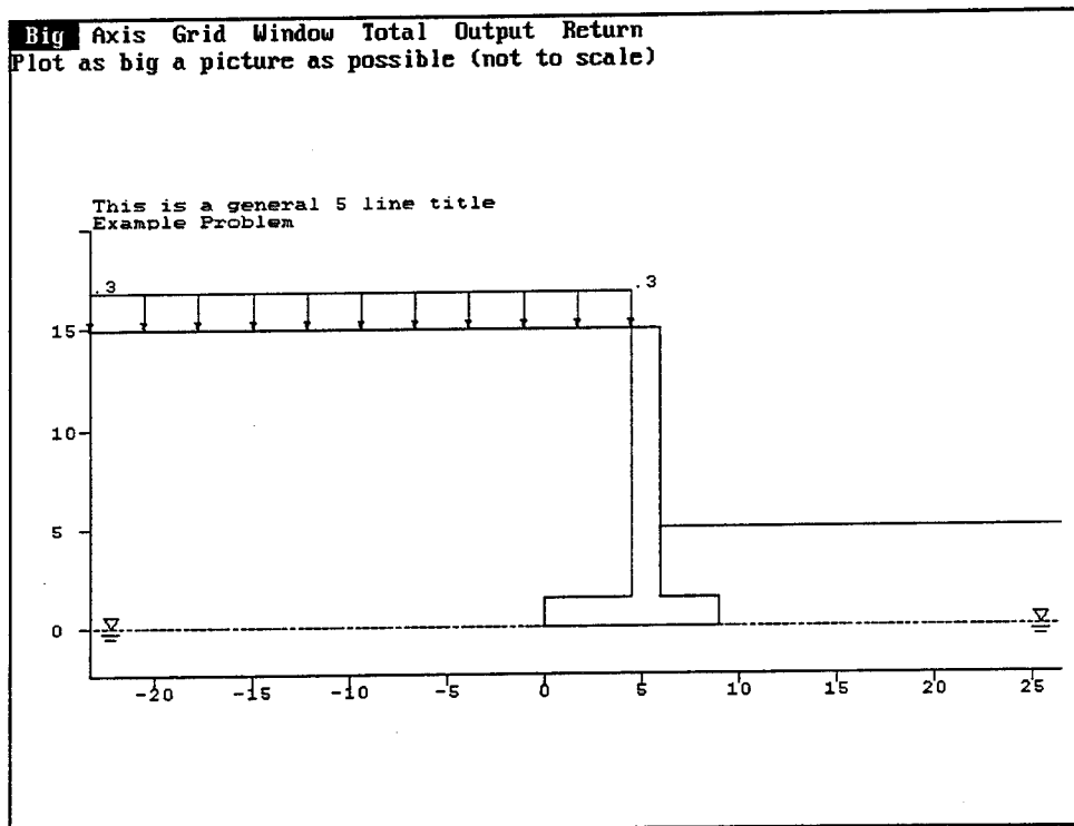
Figure 21. Input data plot
