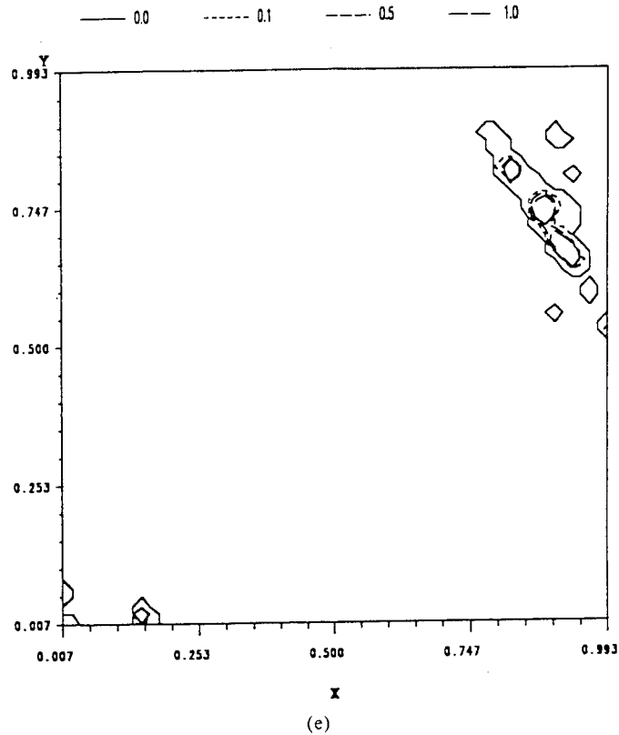
Fig. 4. (e) \gamma_{\text{avg}} = 0.07755 .
