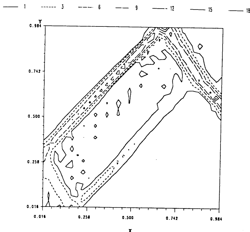
Fig. 10. (c) \gamma_{avg} = 0.10755 .
