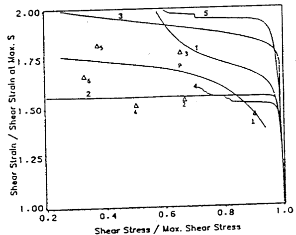
FIG 3. Plot of the normalized shear strain vs the normalized shear stress during the time shear stress is dropping with increasing strain. See FIG 2 for legends of curves.
