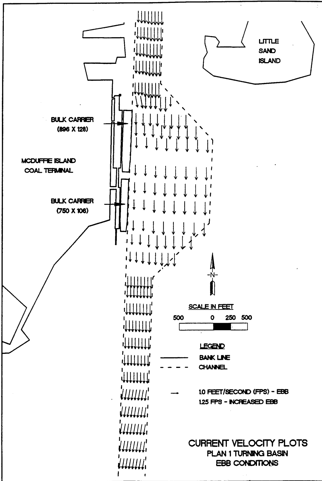
Figure 7. Plan 1 currents - Ebb tide
