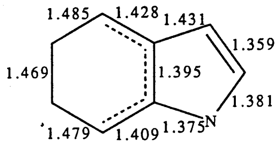
MC Geometry and Schematic Bonding
