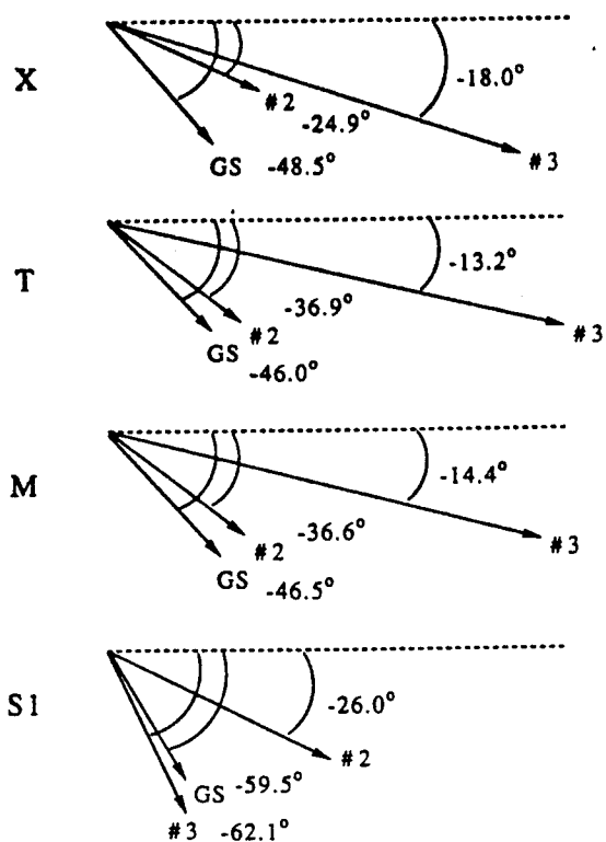
Figure 2. Transition dipole orientations relative to the indole long axis for excitation of both excited states from the ground state.
