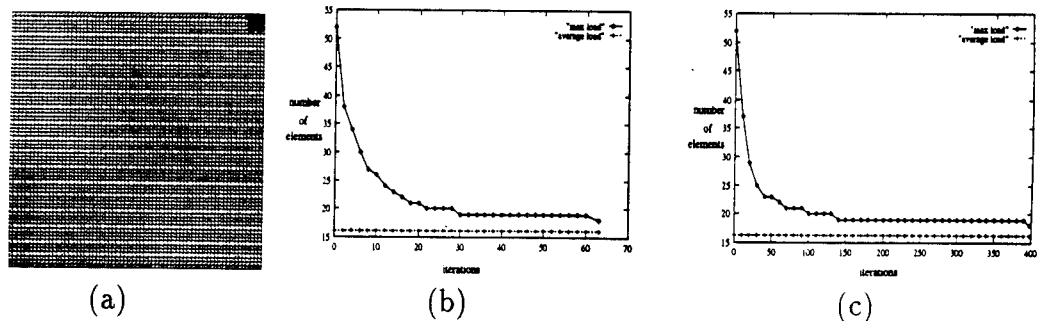
Figure 10: (a) Test mesh for square2 and square3 of Example 3.1, (b) and (c) corresponding convergence histories.
