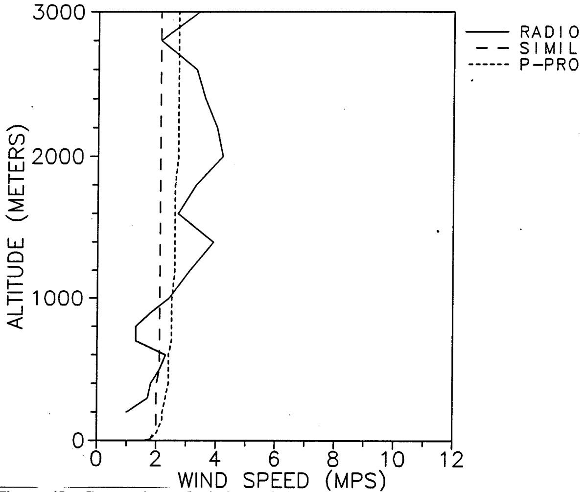
Figure 48. Comparison of wind speed data collected by a radiosonde launched July 22 at 1321 MDT with values estimated from tower measurements using Monin-Obukhov similarity and a p-profile fit.
