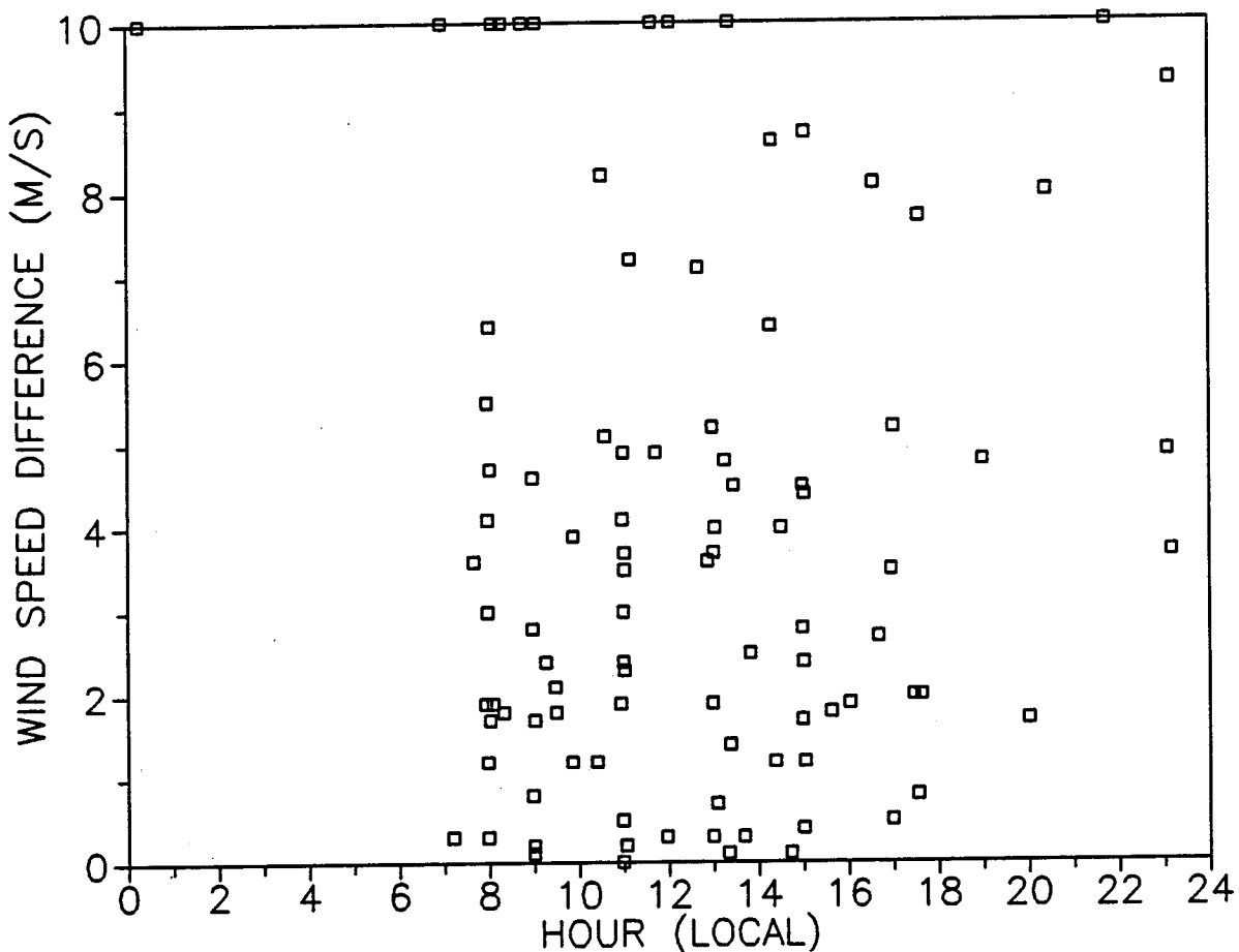
Figure 44. Absolute value of differences between radiosonde wind speed measurements and data estimated from tower measurements using p-profile.
