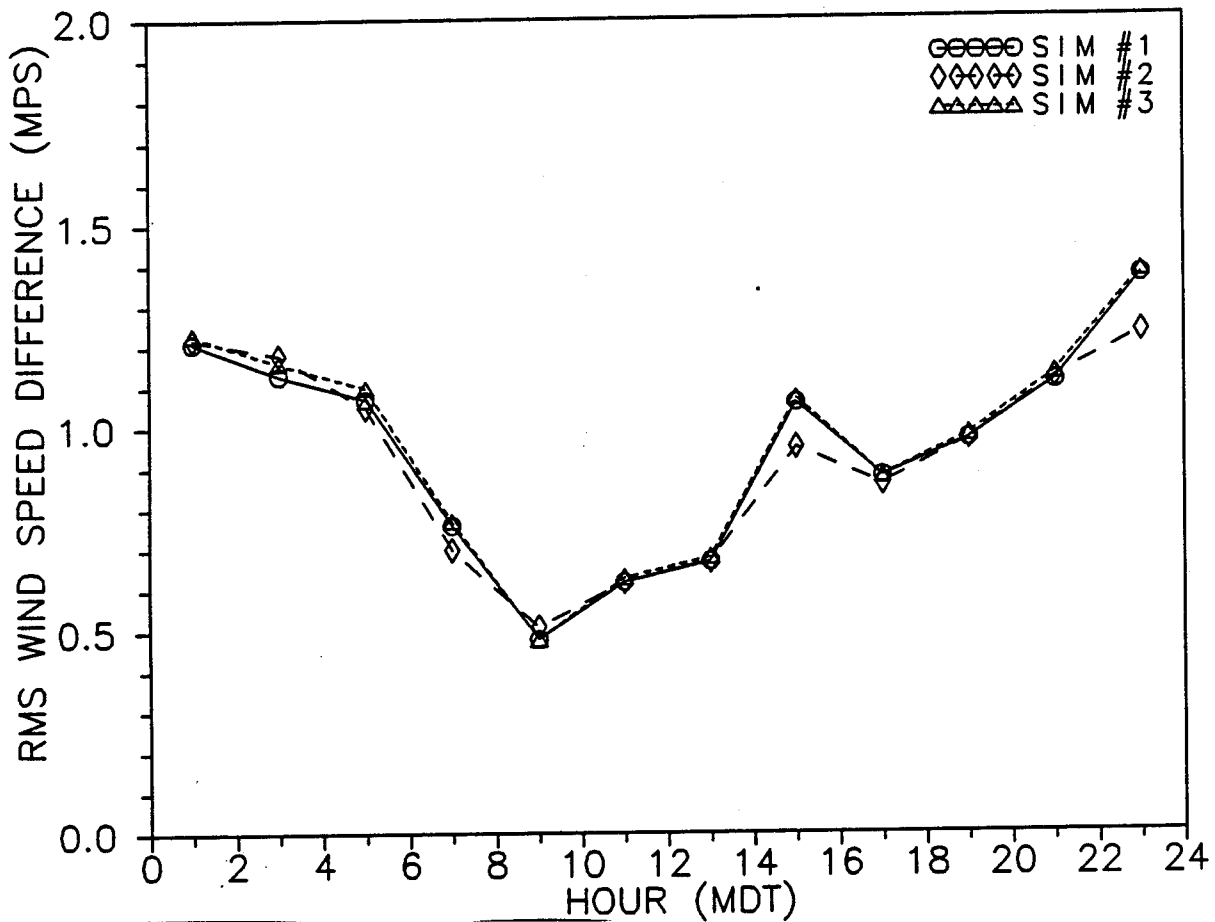
Figure 3. Rms differences between measured 30-m wind speeds and values estimated from 2- and 8-m measurements using three Monin-Obukhov similarity algorithms.
