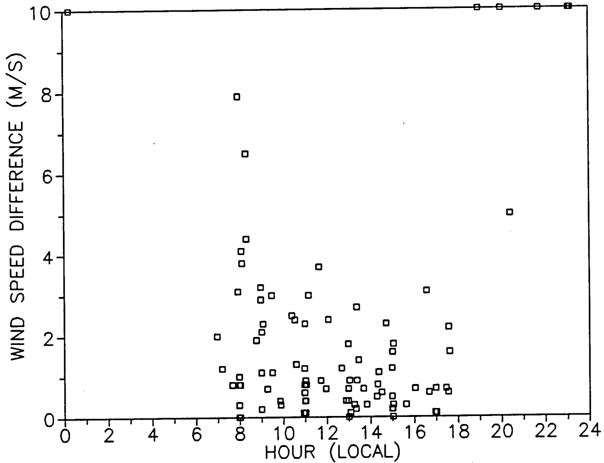
Figure 43. Absolute value of differences between radiosonde wind speed measurements and data estimated from tower measurements using Monin-Obukhov similarity.
