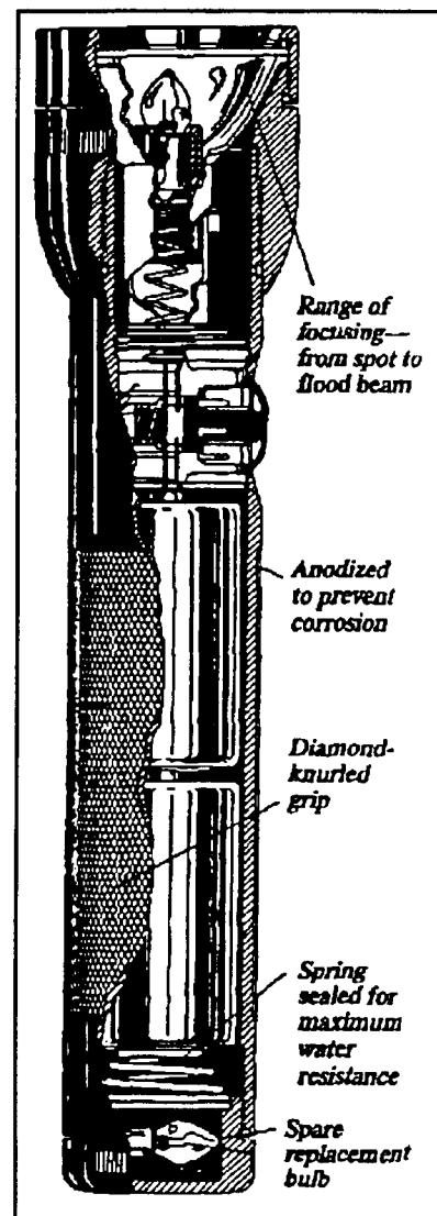
Figure 7 Mag-Lite (typical)
