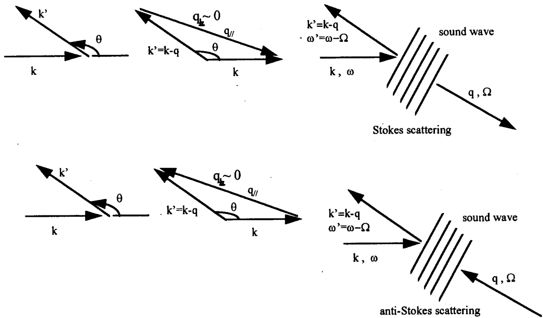
Fig.1 \Omega = 2|k|v \sin(\theta/2) = 2n\omega v/c \sin(\theta/2)
