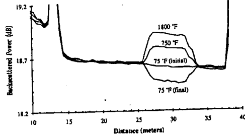
2. OTDR traces of 50/125µm graded index fiber showing irreversible change after cycling fiber to 1800°F. Note (in the lower trace) the return to the same level of scattering after the heated up region as before, indicating no extra attenuation associated with the irreversible change.
