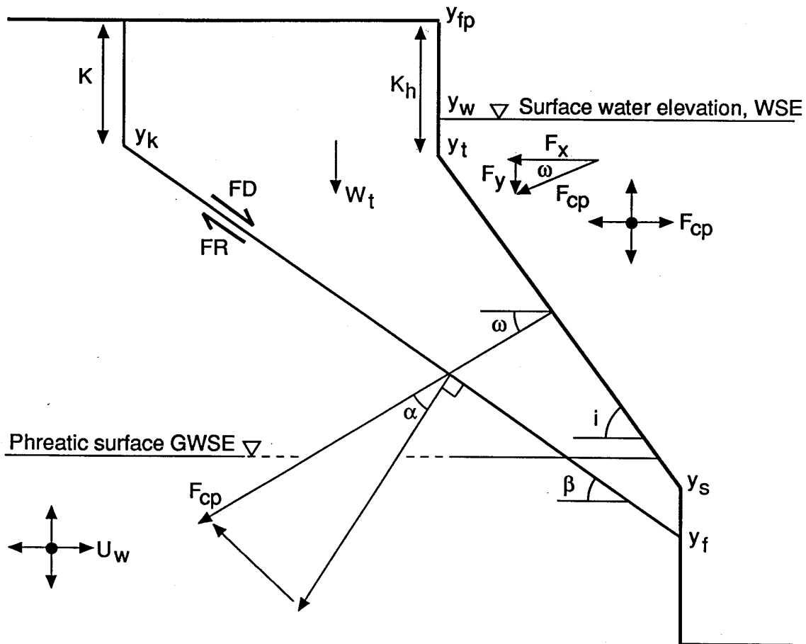
Figure 4 Bank stability analysis definition diagram
