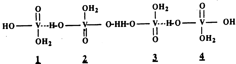
Proposed Assembly of Hydrolyzed Linear Polymers into Ribbon Structure. Individual Chains are numbered for identification.
