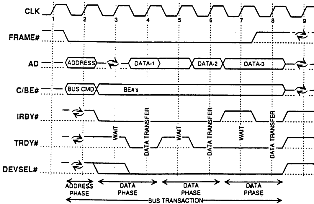
Basic Read Operation
