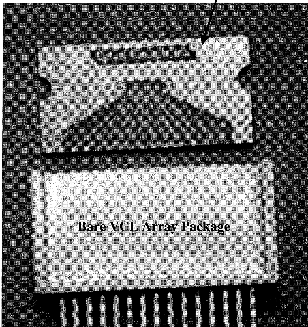
Close up of VCSEL Array Package
