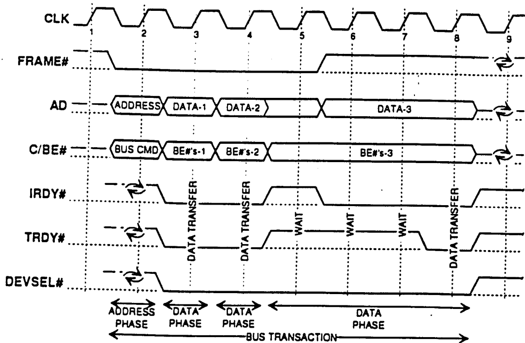
Basic Write Operation
