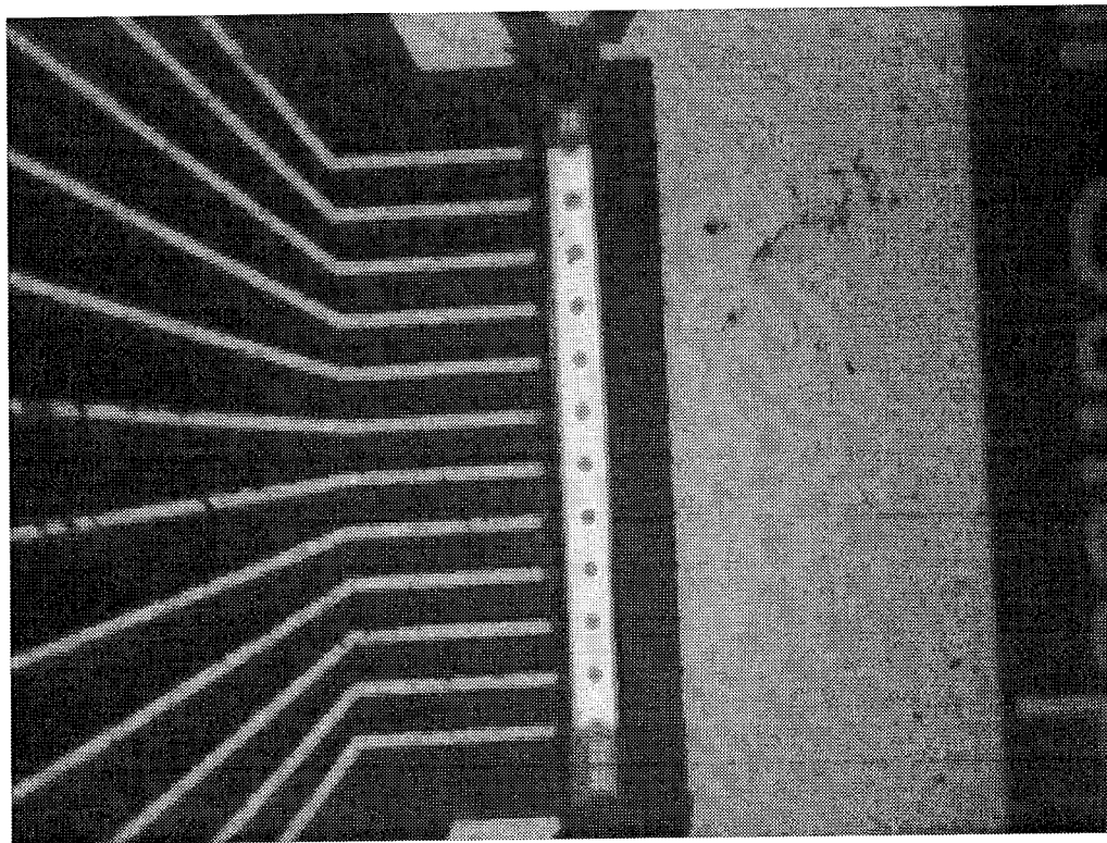
Flip Chip Mounted Bottom Emitting VCSEL Array
