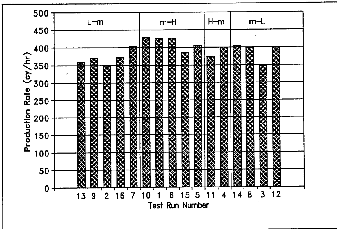
Figure 17. Water level-sorted average production rate, DRP eductor
