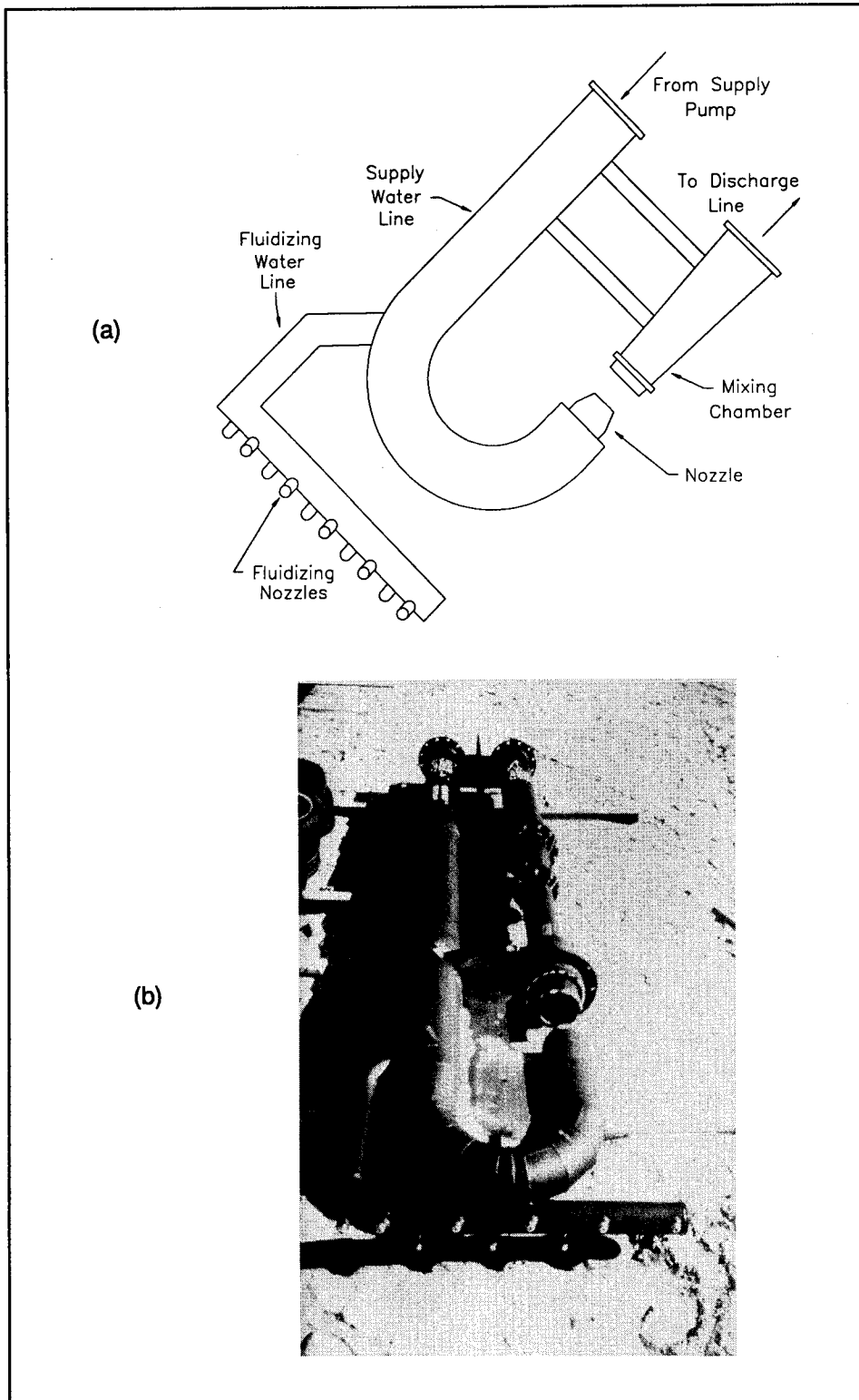
Figure 3. IRI eductor
