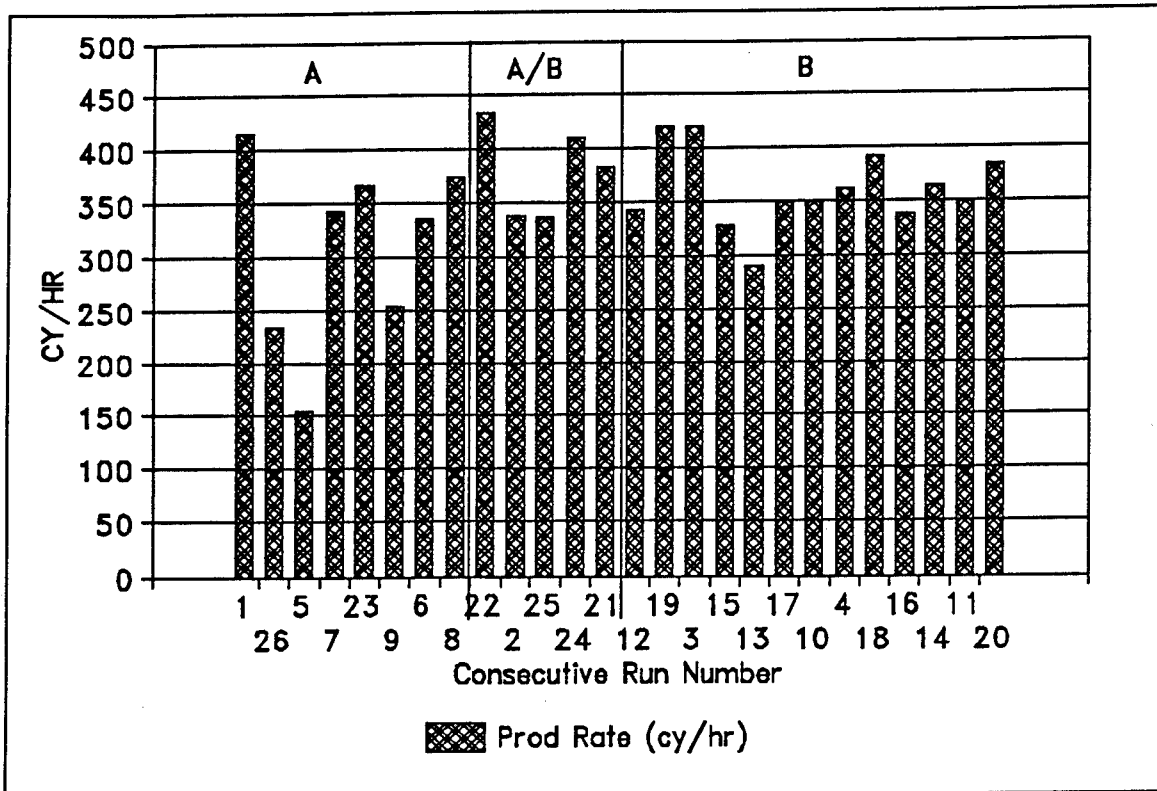
Figure 14. Operator-sorted average daily production rates, IRI eductor
