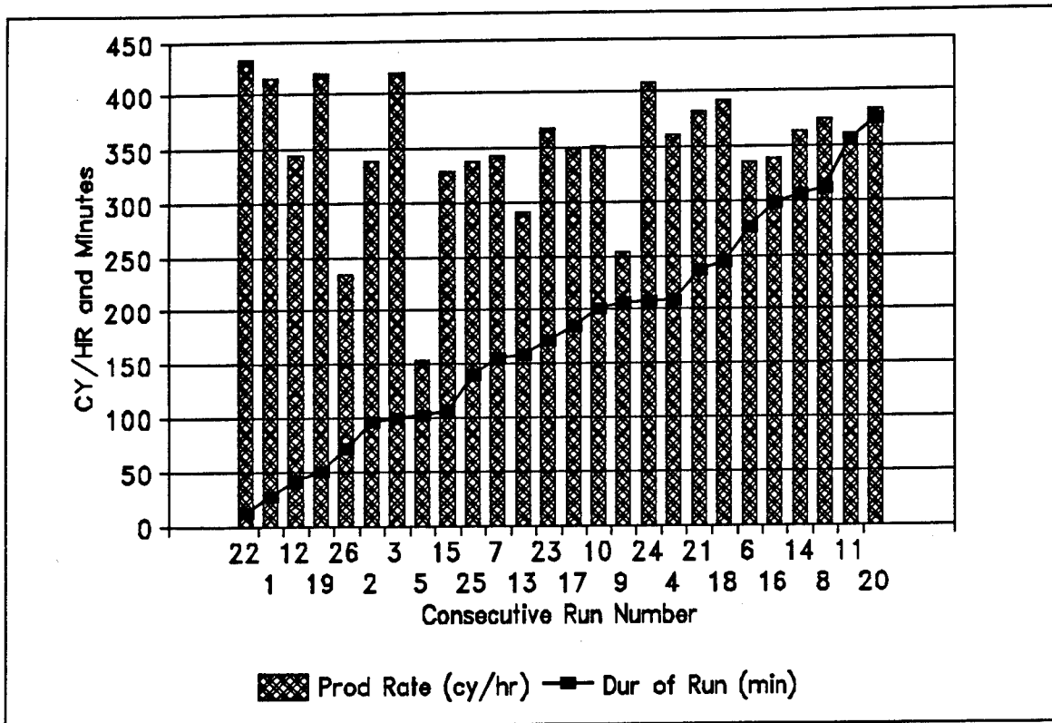
Figure 10. Average daily production rates for IRI eductor (duration sorted)
