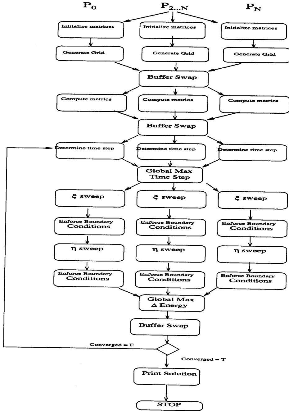
Figure 21. Parallel Flow of Roe Scheme Code.
