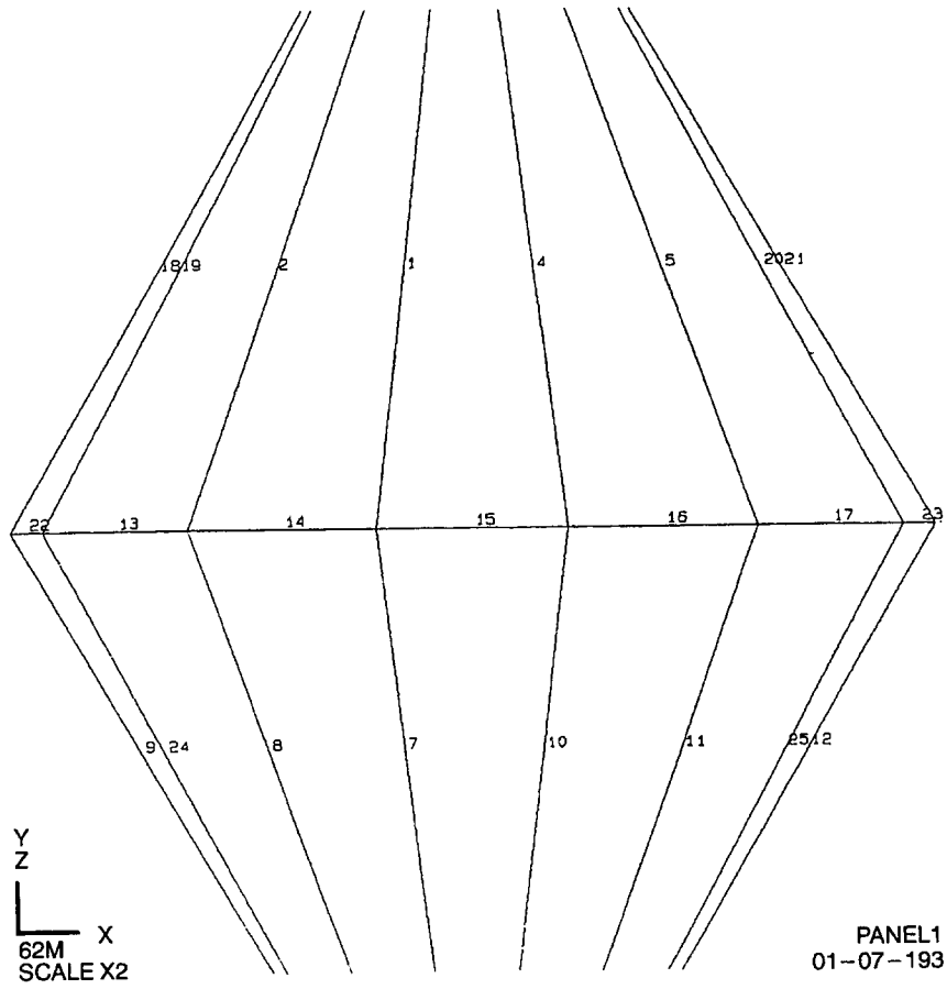
Figure 3. CFG2 panel.
