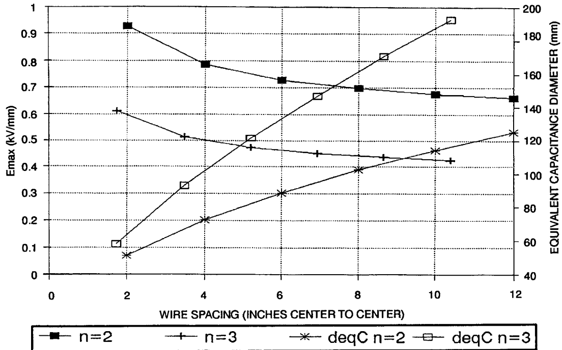
Figure 9. Cutler topload estimated cage gradient 1.01-inch-diameter wires near the catenary.
